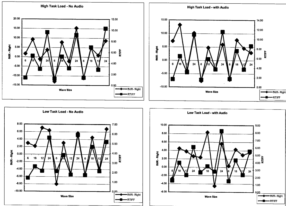
Figure 8. fNIR (Right) measurements vs. RTIFF (n=8). The plot reflects the correlation between rate of change in right prefrontal oxygenation and performance measure RTIFF for each of the 12 waves of the scenario.
