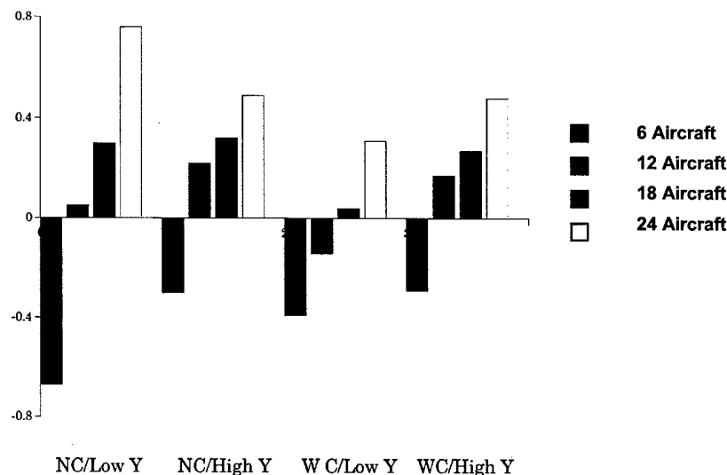
Figure 3: Estimates of executive demand derived from analysis of physiology. NC = SST off, WC = SST on, Low Y = low number of yellows, High Y = high number of yellows
