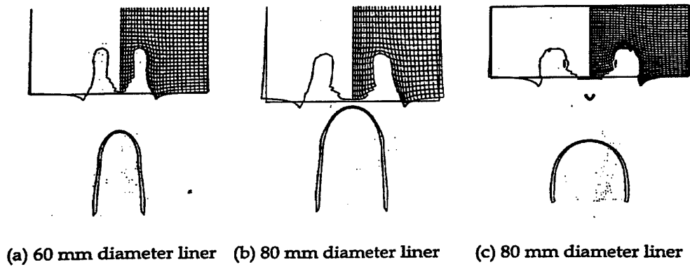
Figure 5 Dyna 2D outputs for the penetration into mild steel of three different designs of EFP's. The liner diameters are as indicated with variation in the charge diameter and the geometry of the liner contour radii giving rise to the different penetration profiles.
