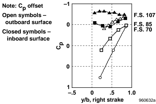
(c) \delta_{s,LR} = 0^\circ/60^\circ , M = 0.26 , Re_c = 9.3 \times 10^6 .
