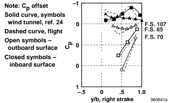
Figure 15. Comparison of flight and wind tunnel pressure distributions, \alpha = 50^\circ , \delta_{s,LR} = 0^\circ/90^\circ , M = 0.24 , Re_c = 9.4 \times 10^6 .
