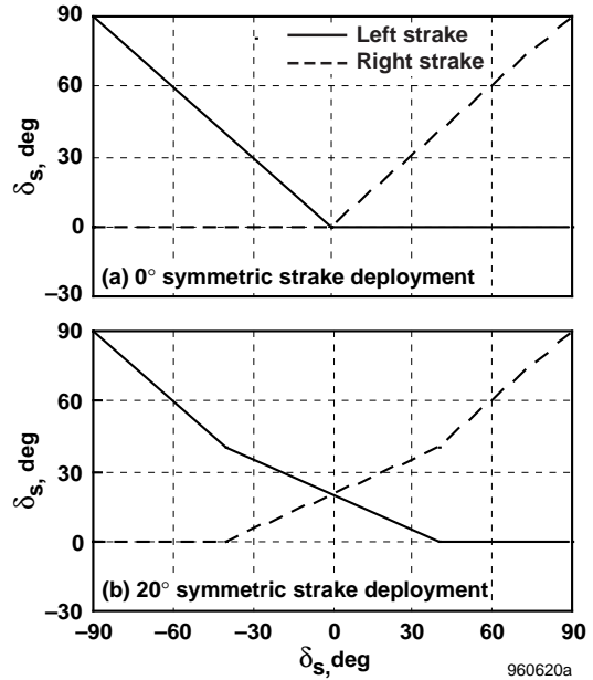
Figure 7. Symmetric strake deployment schedule.
