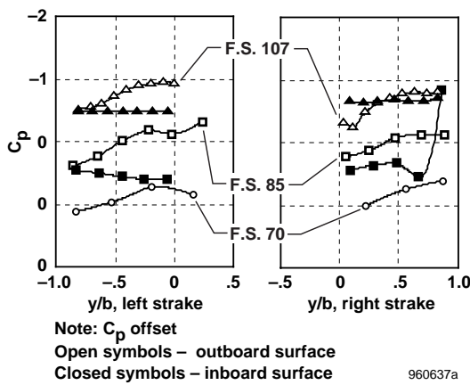
Figure 13. Forebody and strake pressure distributions with the ANSER radome at \alpha = 50^\circ for the 20^\circ symmetric strake deployment, pilot's view, \delta_{s,LR} = 10^\circ/30^\circ , M = 0.28 , Re_c = 10.2 \times 10^6 .
