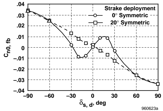
Figure 8. F-18 HARV forebody yawing moments as a function of differential strake position, \beta = 0^\circ .
