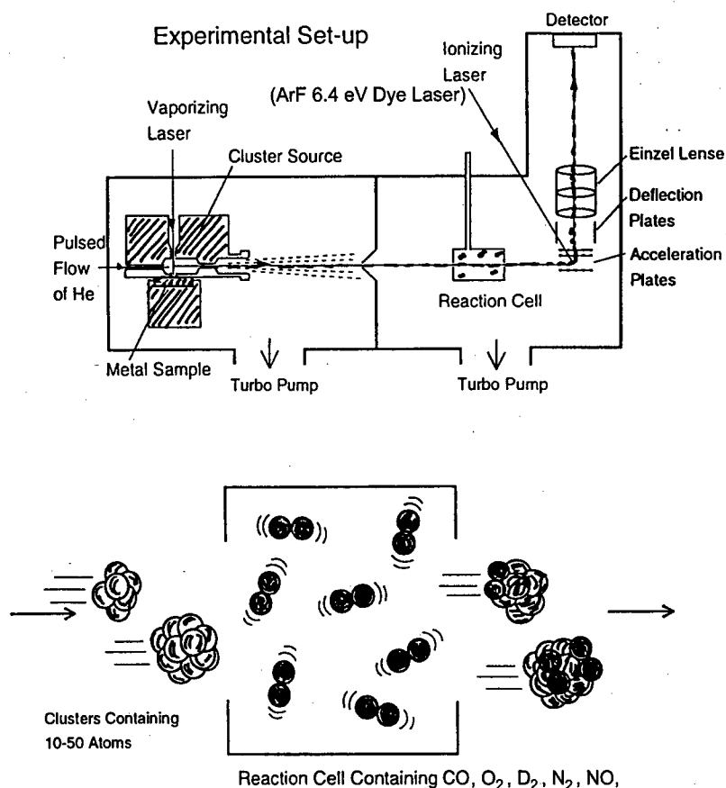
Figure 4.1. Schematic drawing of the experimental setup used in Göteborg for studies of chemical reactivity and/or sticking probability of various molecules with the clusters. The production of clusters is via laser vaporization of metal substrates and detection via photo-ionization time-of-flight mass spectrometry (A. Rosen, University of Göteborg, Sweden).
