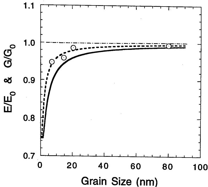
Figure 6.1. Ratio of the Young's ( E ) and shear ( G ) moduli of nanocrystalline materials to those of conventional grain size materials as a function of grain size. The dashed and solid curves correspond to a grain boundary thickness of 0.5 and 1 nm, respectively (Shen et al. 1995).
