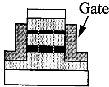
Figure 5.7. Gated double barrier tunnel diode structure (Max-Planck-Institut, Stuttgart; NTT; Purdue University).
