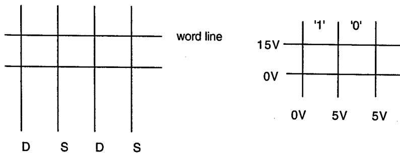
Figure D.6. Polysilicon transistors.
