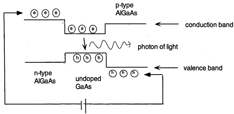
Figure 5.16. Schematic of a semiconductor laser.
