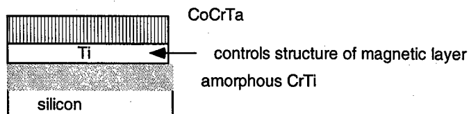
Figure D.4. Perpendicular recording using CoCrTa (Hitachi).
