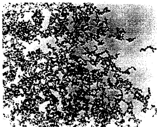
Figure B.2. Electron micrograph of antimony-doped tin dioxide particles (primary particle size \sim 20 nm).
