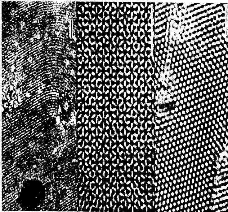
Figure 2.3. TEM images of (a) the lamellar morphology, (b) the cubic phase with Ia3d symmetry viewed along its [111] zone axis, and (c) the hexagonal phase viewed along its [001] zone axis of the silica/surfactant nanostructured composites by co-assembly (McGehee et al. 1994) (bars = 30 nm).
