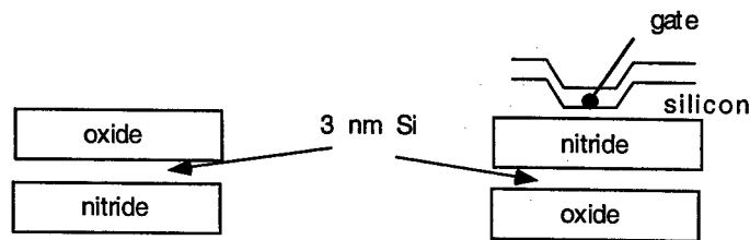
Figure D.6. Polysilicon transistors.
