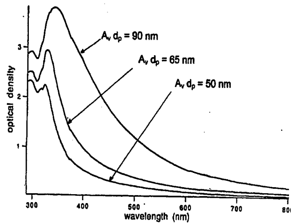
Figure 3.1. Transparency as a function of particle size (Nanophase).
