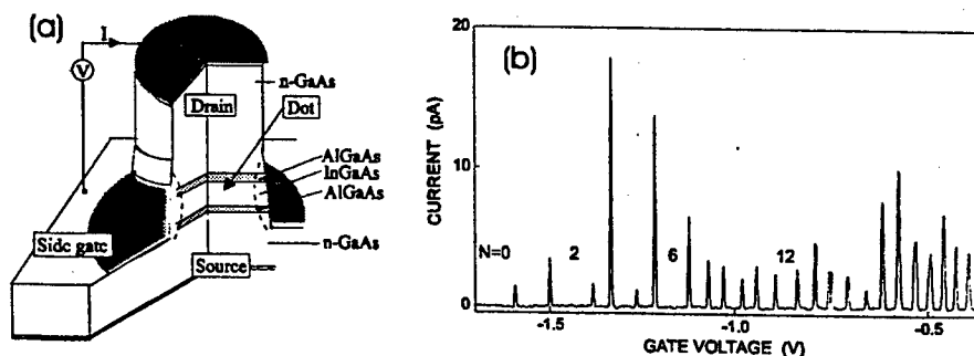
Figure B.6. (a) Schematic diagram of the gated quantum dot device and (b) the Coulomb oscillations in the current vs. gate voltage at B = 0T observed for a 0.5 \mu\text{m} diameter dot.
