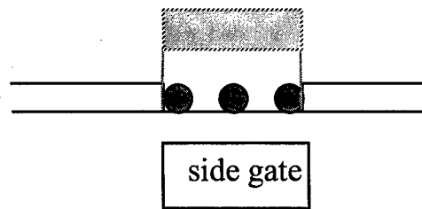
Figure 5.2. Metal colloids, self-assembled monolayer (SAM) coatings, polysilicon, quantum dots embedded in SiO 2 (Hitachi, IBM, RIKEN, NTT, ETL, University of Lund).
