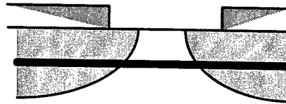
Figure 5.8. Depletion layer control of 2DEG area (Hitachi, University of Glasgow, University of Tokyo).
