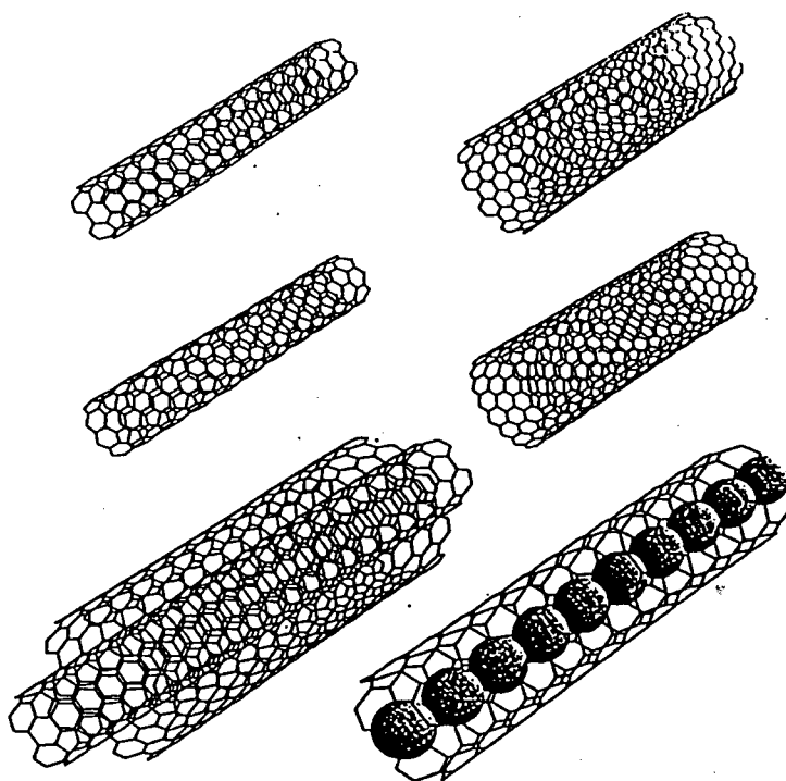
Figure 4.6. Examples of carbon nanotube structures, including multiwalled and metal-atom-filled nanotubes.
