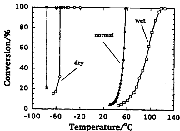
Figure 4.2. Effect of moisture on conversion profiles for CO oxidation over \text{Co}_3\text{O}_4 and \text{Au}/\text{Co}_3\text{O}_4 .
