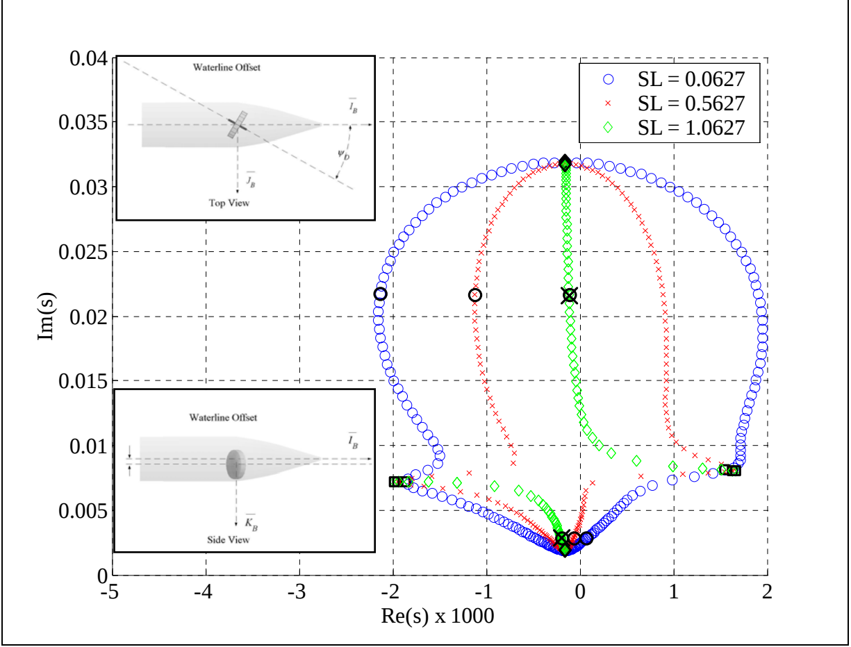
Figure 10. Root-locus for a disk located 3/4 in off-axis of symmetry in the waterline direction (spin ratio = 10, mass ratio = 1/10) ( \diamond = 0^\circ, 360^\circ disk angle; \circ = 90^\circ disk angle; \square = 180^\circ disk angle; \times = rigid projectile).
