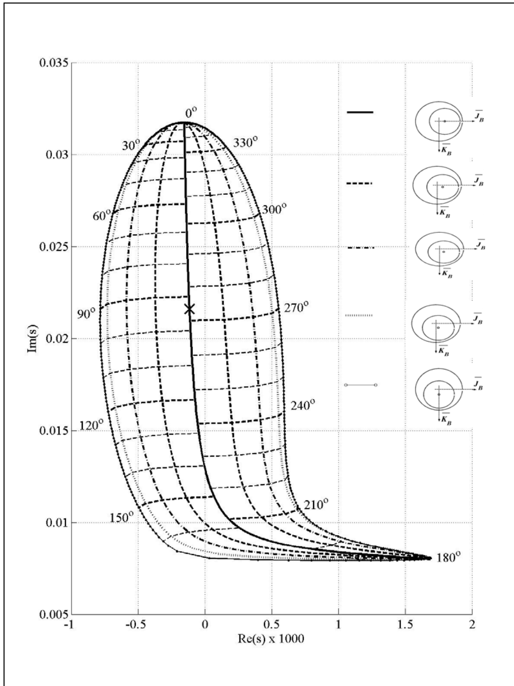
Figure 11. Fast mode root-locus for a disk located 1/4 in off-axis of symmetry in the waterline and buttline directions (spin ratio = 10; mass ratio = 1/10).
