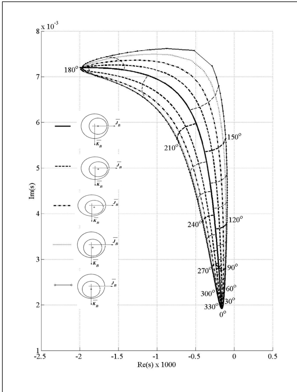
Figure 12. Slow mode root-locus for a disk located 1/4 in off-axis of symmetry in the waterline and buttline directions (spin ratio = 10; mass ratio = 1/10).
