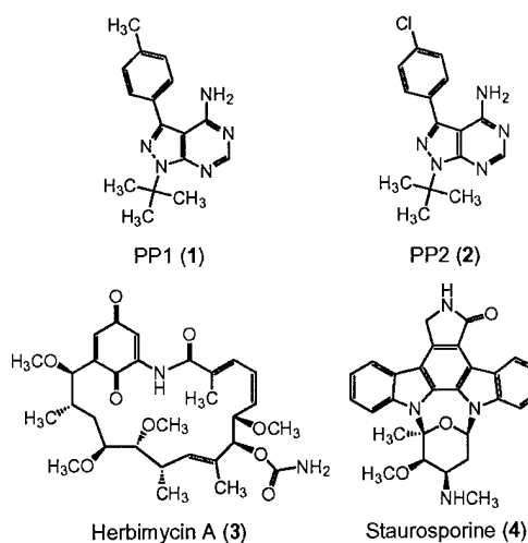
Scheme 1. Structures of protein tyrosine kinase inhibitors that engage the ATP binding site.
