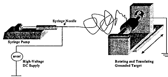
Figure 1. Schematic of the electrospinning system
