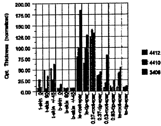
Figure 7: Conventional Wing - Four Spars
