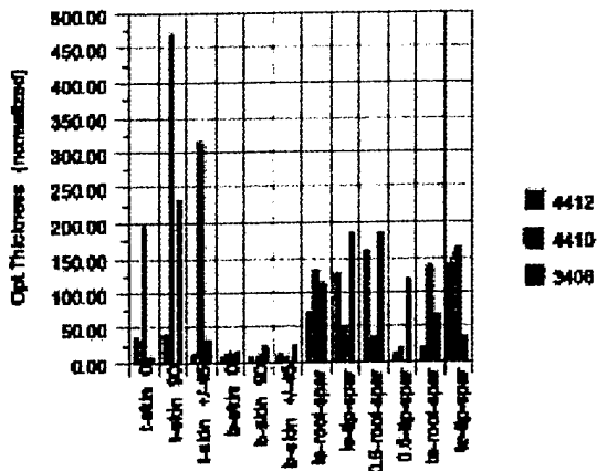
Figure 8: Lambda Wing - Three Spars
