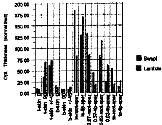
Figure 11: NACA 3408 - Four Spars
