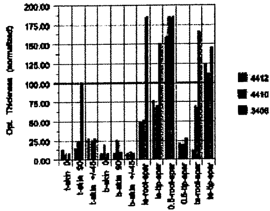
Figure 6: Conventional Wing - Three Spars
