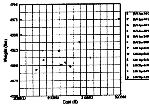
Figure 12: Weight vs. Cost - Exploded View
