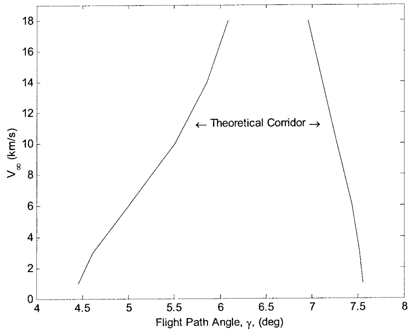
Figure 4.4: Theoretical Corridor, L/D = 0.75
