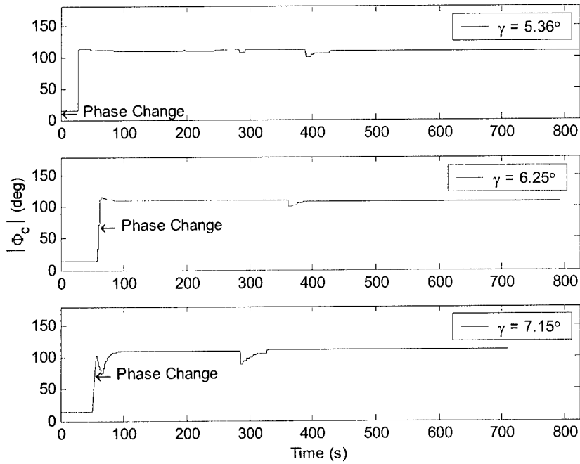
Figure 5.12: Commanded Bank Angle vs. Time, V_\infty = 6 km/s, L/D = 0.75
