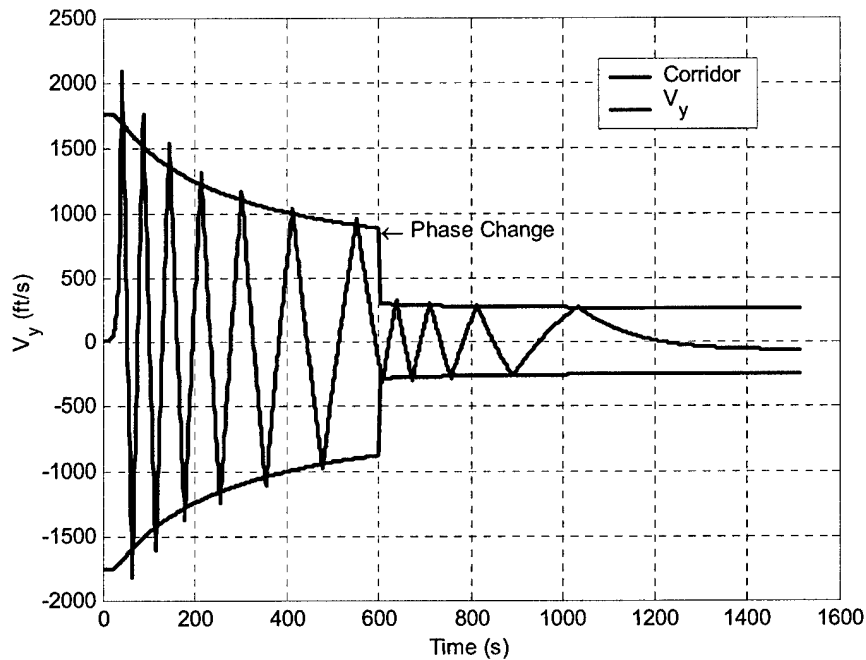
Figure 5.46: Out of Plane Velocity vs. Time, V_\infty = 14 \text{ km/s} , L/D = 1.5 , \gamma = 6.9^\circ
