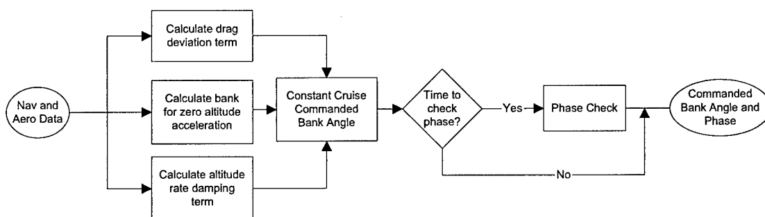
Figure 3.2: Energy Management Phase
