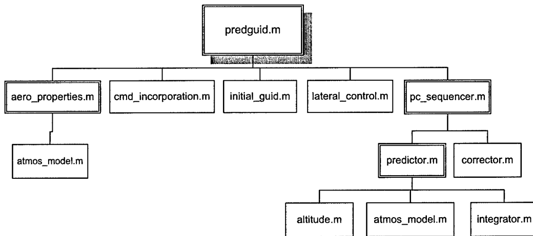
Figure A.2: Aerocapture Guidance Functional Flow: pred_guid.m
