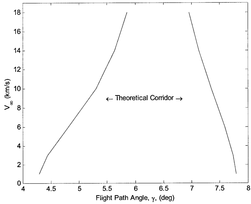
Figure 4.6: Theoretical Corridor, L/D = 1.25
