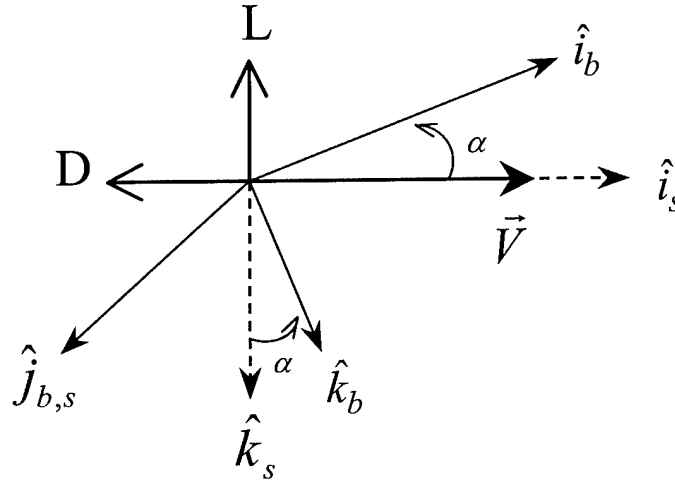
Figure 2.2: Angle of Attack Rotation
