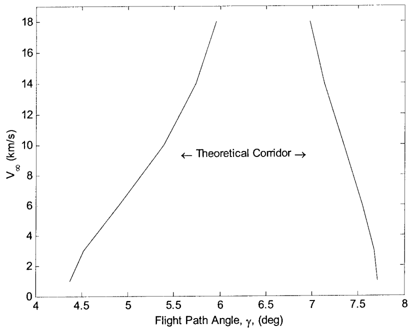
Figure 4.5: Theoretical Corridor, L/D = 1.00
