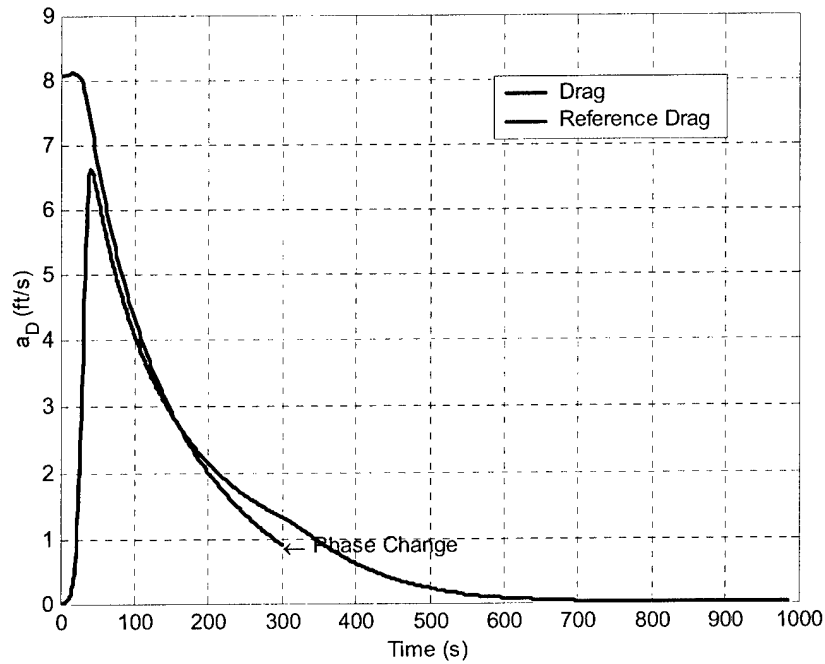
Figure 5.5: Drag Acceleration vs. Time, V_\infty = 14 \text{ km/s} , L/D = 0.75 , \gamma = 6.9^\circ
