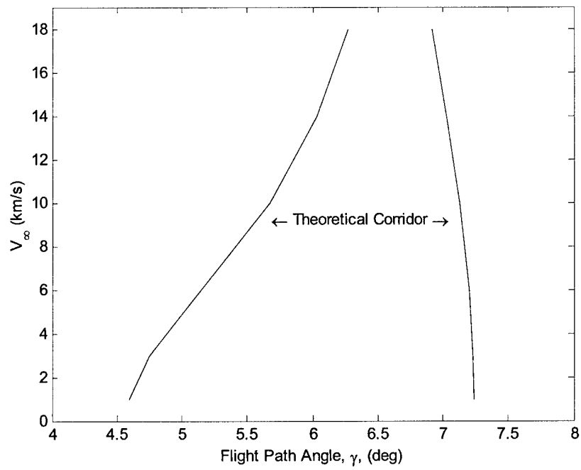
Figure 4.3: Theoretical Corridor, L/D = 0.50
