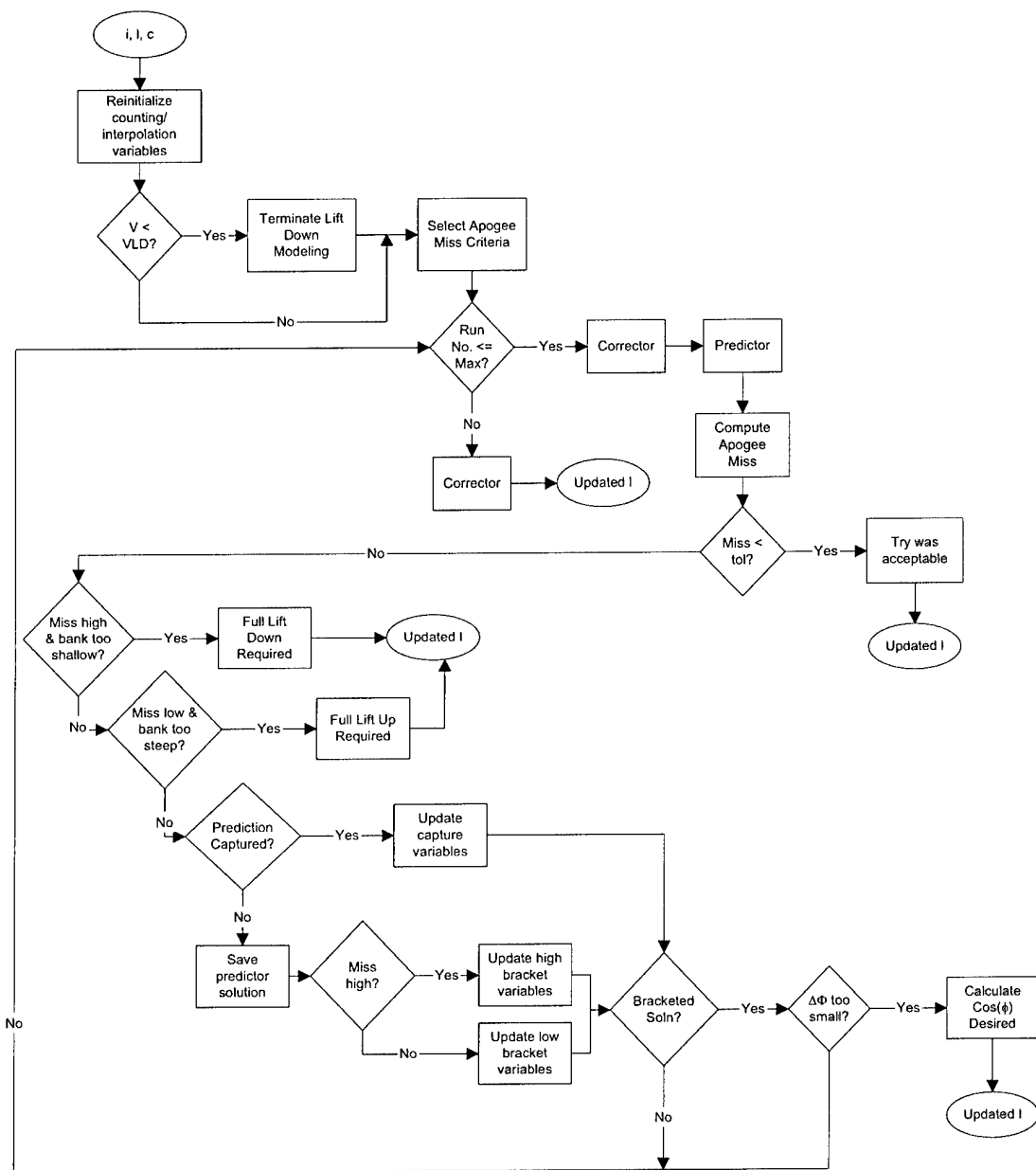
Figure A.5: Predictor-Corrector Sequencer Logical Flow: pc_sequencer.m
