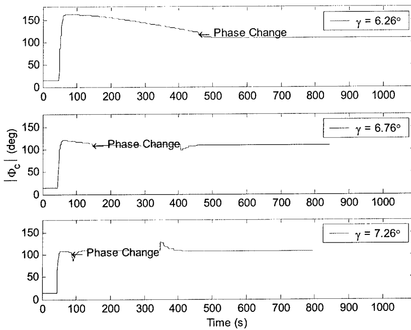
Figure 5.13: Commanded Bank Angle vs. Time, V_\infty = 10 km/s, L/D = 0.75
