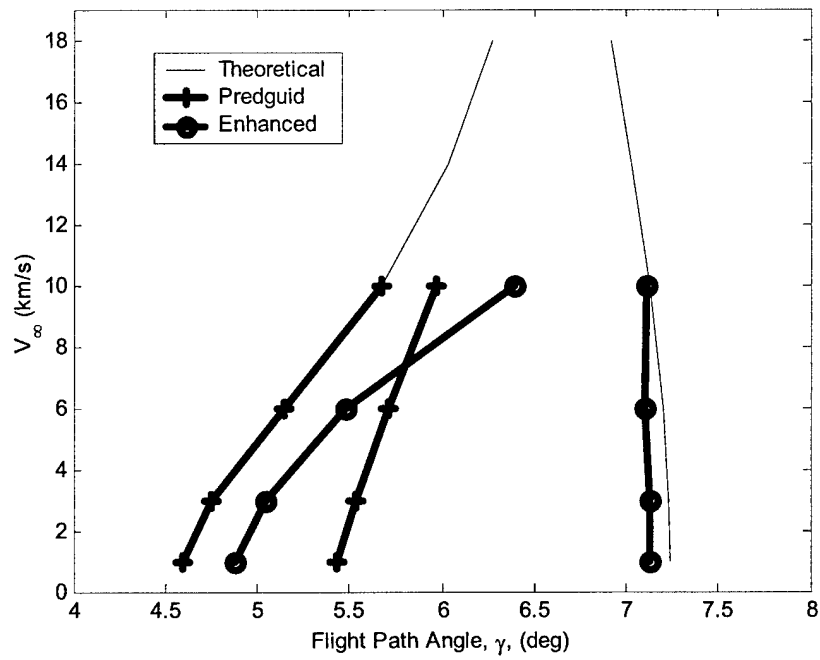
Figure 5.21: Theoretical and Capturable Corridors, L/D = 0.50
