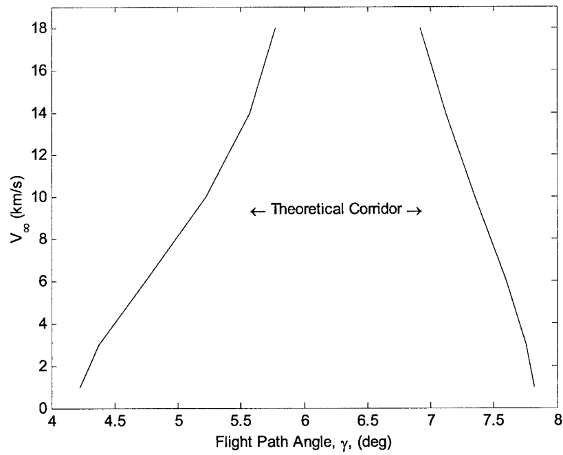
Figure 4.7: Theoretical Corridor, L/D = 1.50
