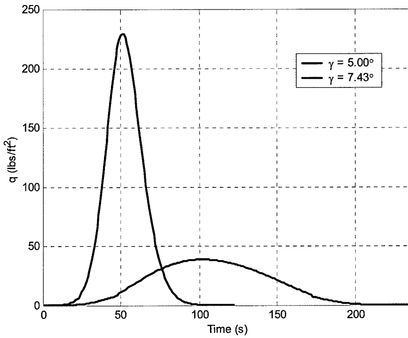
Figure 4.9: Dynamic Pressure vs. Time, Corridor Extremes
