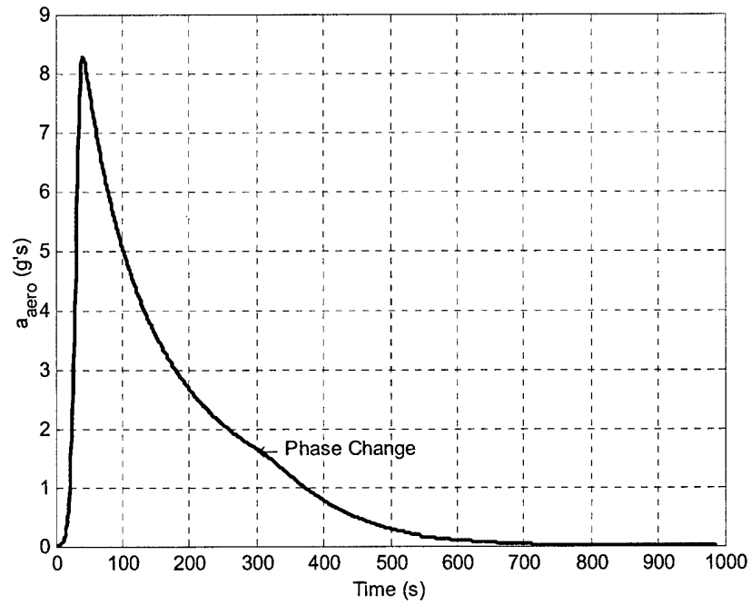
Figure 5.3: Acceleration vs. Time, V_{\infty} = 14 km/s, L/D = 0.75 , \gamma = 6.9^{\circ}
