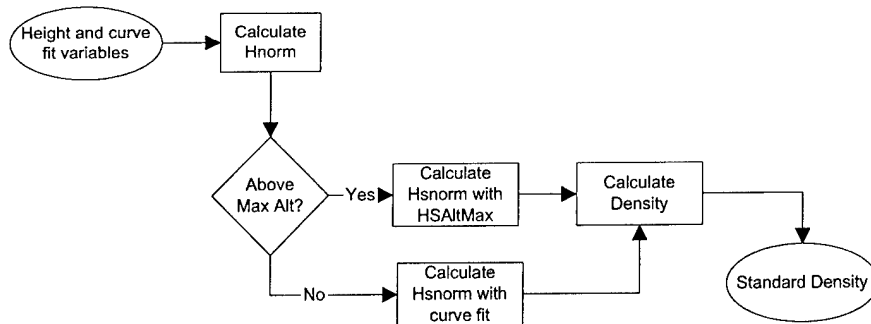
Figure A.11: Atmospheric Model Logical Flow: atmos_model.m
