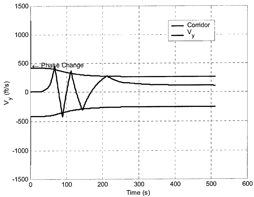
Figure 5.47: Out of Plane Velocity vs. Time, V_\infty = 6 \text{ km/s} , L/D = 0.25 , \gamma = 6.0^\circ
