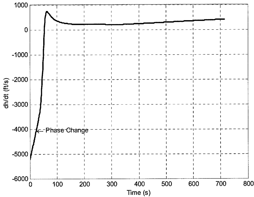
Figure 5.40: Altitude Rate vs. Time, V_{\infty} = 6 \text{ km/s} , L/D = 0.75 , \gamma = 7.25^{\circ}
