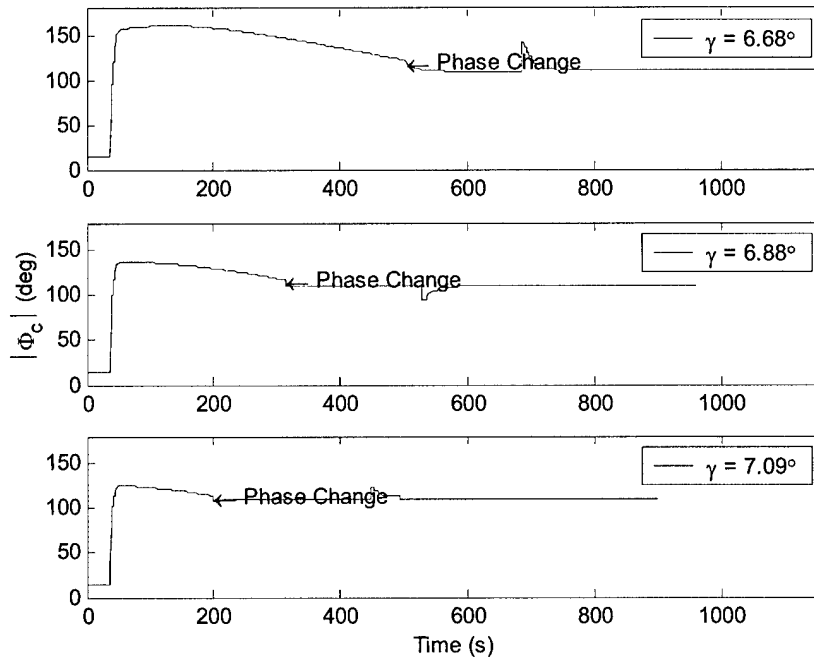
Figure 5.14: Commanded Bank Angle vs. Time, V_\infty = 14 km/s, L/D = 0.75
