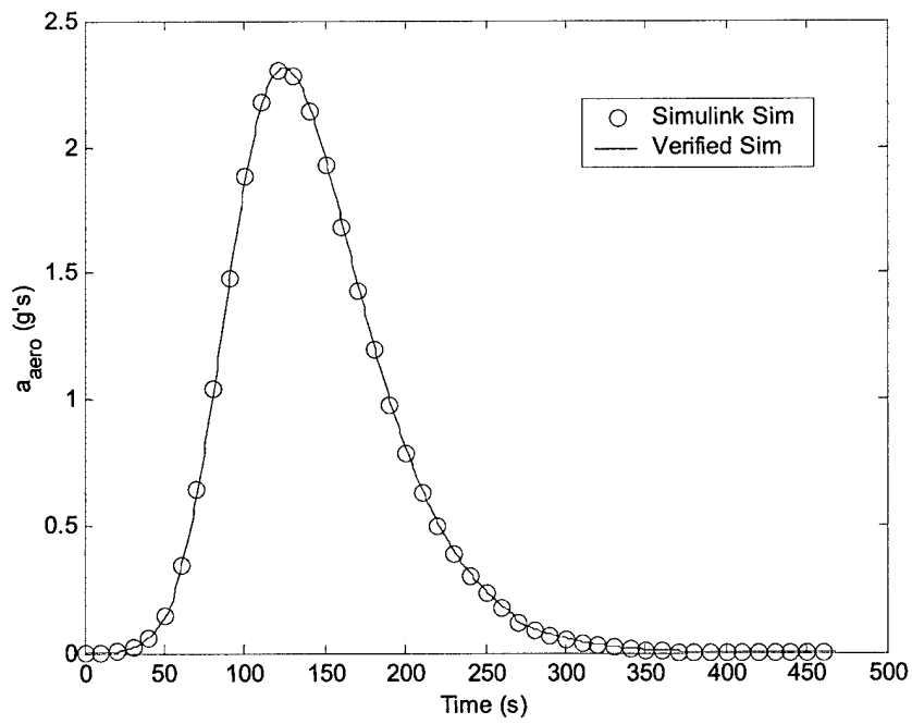
Figure B.9: Vehicle Acceleration vs. Time
