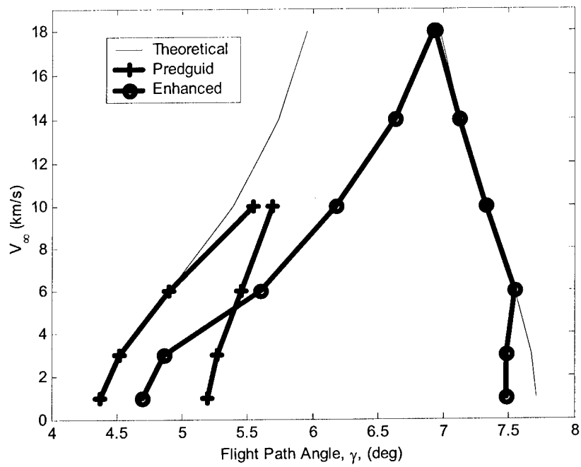
Figure 5.23: Theoretical and Capturable Corridors, L/D = 1.00
