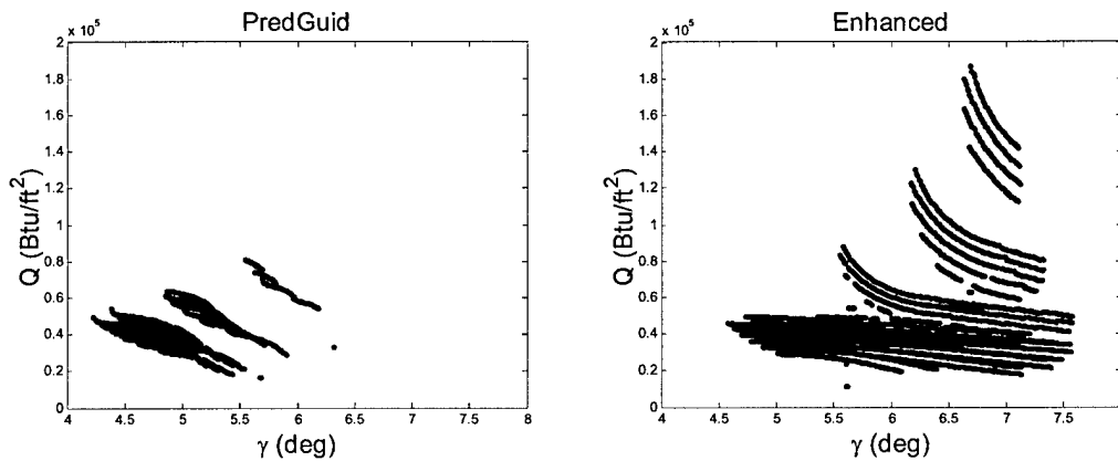
Figure 5.43: Heating Load vs. Flight Path Angle
