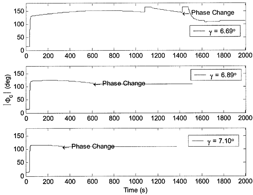
Figure 5.19: Commanded Bank Angle vs. Time, V_\infty = 14 km/s, L/D = 1.5
