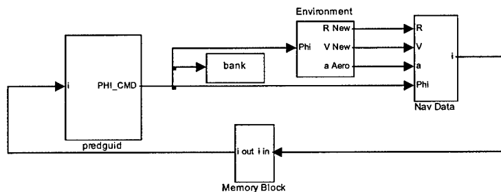
Figure B.20: Closed Loop Guidance Verification Setup
