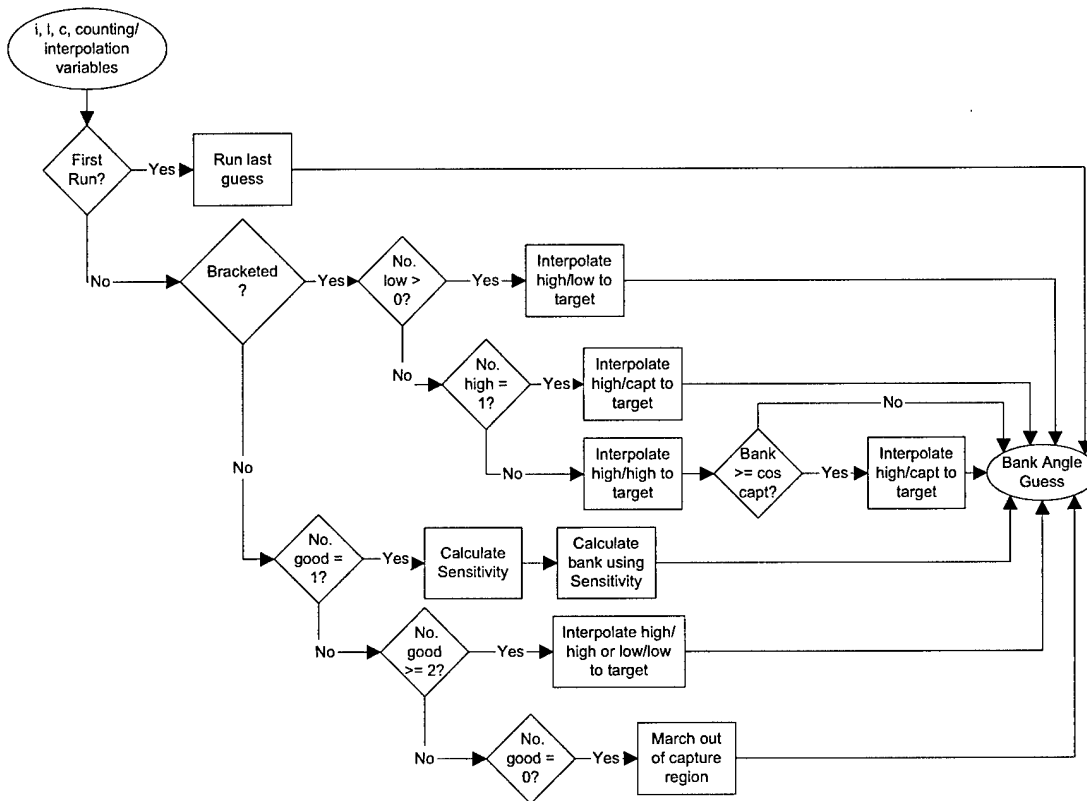
Figure A.6: Corrector Logical Flow: corrector.m
