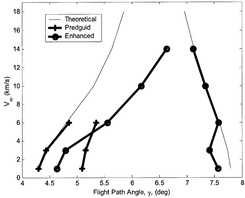
Figure 5.24: Theoretical and Capturable Corridors, L/D = 1.25
