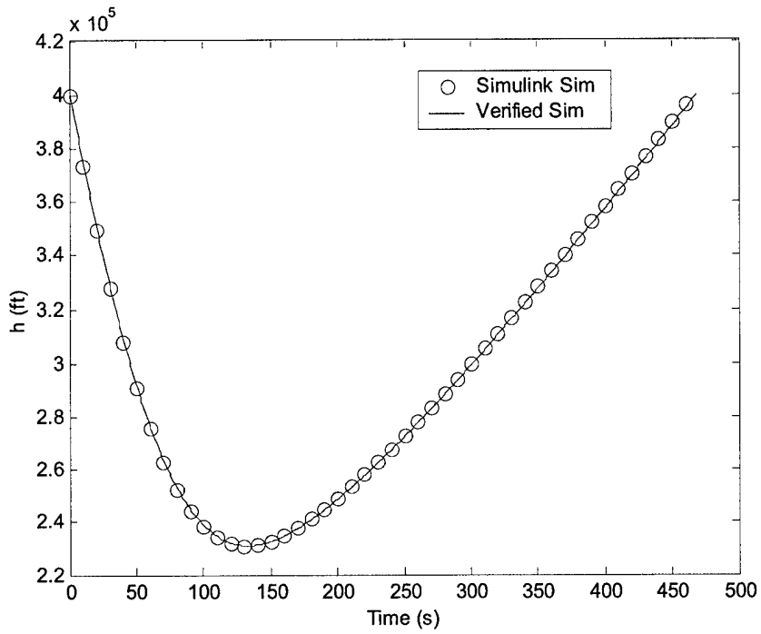
Figure B.8: Vehicle Altitude vs. Time
