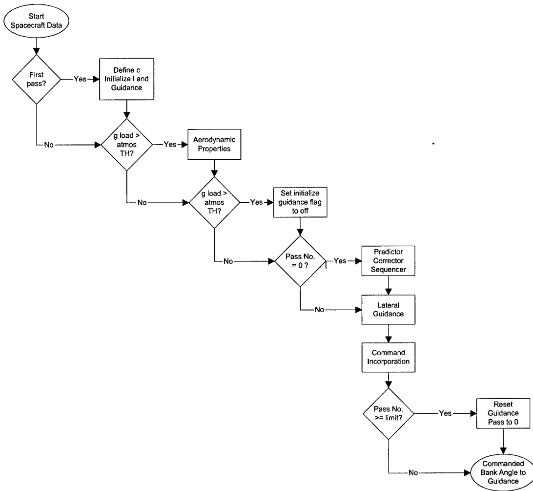
Figure A.1: Aerocapture Guidance Logical Flow: pred_guid.m
