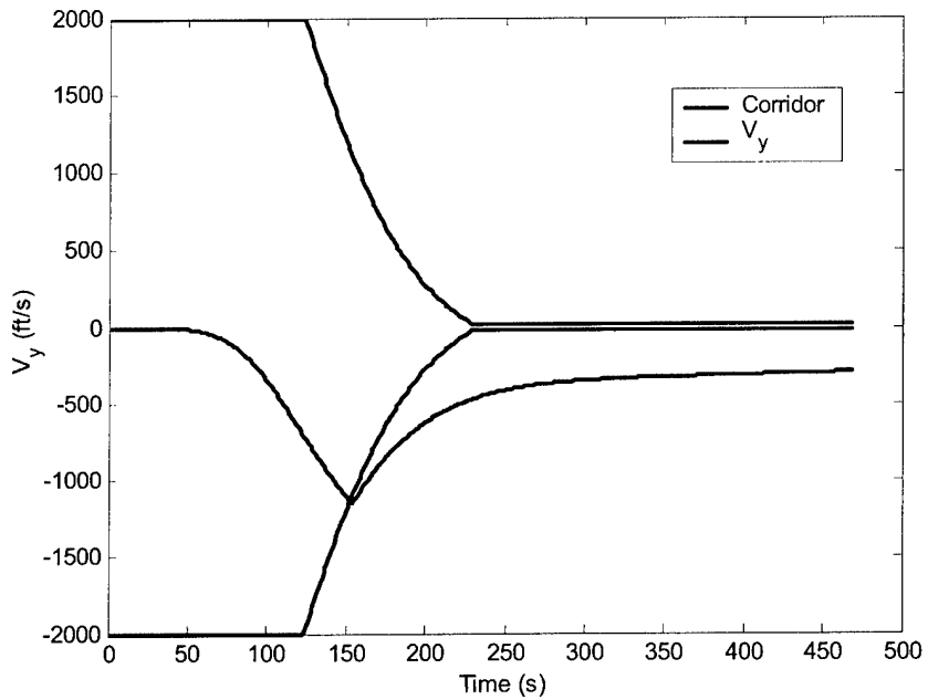
Figure B.24: Lateral Corridor and Out of Plane Velocity, Corrected
