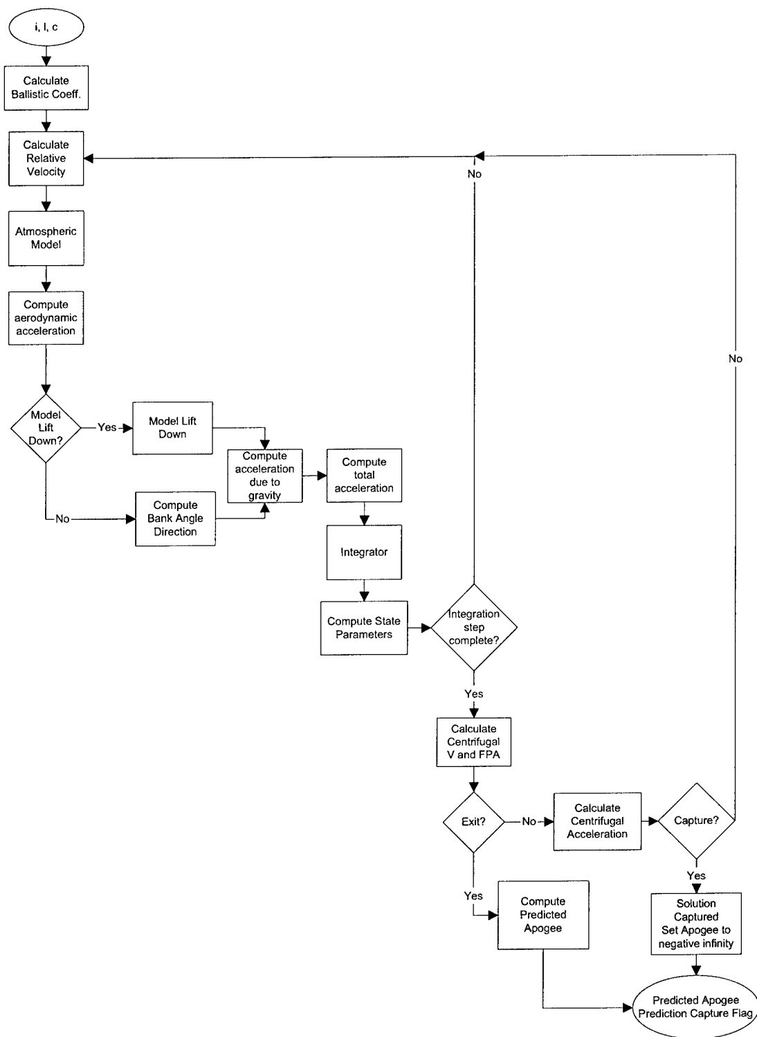
Figure A.7: Predictor Logical Flow: predictor.m
