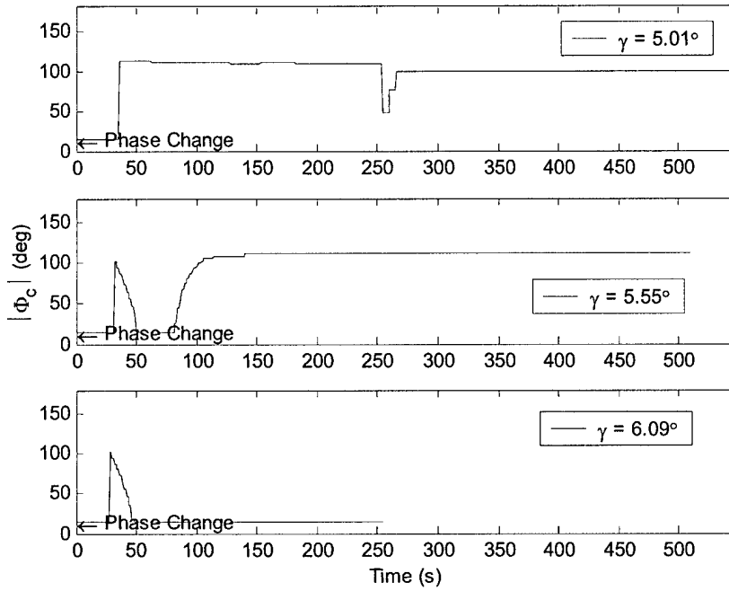
Figure 5.6: Commanded Bank Angle vs. Time, V_\infty = 1 km/s, L/D = 0.25
