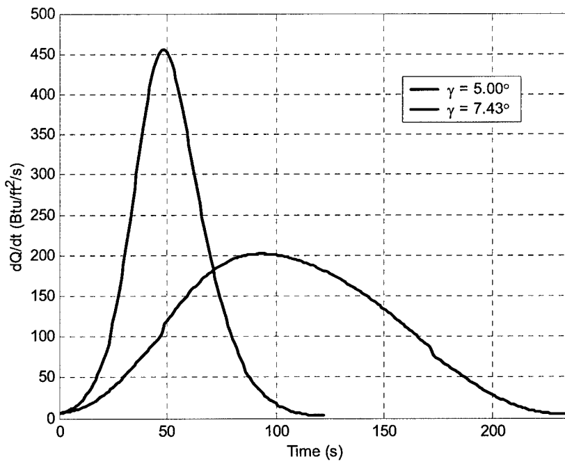
Figure 4.10: Heating Rate vs. Time, Corridor Extremes
