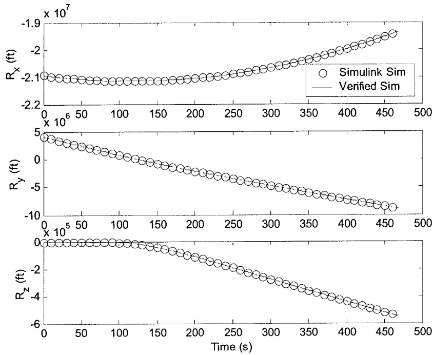
Figure B.2: Vehicle Position vs. Time
