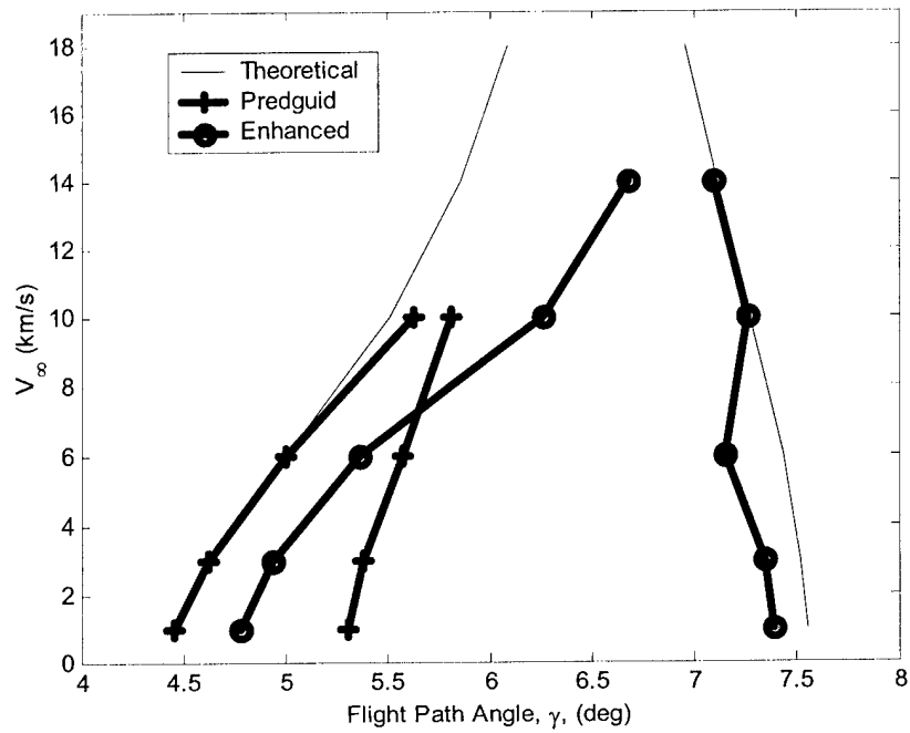
Figure 5.22: Theoretical and Capturable Corridors, L/D = 0.75
