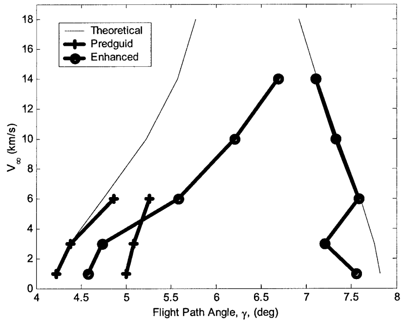
Figure 5.25: Theoretical and Capturable Corridors, L/D = 1.50
