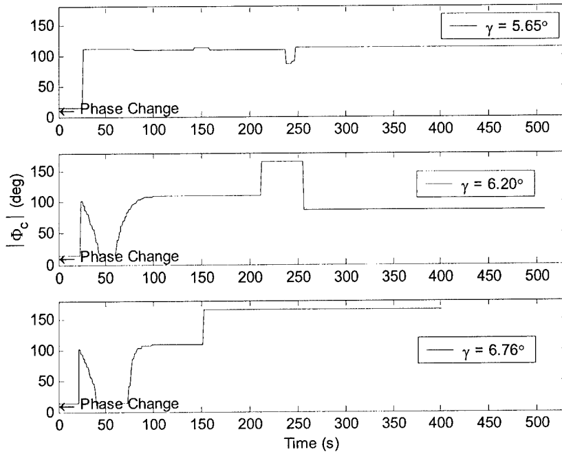
Figure 5.8: Commanded Bank Angle vs. Time, V_\infty = 6 km/s, L/D = 0.25
