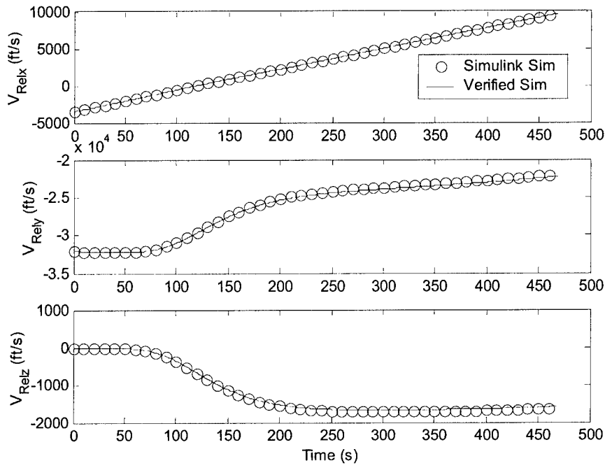
Figure B.13: Vehicle Relative Velocity Components vs. Time, J2 Effects
