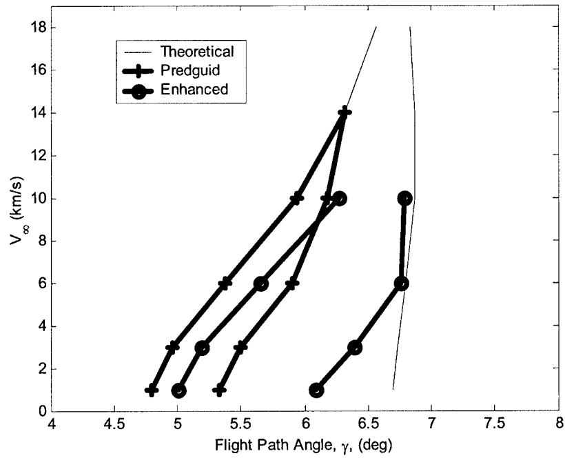
Figure 5.20: Theoretical and Capturable Corridors, L/D = 0.25
