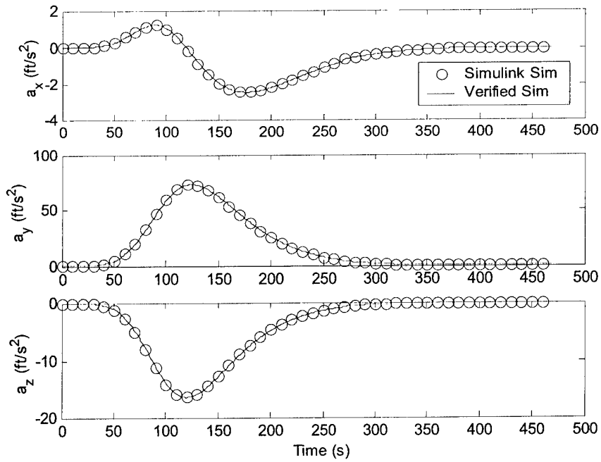
Figure B.7: Vehicle Acceleration Components vs. Time
