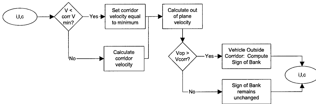
Figure A.9: Lateral Guidance Logical Flow: lateral_control.m
