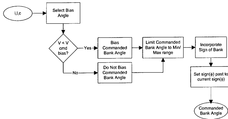
Figure A.10: Command Incorporation Logical Flow: cmd_incorporation.m
