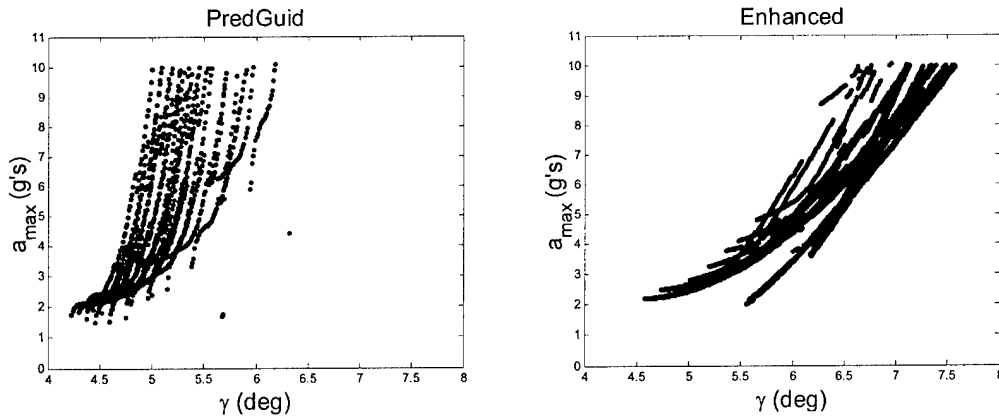
Figure 5.41: Maximum Acceleration vs. Flight Path Angle
