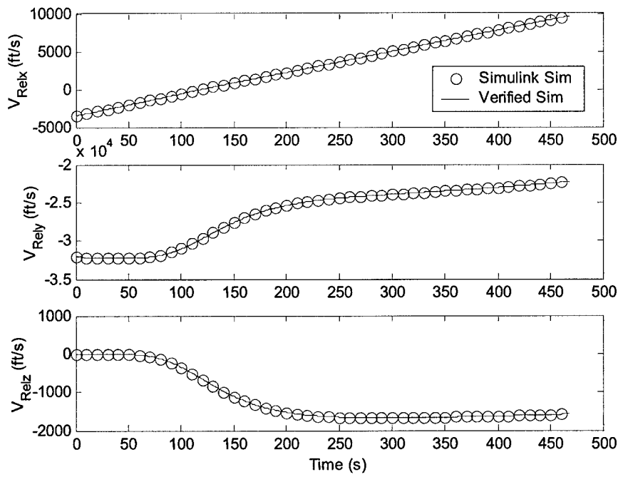
Figure B.5: Vehicle Relative Velocity Components vs. Time
