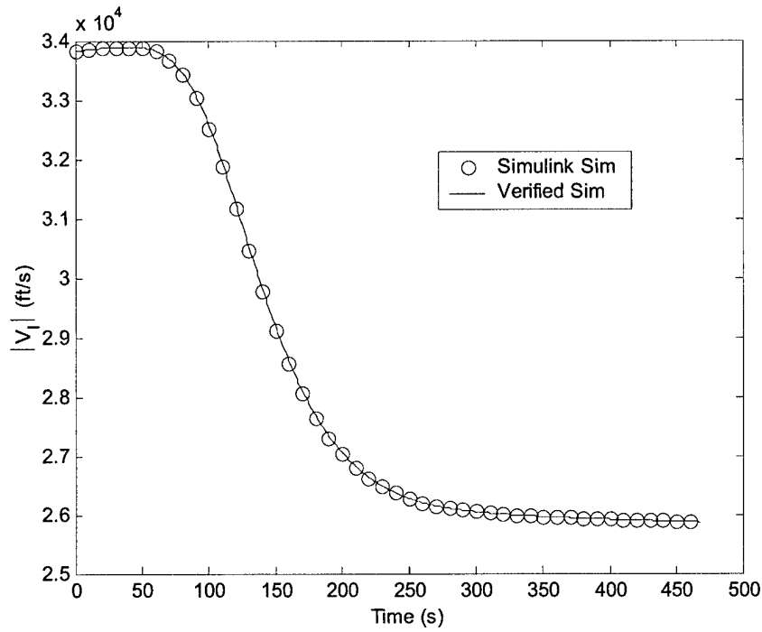
Figure B.4: Vehicle Velocity Magnitude vs. Time
