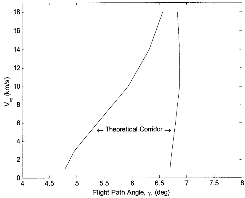
Figure 4.2: Theoretical Corridor, L/D = 0.25
