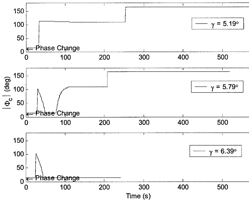
Figure 5.7: Commanded Bank Angle vs. Time, V_\infty = 3 km/s, L/D = 0.25
