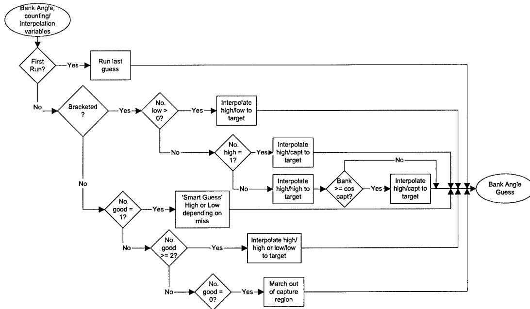
Figure 3.5: Corrector Functional Flow
