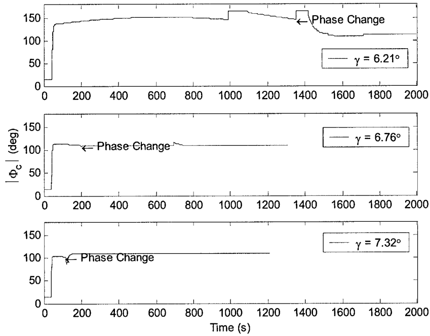
Figure 5.18: Commanded Bank Angle vs. Time, V_\infty = 10 km/s, L/D = 1.5
