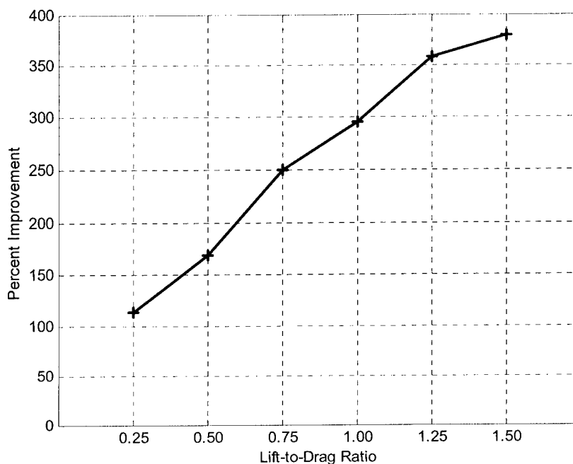
Figure 5.26: Percent Improvement of Corridor Captured
