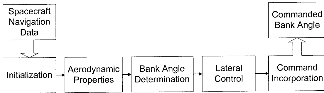
Figure 3.1: Guidance Algorithm Flow
