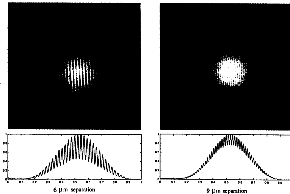
Fig. 2. Measured two-pinhole interference patterns for horizontal pinhole separations of 6 and 9\text{ }\mu\text{m} , for a wavelength of 13.4\text{ nm} and a beamline acceptance half-angle of 48\text{ }\mu\text{rad} . The pinhole diffraction patterns overlap and produce an interference pattern within the Airy envelope. The interference patterns are recorded on an EUV sensitive CCD camera, located 26\text{ cm} downstream of the pinhole mask. Pinhole diameters range from 400 to 500\text{ nm} , but are equal in their respective pairs. As shown in the lineouts, fringe visibility of the modulation decreases for larger separations ( 0.4 for 6\text{ }\mu\text{m} and 0.14 for 9\text{ }\mu\text{m} ), indicating reduced spatial coherence. Spectral resolution for these measurements is 55 .
