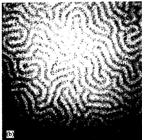
Fig. 2. Images of magnetization within an iron gadolinium multilayer, imaged at the iron L_{III} (a) and L_{II} (b) edges (707.5 and 720.5 eV, respectively). The expected contrast reversal of X-MCD between the edges can be seen.
