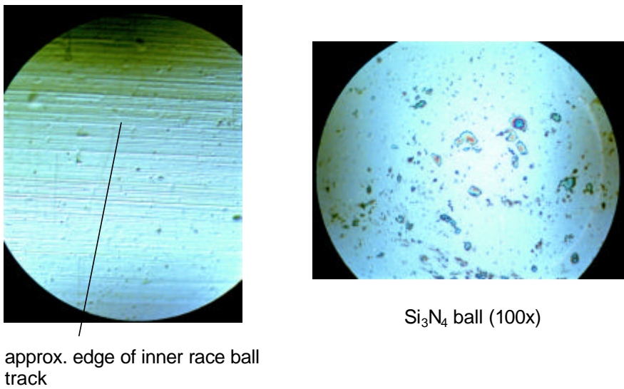
Figure 14. Micrographs of the Bearing Surface of a Bearing Tested with a Cotton-Phenolic Cage
