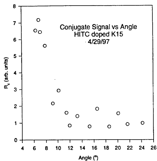
Figure 7 Phase conjugate signal R_c vs. probe-pump crossing angle, \alpha , for DFWM in a 100 \mu\text{m} dye-doped LC film. R_c increases as the \alpha decreases, so that small crossing angles can be used (minimizing beam-walk off effects).
