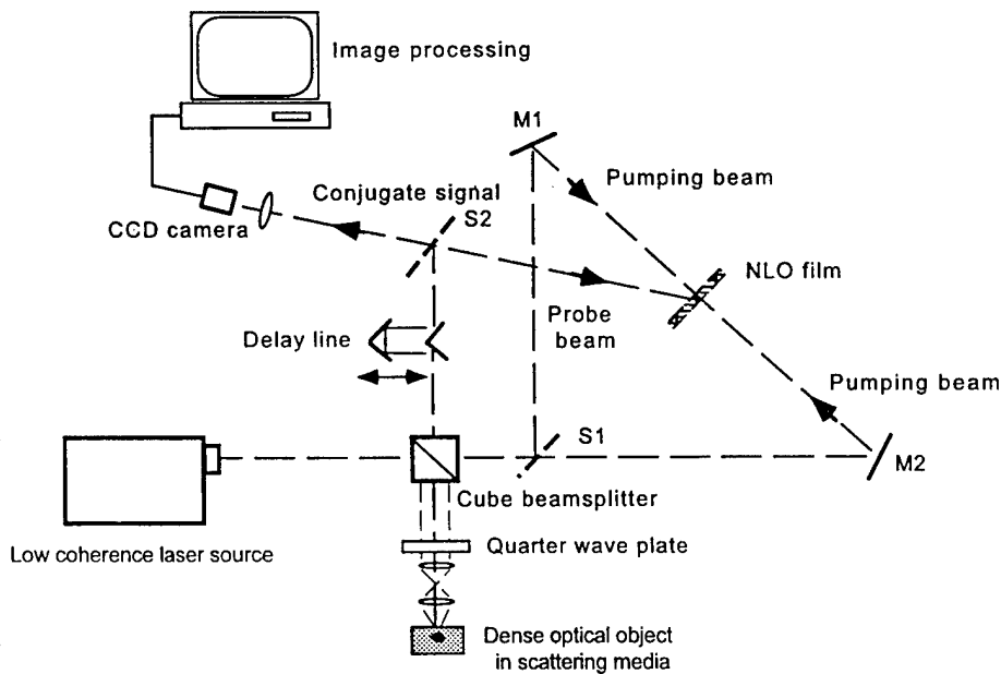
Figure 8 Instantaneous 2-D Imaging Optical Set-Up
