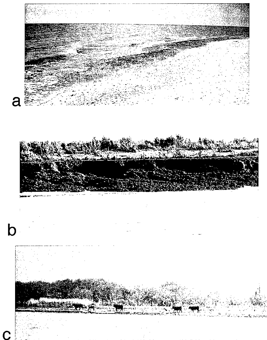
Figure 2-17. Examples of coastal morphology that typify erosional environments on the chenier plain. a: Peat terrace exposed in the swash zone at Site CSB. The old marsh surface is covered by a thin veneer of carbonate sand that forms a beach. b: Peat terrace ~1 m high, forming a scarp along the central chenier plain near Site CSC. A thin carbonate sand beach (~5 m wide and <0.1 m thick) is perched on top of the peat. Backshore marsh vegetation is visible behind the beach. c: Coastal morphology near Tigre Point indicates pronounced erosion, with oak trees standing only ~20 m from the present shoreline. Peat terrace is exposed at the shoreline with minor carbonate sand above it; cattle for scale.
