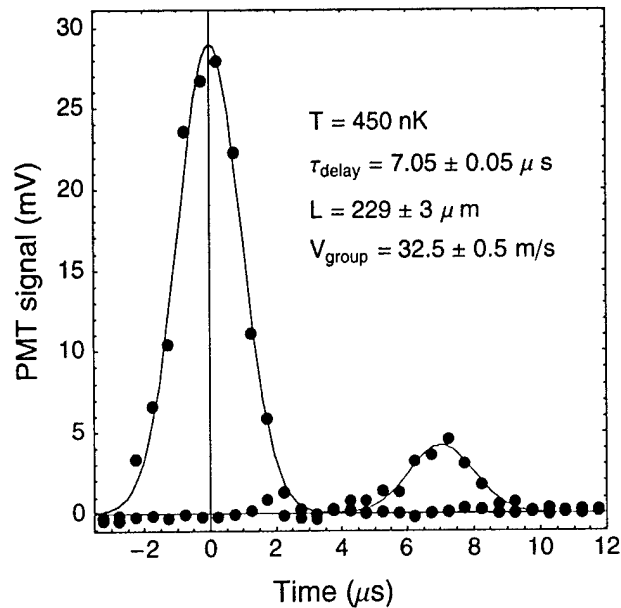
Fig. 2. An example of a pulse delay measurement. The blue pulse is a reference pulse obtained with no atoms in the system. By latching a similar pulse through the 230 micron long cloud shown in insert (ii) in Fig. 1, we obtain the red pulse delayed by 7 microseconds which corresponds to a light speed of 32 m/s. To obtain the same delay with an optical fiber would require a fiber length of 1/2 mile. The presence of the coupling laser also allows for transmission of the probe pulse through an otherwise opaque medium. (In the absence of the coupling laser beam, the transmission of the resonant probe pulse would have been on the order of \exp(-65) ). We have already demonstrated in the laboratory that the small remnant transmission loss seen in the figure can be mitigated by using the D1 line in sodium rather than the D2 line used here. (Figure taken from Ref. 1).
