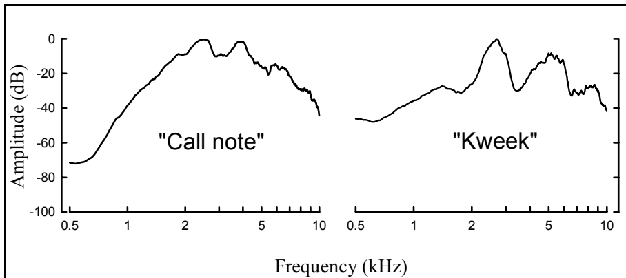
Figure B - 5. Average power spectra of two common vocalizations of the Red-cockaded Woodpecker.
