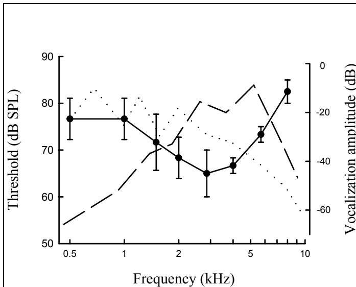
Figure B - 6. Average audiogram for three Downy Woodpeckers (solid line) with superimposed average power spectra for the percussive “drum” (dotted line), and the “call note” vocalization (dashed line) of Downy Woodpeckers.
