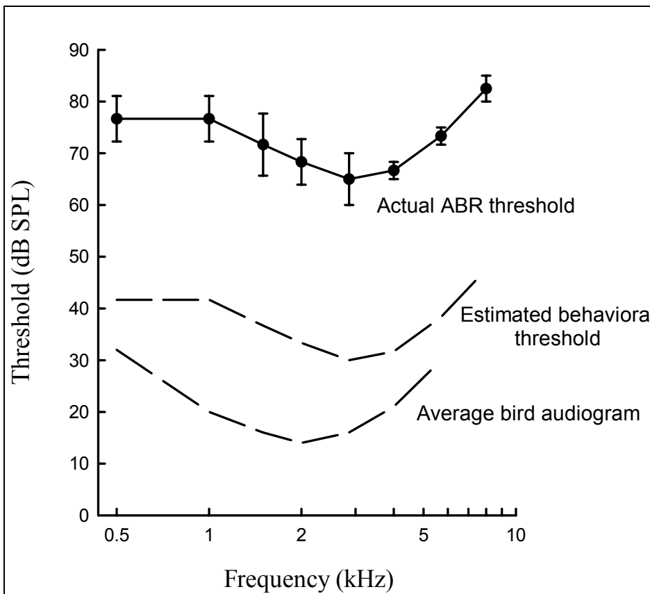
Figure B - 3. Average ABR audiogram for three Downy Woodpeckers (top), audiogram adjusted for absolute difference between physiological and behavioral thresholds (middle), and average passerine audiogram (estimated using behavioral techniques).
