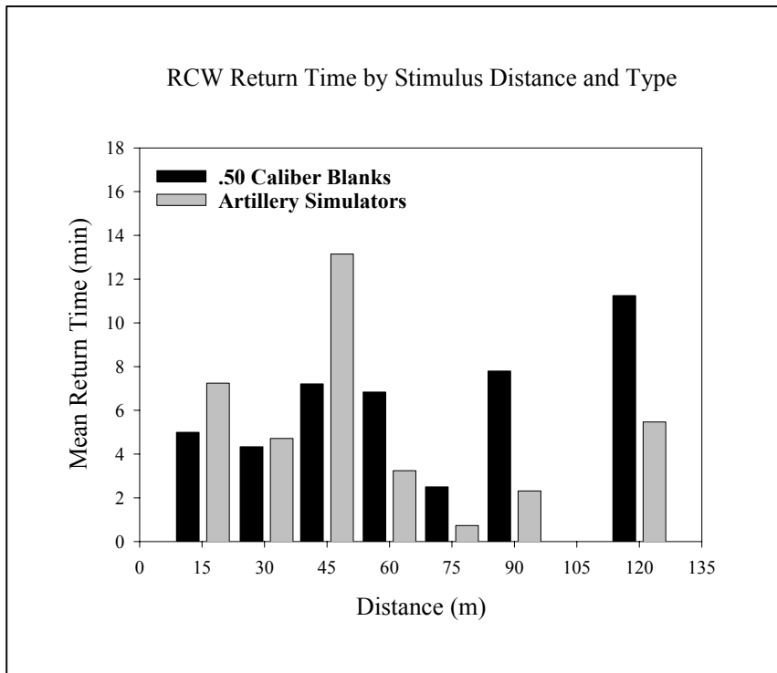
Figure 10. Mean return time for RCW in response to experimental testing in 1999 and 2000.
