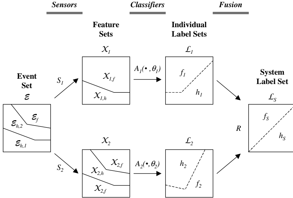
Figure 6: Event, Feature and Label Sets for a Two-Classifier System Combining Decisions Across Target Types
