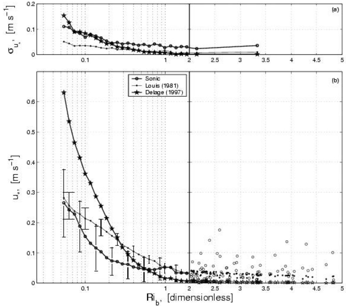
Figure 2: a) \sigma_{u_*} and \sigma_{u_*p} (Louis 1981 [dots] and Delage 1997 [stars]) versus Ri_b and b) u_* and u_*p (Louis 1981 and Delage 1997) versus Ri_b . Insufficient data does not allow the drawing of a meaningful line beyond Ri_b = 2.0 in b). Standard deviation ranges are also shown in b) for some of the data.
