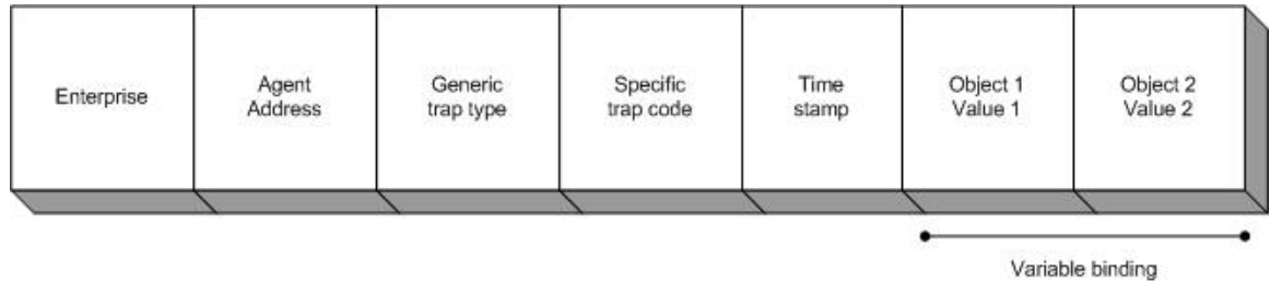
Figure 6 – SNMPv1 Trap PDU From Ref.[03].
