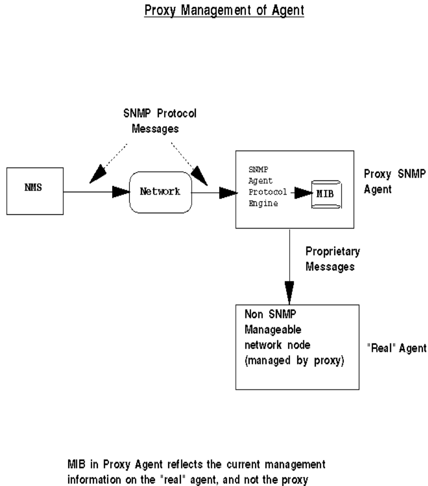
Figure 11 – SNMP Proxy Application Architecture [From: Ref.02.]
