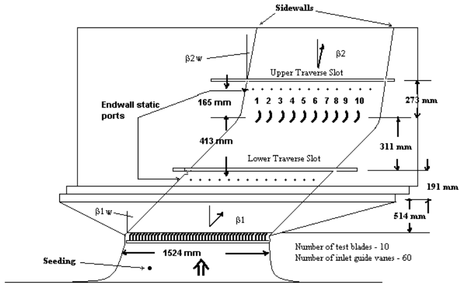
Figure II.2 Test section schematic
