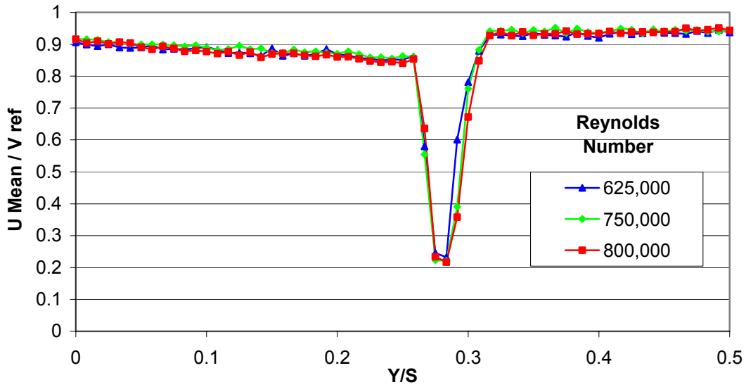
Figure VI.6 Wake mean flow velocity profile at inlet-flow angle of 33 degrees
