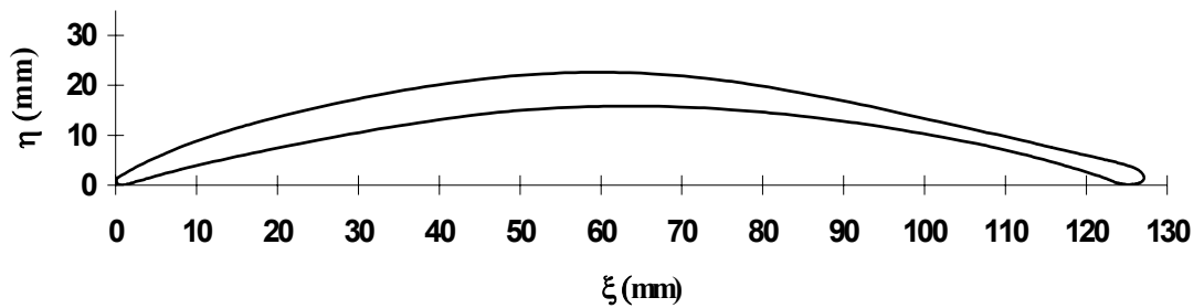
Figure II.3 Blade profile
