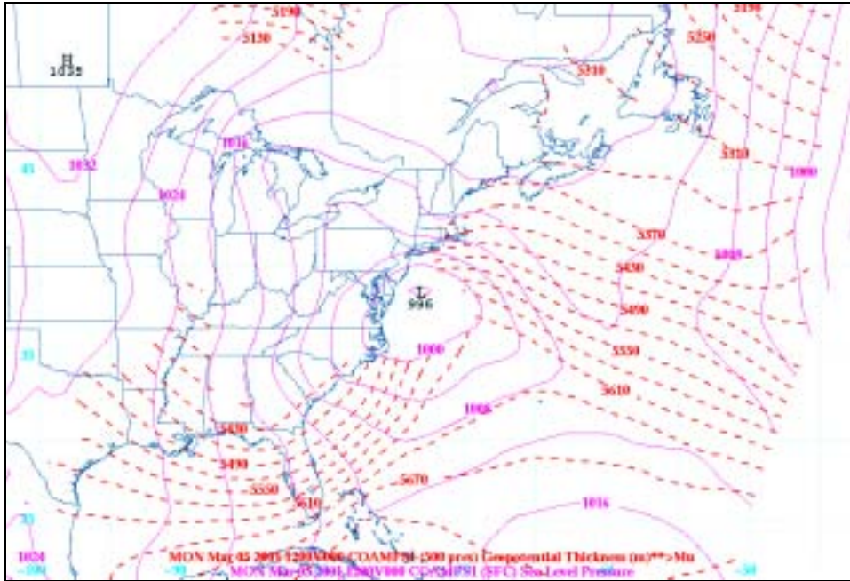
Figure 40. COAMPS Sea Level Pressure and 1000-500mb Geopotential Thickness Contours (1200Z 05MAR01)
