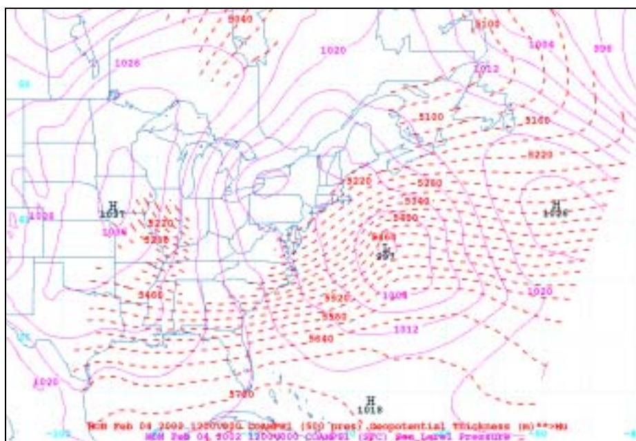
Figure 4. COAMPS Sea Level Pressure and 1000-500mb Geopotential Thickness Contours (1200Z 04FEB02)
