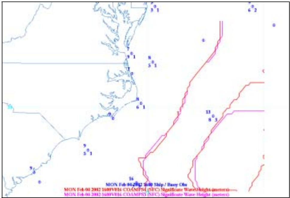
Figure 94. WWIII Significant Wave Height and Observations (February 2002 04/16Z)
