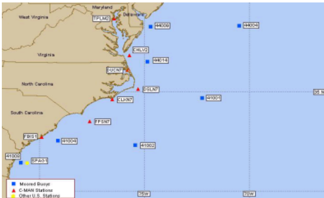
Figure 10. NDBC Buoy Locations Along the Mid-Atlantic Coast
