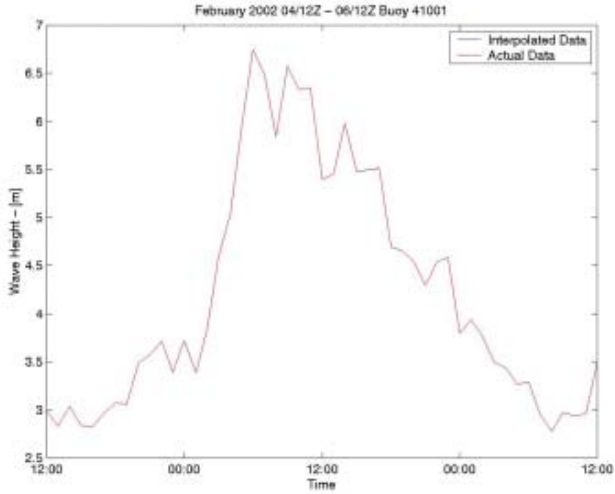
Figure 21. Buoy 41001 Significant Wave Height (February 2002 04/12Z-06/12Z)
