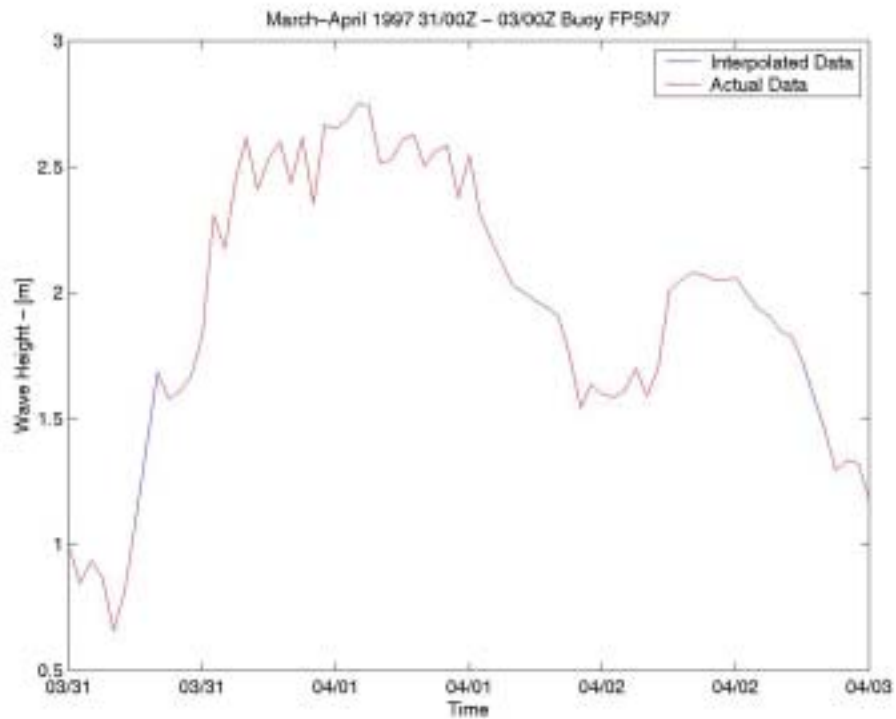
Figure 72. Buoy FPSN7 Significant Wave Height (March-April 1997 31/00Z-03/00Z)
