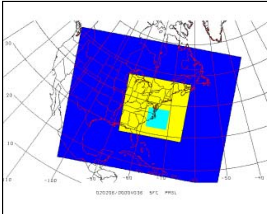
Figure 9. COAMPS 81, 27 and 9 km Nested Grids Used for the Experiment
