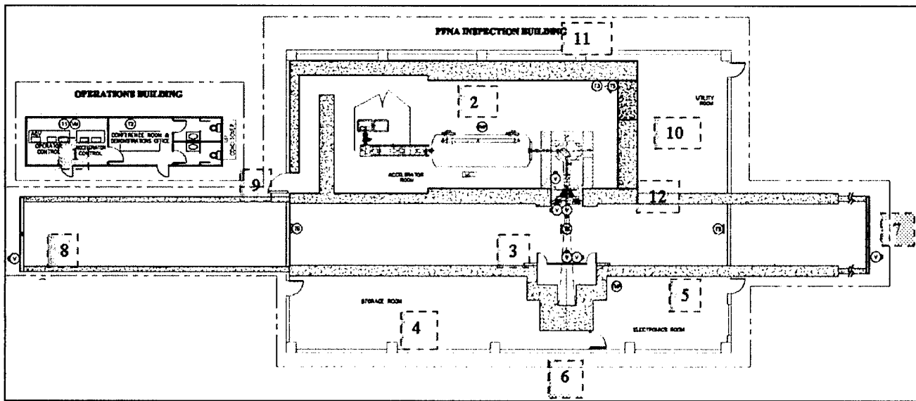
Figure 1.3-2 Survey Points
