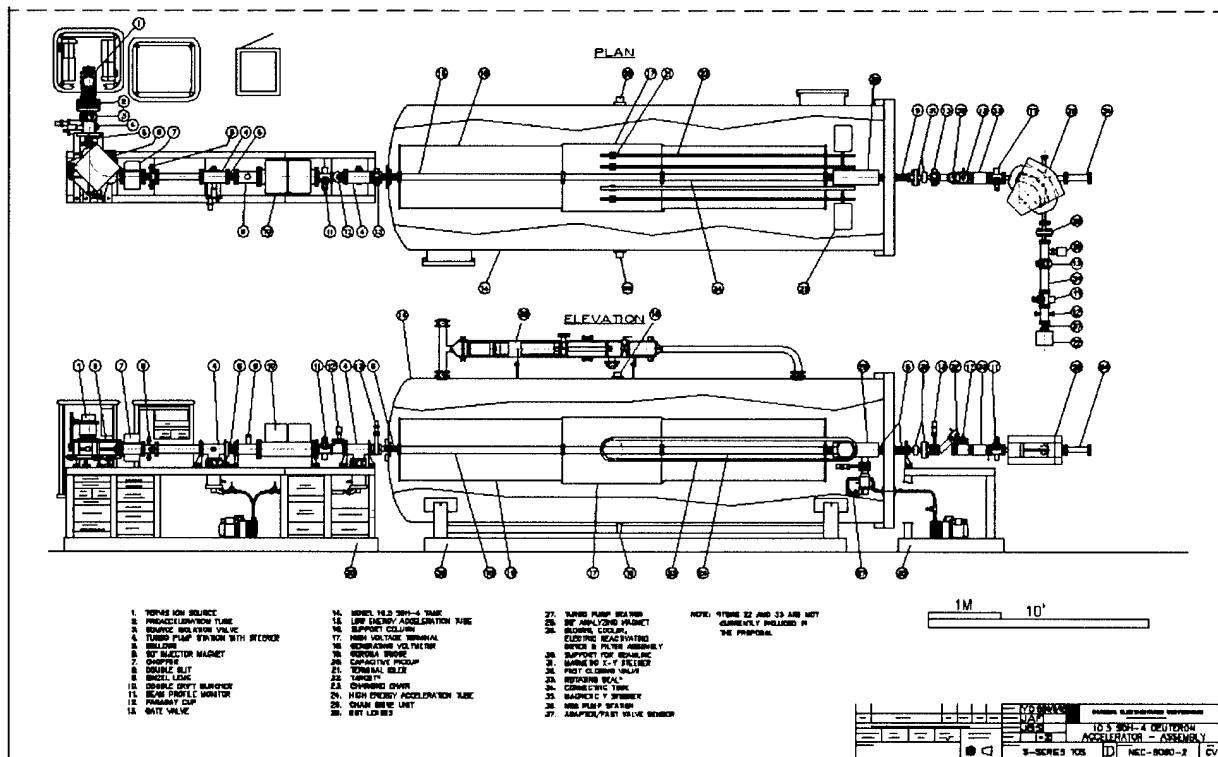
Figure 2.1 Pelletron Accelerator
