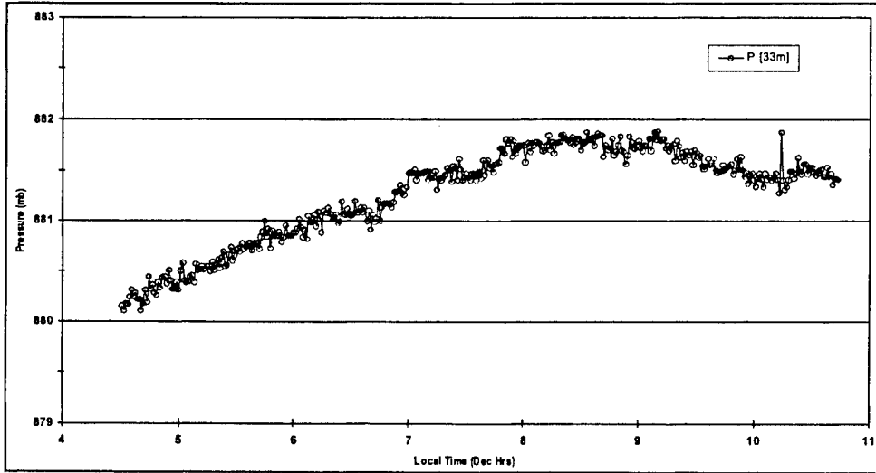
Figure A12. Thompson Tower-2001 June 20: Pressure.
