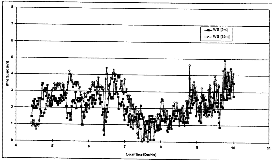
Figure A17. Thompson Tower-2001 June 21: Wind Speed.
