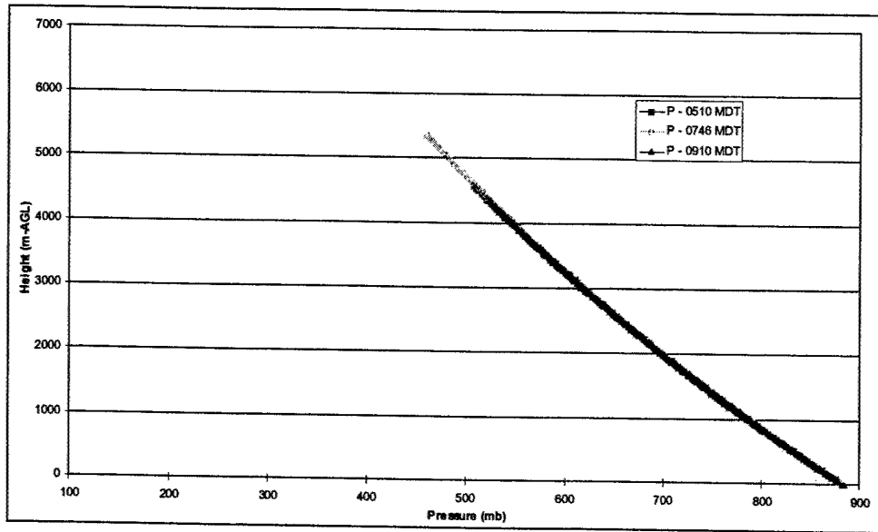
Figure B11. Thompson Tower RAOB Launch-2001 June 20: Pressure.
