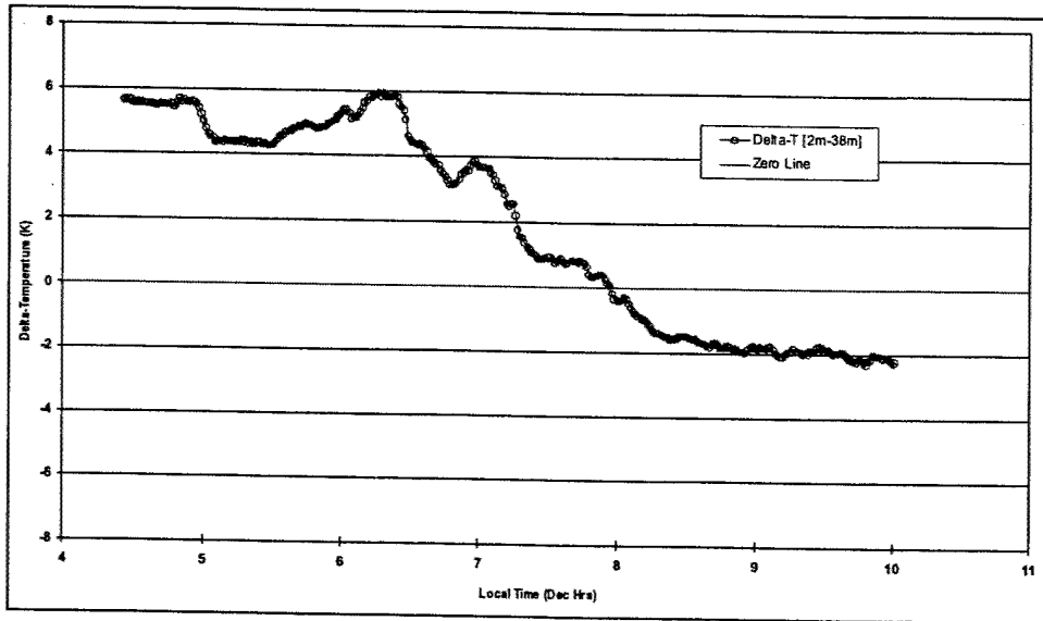
Figure A21. Thompson Tower-2001 June 21: Delta-T.
