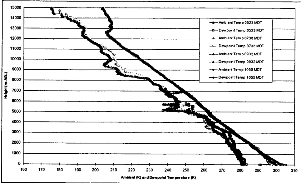
Figure B13. Thompson Tower RAOB Launch-2001 June 21: Temperature.
