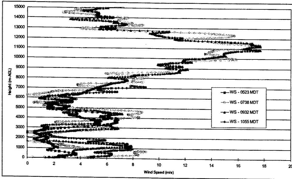
Figure B15. Thompson Tower RAOB Launch-2001 June 21: Wind Speed.
