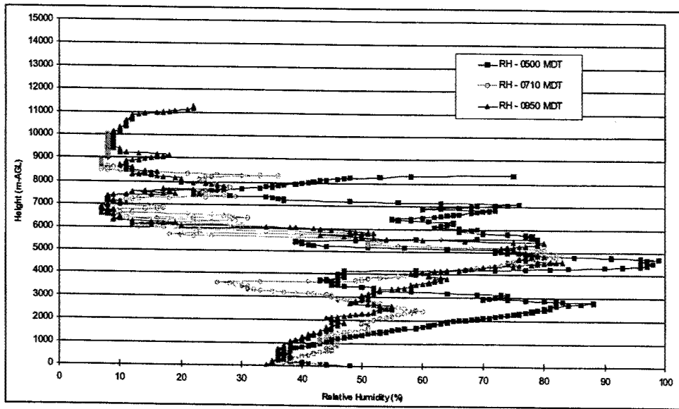
Figure B20. Thompson Tower RAOB Launch-2001 June 22: Relative Humidity.
