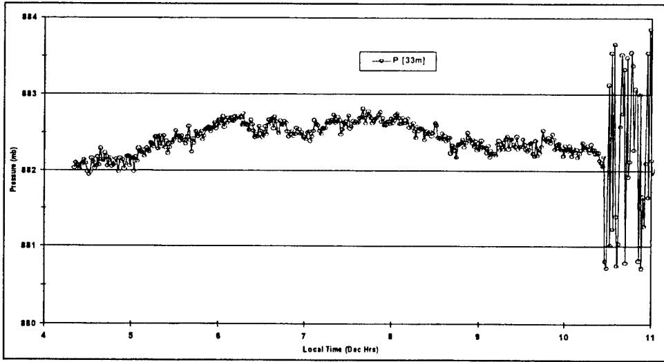
Figure A26. Thompson Tower-2001 June 22: Pressure.
