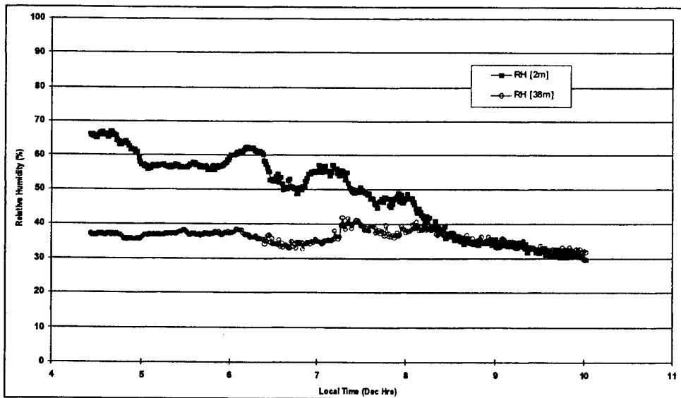
Figure A16. Thompson Tower-2001 June 21: Relative Humidity.
