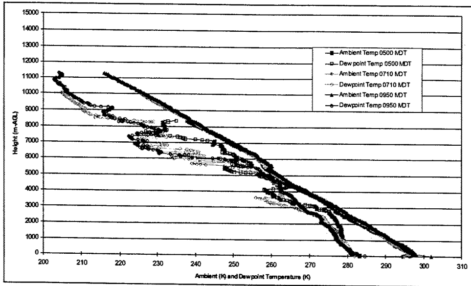
Figure B19. Thompson Tower RAOB Launch-2001 June 22: Temperature.
