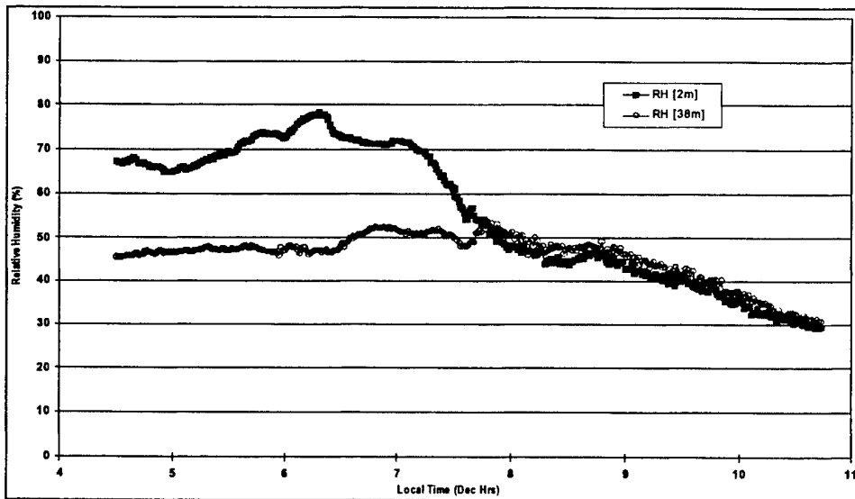
Figure A9. Thompson Tower-2001 June 20: Relative Humidity.
