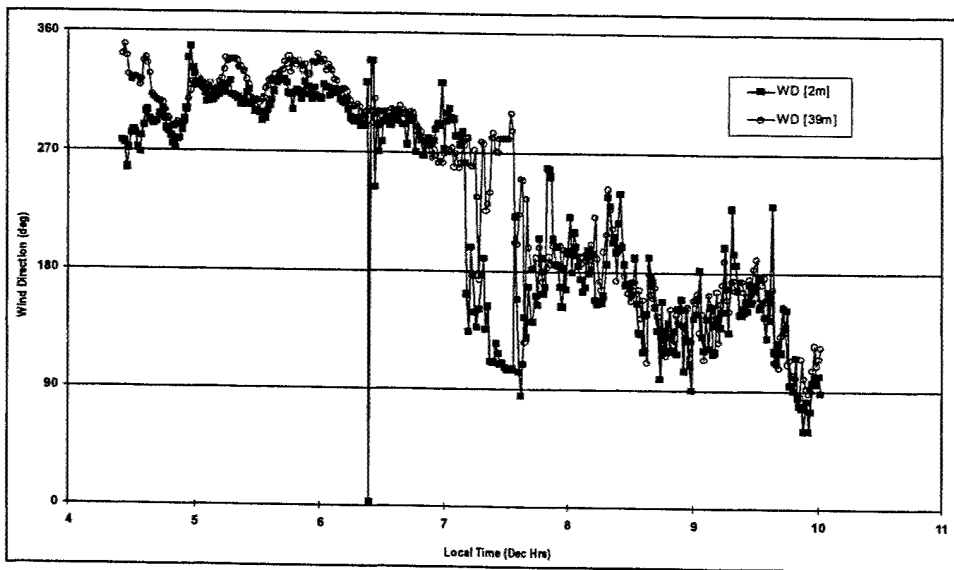
Figure A18. Thompson Tower-2001 June 21: Wind Direction.
