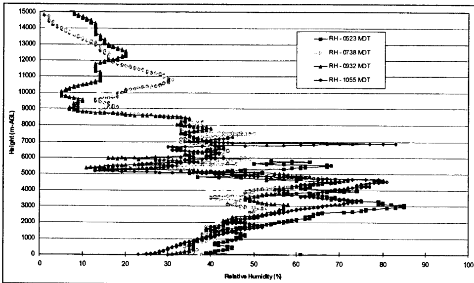
Figure B14. Thompson Tower RAOB Launch-2001 June 21: Relative Humidity.
