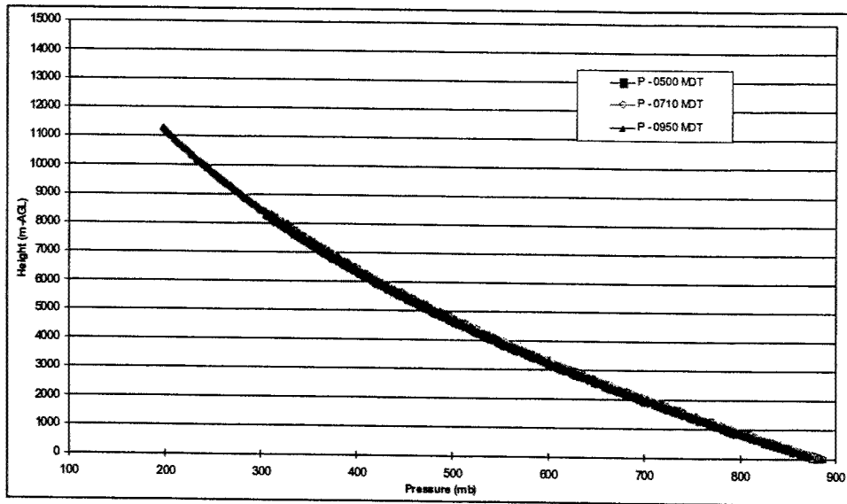
Figure B23. Thompson Tower RAOB Launch-2001 June 22: Pressure.
