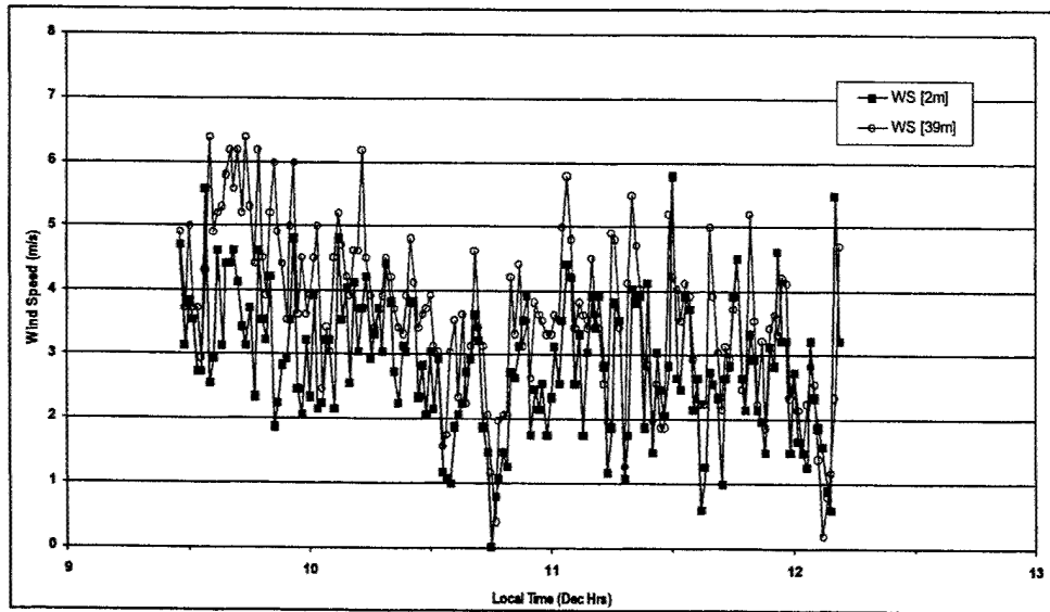
Figure A3. Thompson Tower-2001 June 19: Wind Speed.
