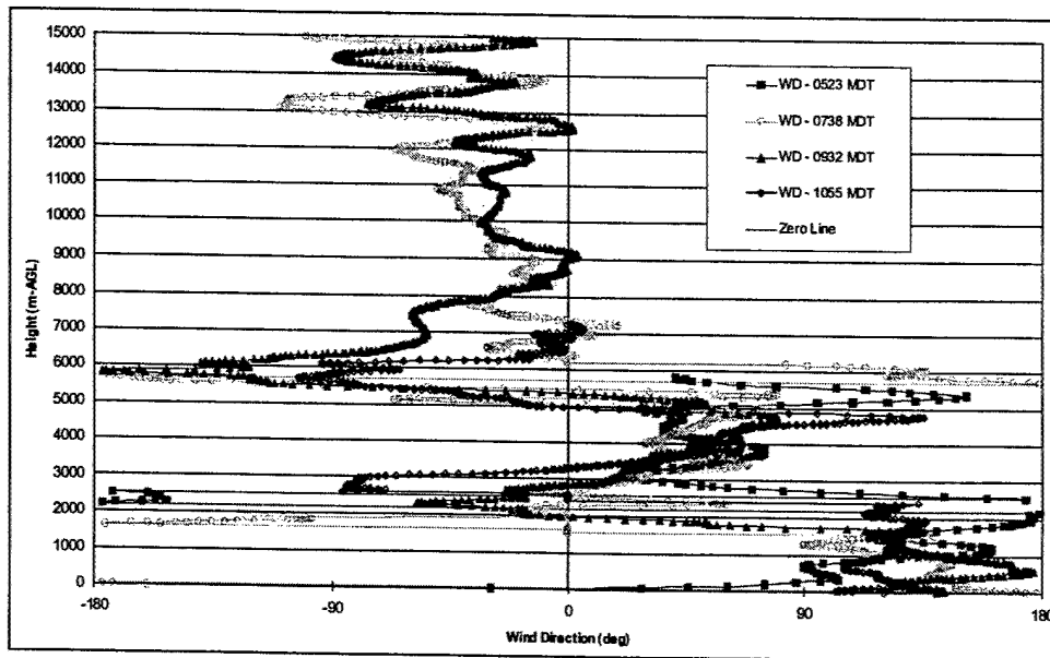
Figure B16. Thompson Tower RAOB Launch-2001 June 21: Wind Direction.
