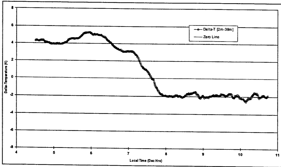
Figure A14. Thompson Tower-2001 June 20: Delta-T.
