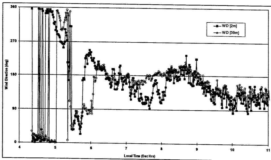
Figure A25. Thompson Tower-2001 June 22: Wind Direction.
