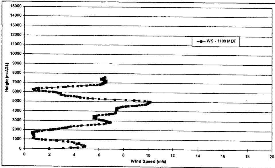
Figure B3. Thompson Tower RAOB Launch-2001 June 19: Wind Speed.
