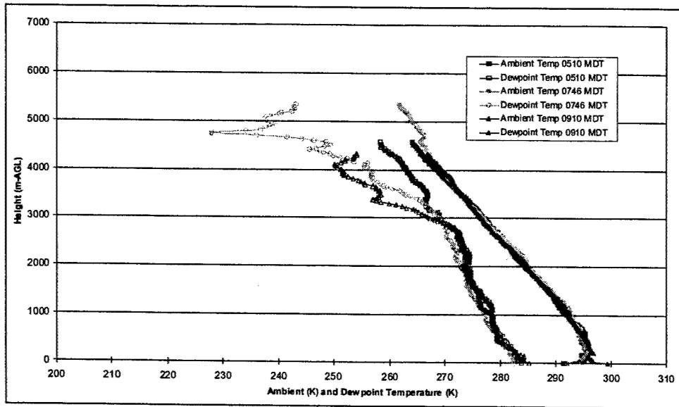
Figure B7. Thompson Tower RAOB Launch-2001 June 20: Temperature.
