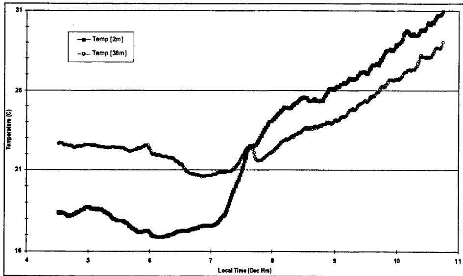
Figure A8. Thompson Tower-2001 June 20: Temperature.
