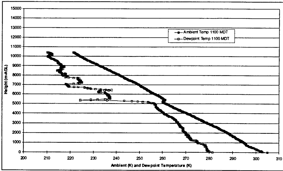
Figure B1. Thompson Tower RAOB Launch-2001 June 19: Temperature.
