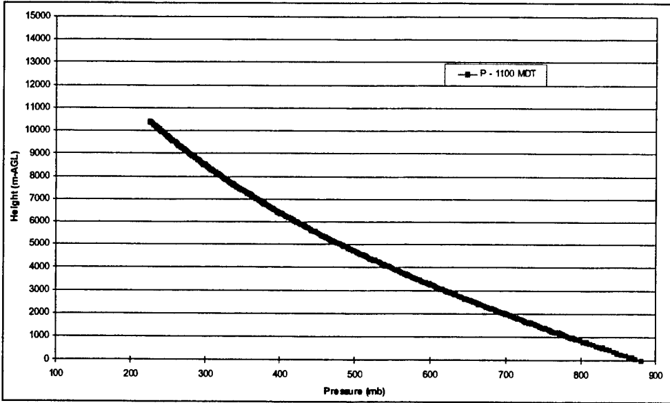
Figure B5. Thompson Tower RAOB Launch-2001 June 19: Pressure.
