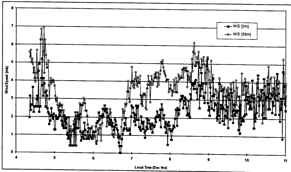
Figure A24. Thompson Tower-2001 June 22: Wind Speed.
