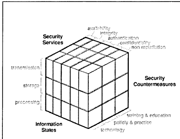
Figure 3. IA model (47).
