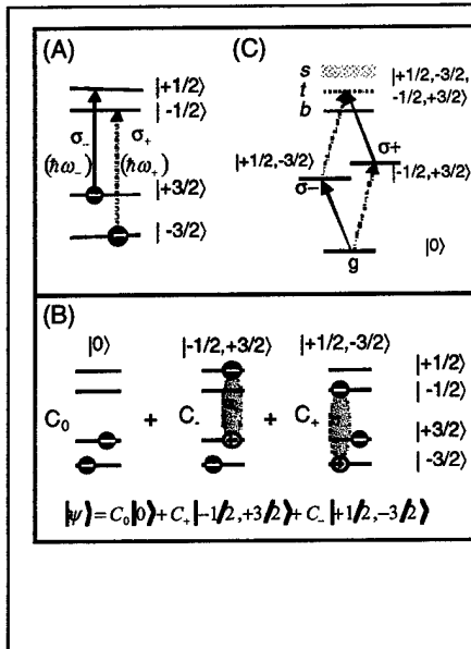
Figure 1. (A) Energy level diagram for two electron in a single QD. In this system, the appropriate quantum numbers reflect the fact that two electrons sit in the valence band characterized by M_j quantum numbers -3/2 and +3/2 . The excited state corresponds to conduction band M_j quantum numbers -1/2 and +1/2 . The usual optical dipole selection rules apply in this problem. (B) Optical manipulation of the system in (A) leads to two-exciton entanglement. (C) The energy levels in (A) are displayed in a single Hilbert space. In this case, if there is no interaction between the two-exciton systems, then state t corresponds to the case where both states are excited. However, in the presence of an interaction, either a bound state b or scattering state s is produced with a resultant energy shift with respect to state t .
