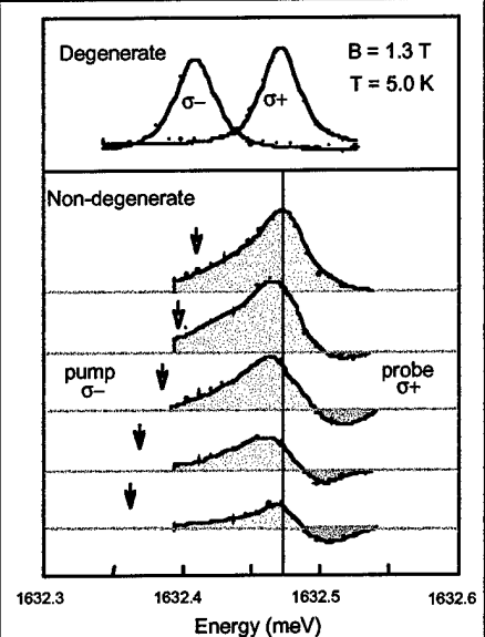
Figure 3. Non-degenerate coherent nonlinear response of a single QD. The pump is placed at the \sigma_- (lower) state with \sigma_- polarization. The probe is scanned across the \sigma_+ state (upper) with \sigma_+ polarization. The results show an interference lineshape identifying the contribution from the Zeeman coherence, implying two-exciton entanglement.
