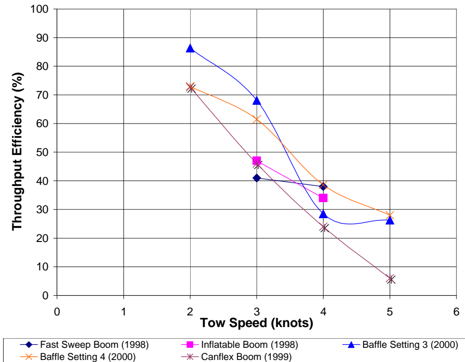
Figure 19. Graph of HSS Historic and 2000 Data.
