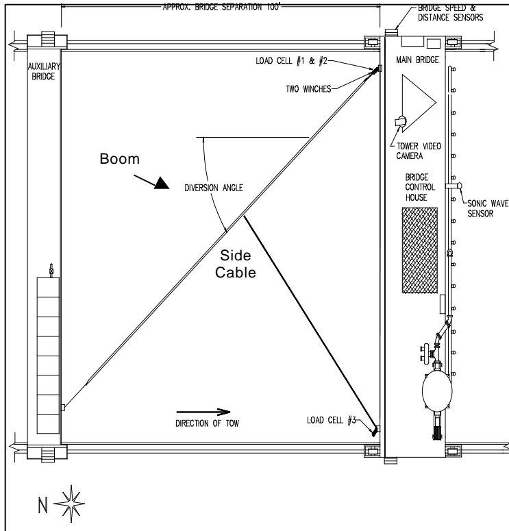
Figure 21. Test Setup for Towing Forces on Fast Water Diversion Booms.
