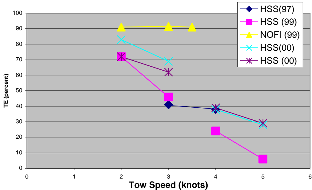
Figure 44. Throughput Efficiency Performance with Hydrocal in Calm Water.
