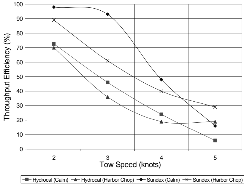
Figure 10. Throughput Efficiency versus Tow Speed.
