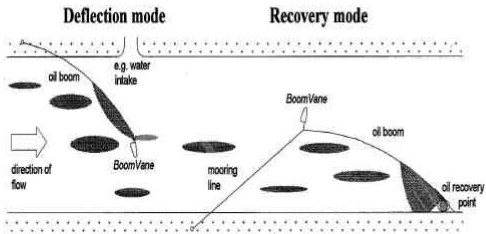
Figure 4. Boom Vane Deployment Modes.
