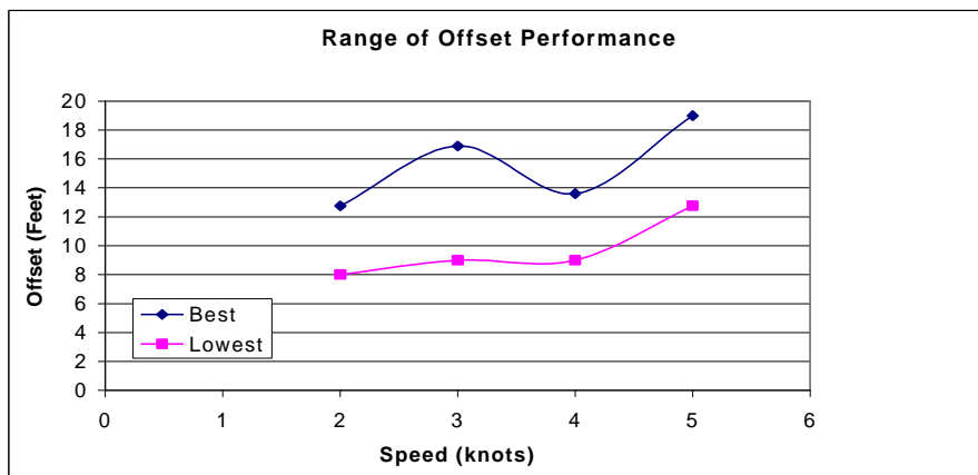
Figure 25. Displacement of Oil at Various Speeds.
