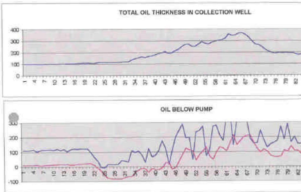
Figure 37. Sample Oil Thickness Data.
