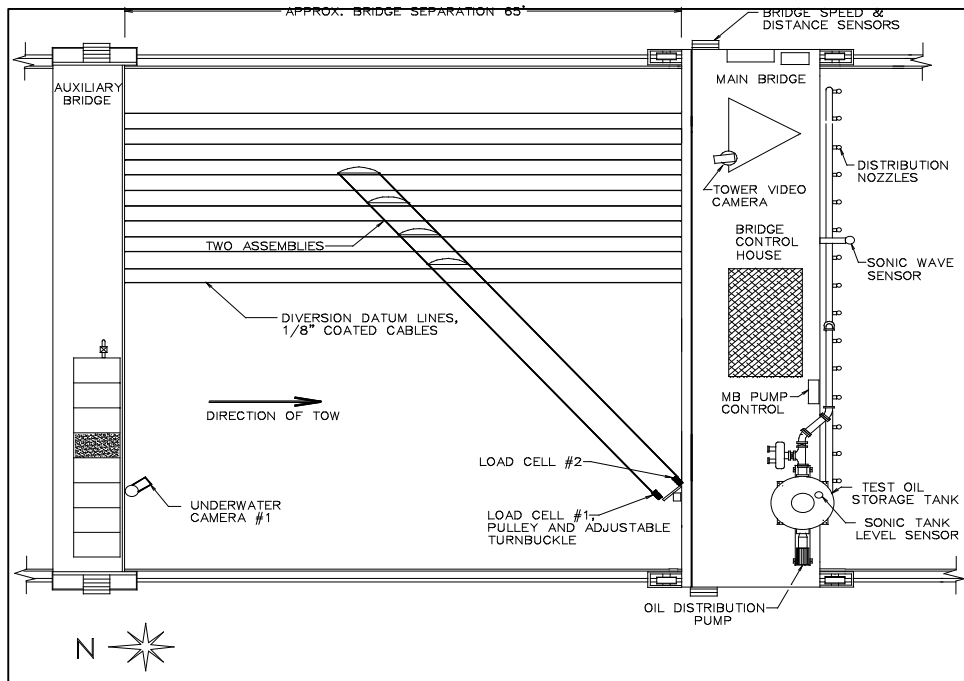
Figure 24. Flow Diverter Test Setup.
