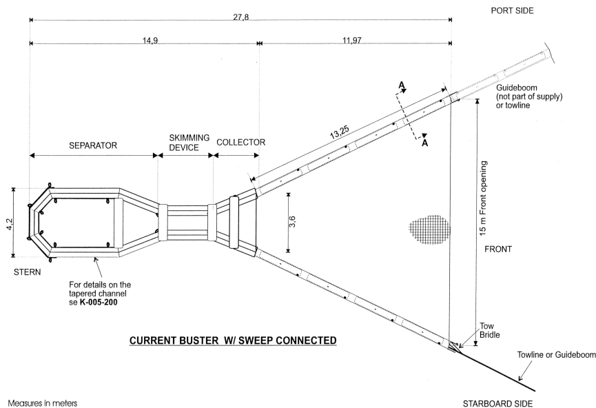
Figure 16. Current Buster Skimmer with Sweep Boom Connected.
