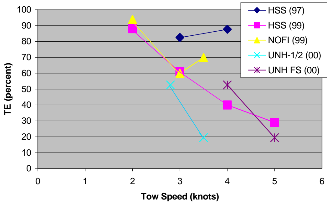
Figure 43. Throughput Efficiency Performance with Sundex Oil in Harbor Chop.
