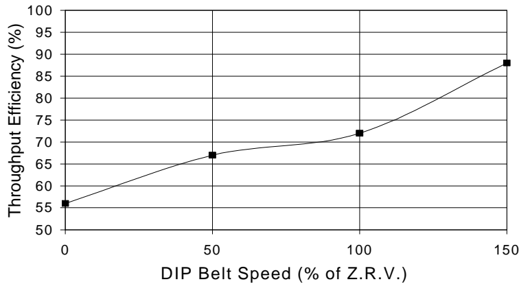
Figure 11. Throughput Efficiency versus Belt Speed for Hydrocal Oil.
