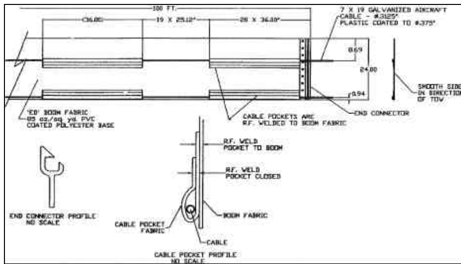
Figure 20. Test Boom Components.
