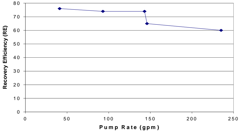
Figure 12. Recovery Efficiency versus Pump Rate for HSS.
