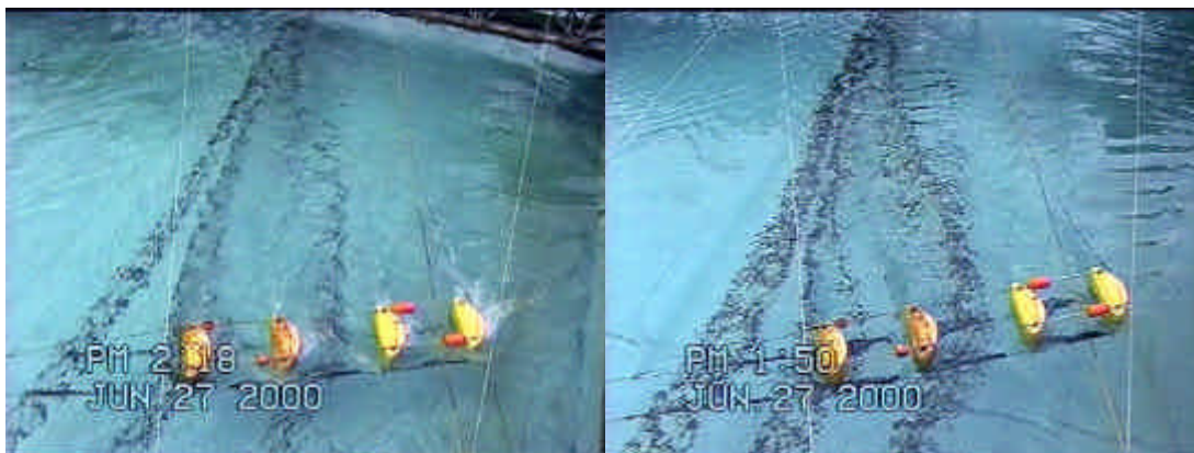
Figure 26. Four Paravanes at 2 Knots (left) and 3 Knots (right).
