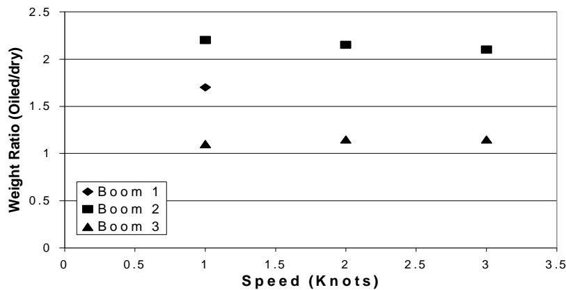
Figure 30. Sorbent Boom Performance.
