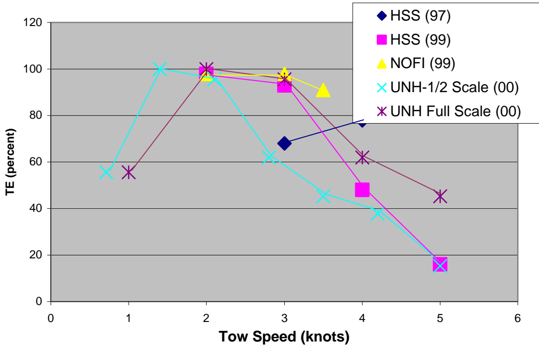
Figure 42. Throughput Efficiency Performance with Sundex Oil in Calm Water.
