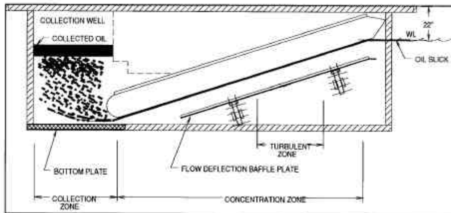
Figure 18. Cross-section of the HSS with Baffle Plate Installed.
