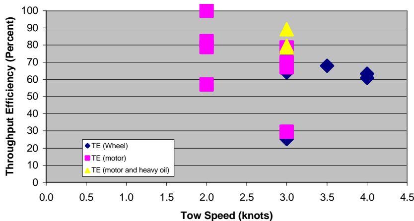
Figure 33. Throughput Efficiency Performance of Stream Stripper.
