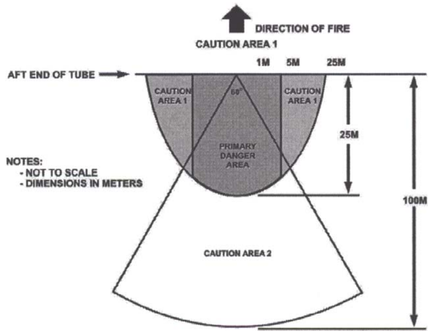
Figure 24: Javelin Back-blast Safety Zone [From Ref. 39]
