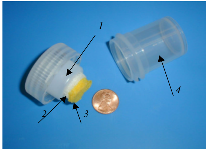
Figure 10. Picture of Agentase Traffic Light Sensor (1 st generation prototype)
