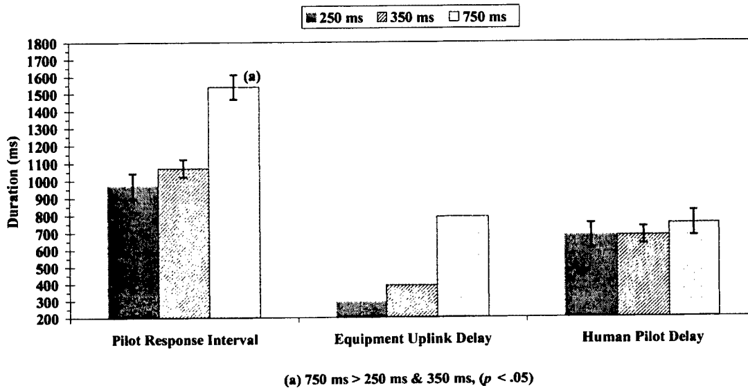
Figure 7. Mean pilot response interval, equipment uplink delay, and human pilot delay-by-condition.
