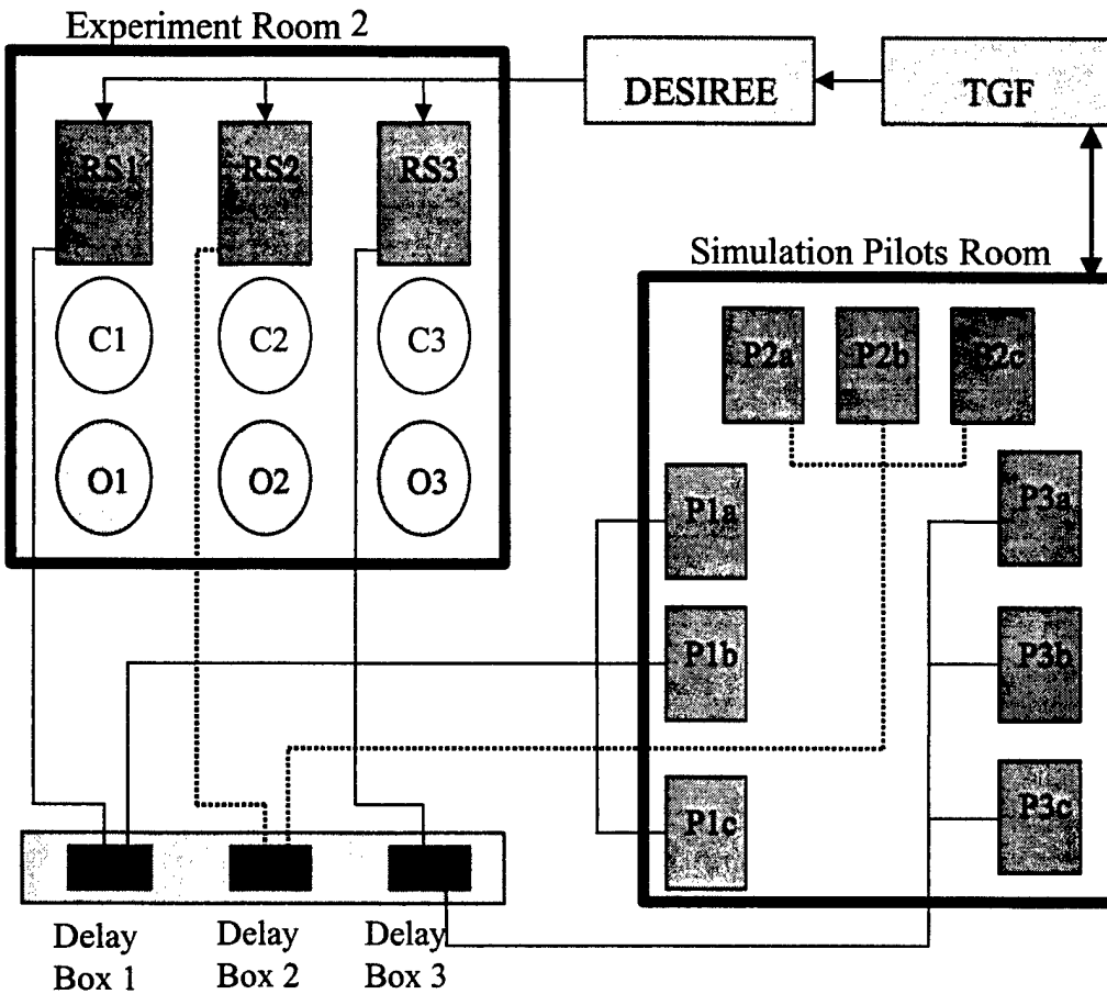
Figure 1. Diagram (not to scale) of the test facility (RS = radar scope, C = controller, O = observer, P = pilot).
