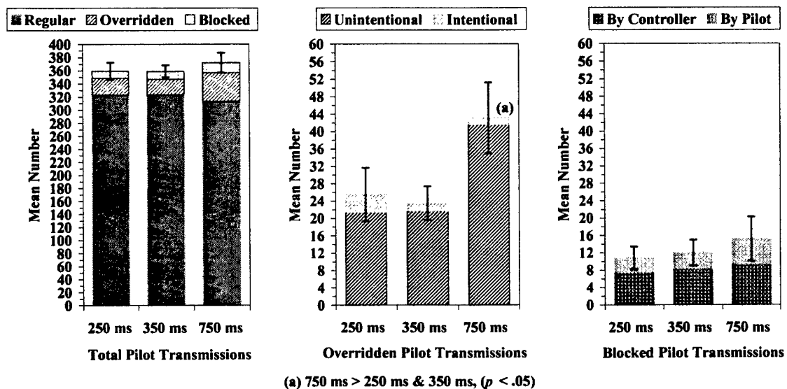
Figure 6. Mean number of regular, overridden, and blocked pilot transmissions by delay condition.
