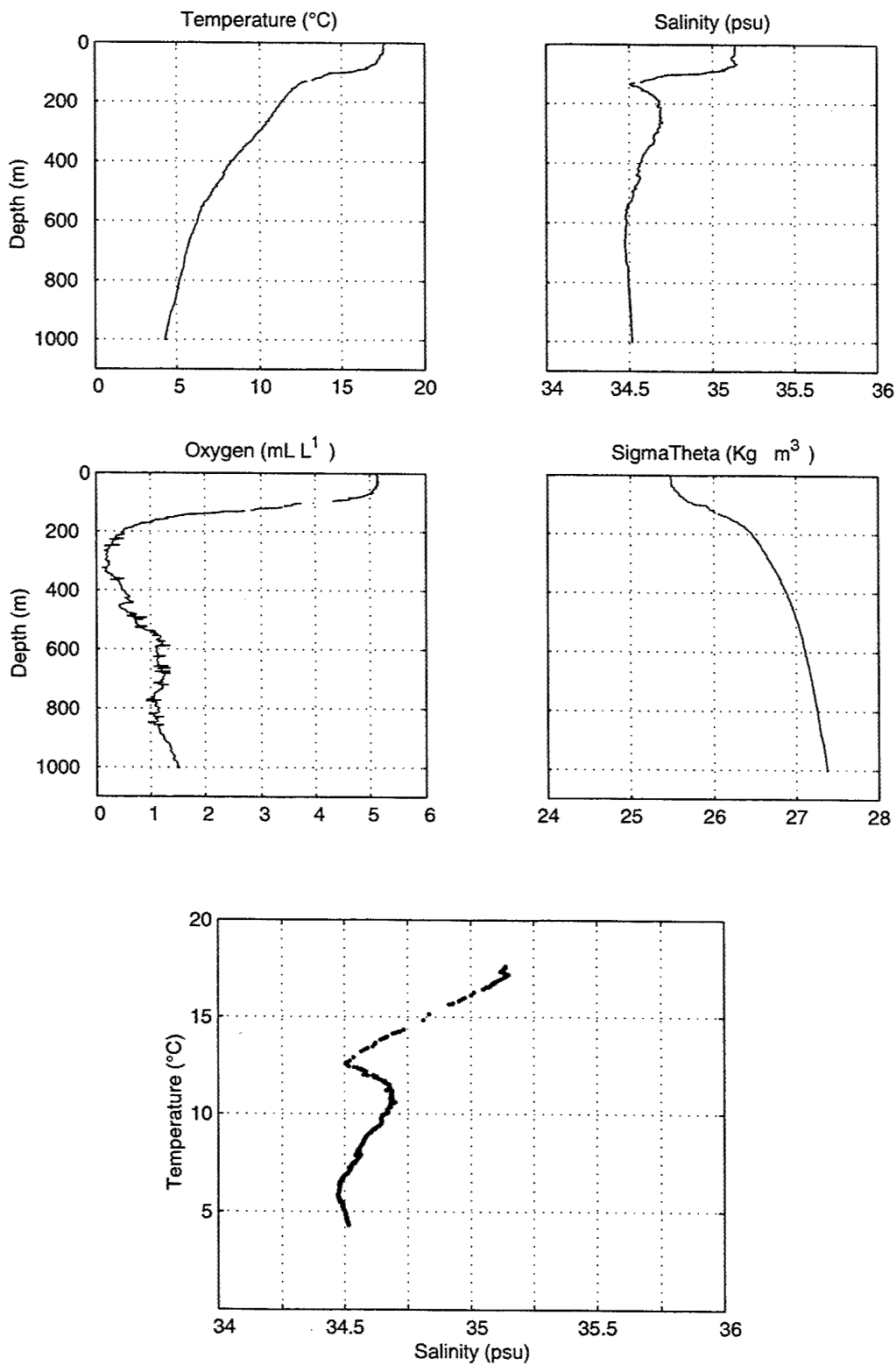
Figure 40. Stratus 11 CTD Cast.
