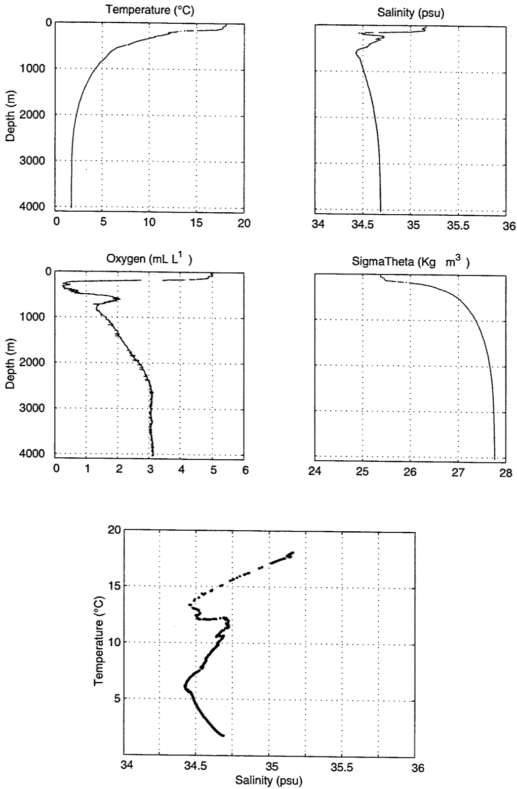
Figure 30. Stratus 01 CTD Cast.
