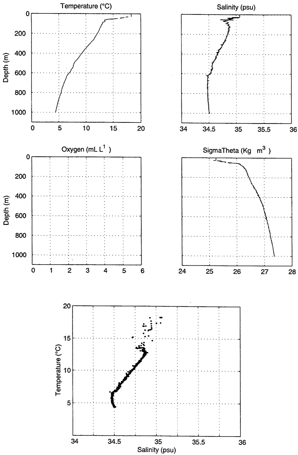
Figure 54. Stratus 18 CTD Cast, SBE 19 Data.
