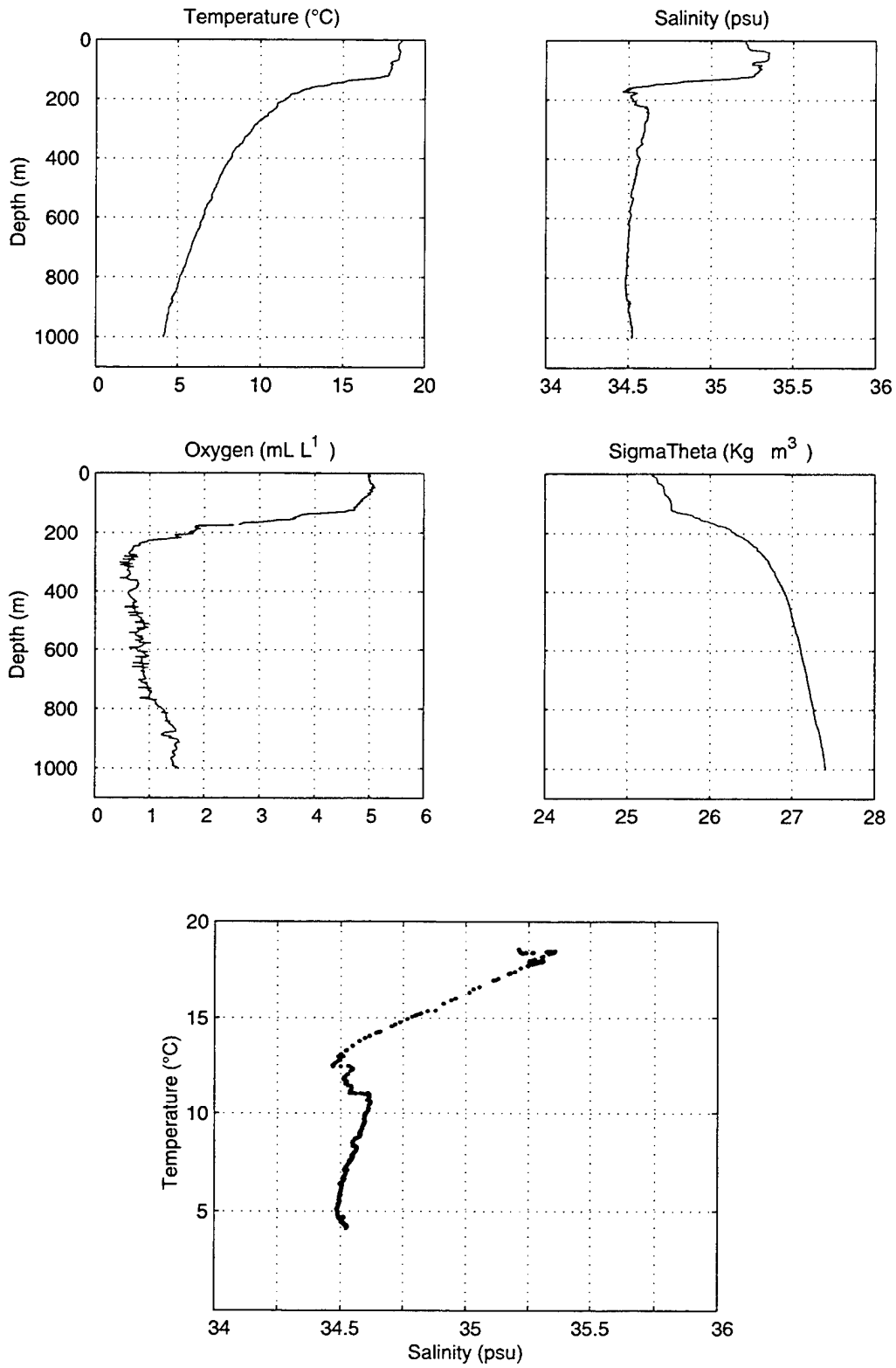
Figure 35. Stratus 06 CTD Cast.
