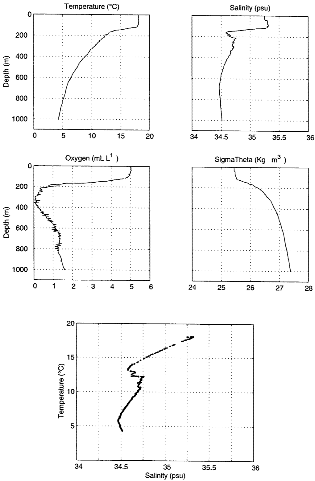
Figure 38. Stratus 09 CTD Cast.
