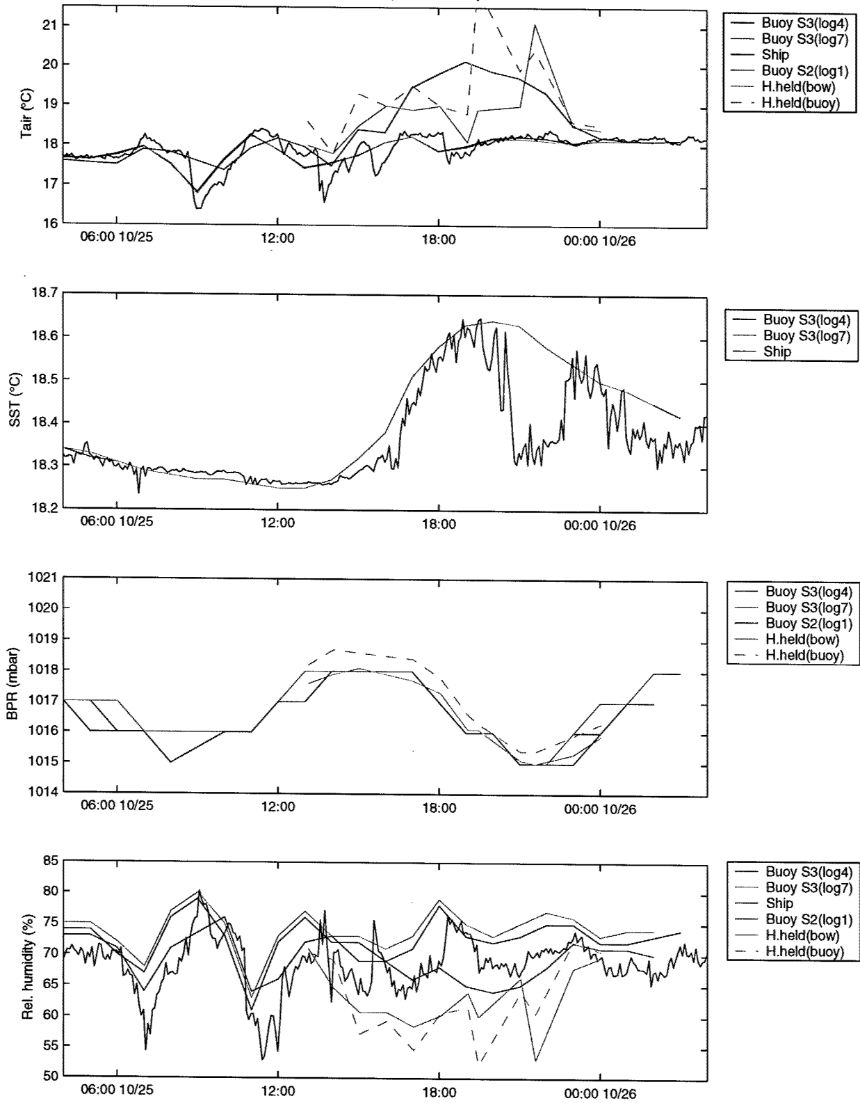
Stratus 3 buoy v ship data comparison
