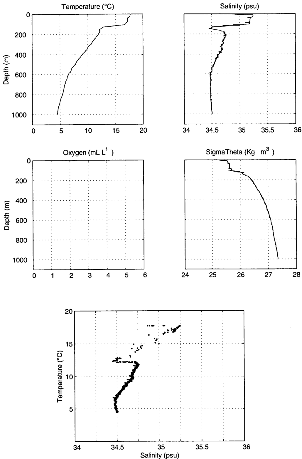
Figure 43. Stratus 12 CTD Cast, SBE 19 Data.
