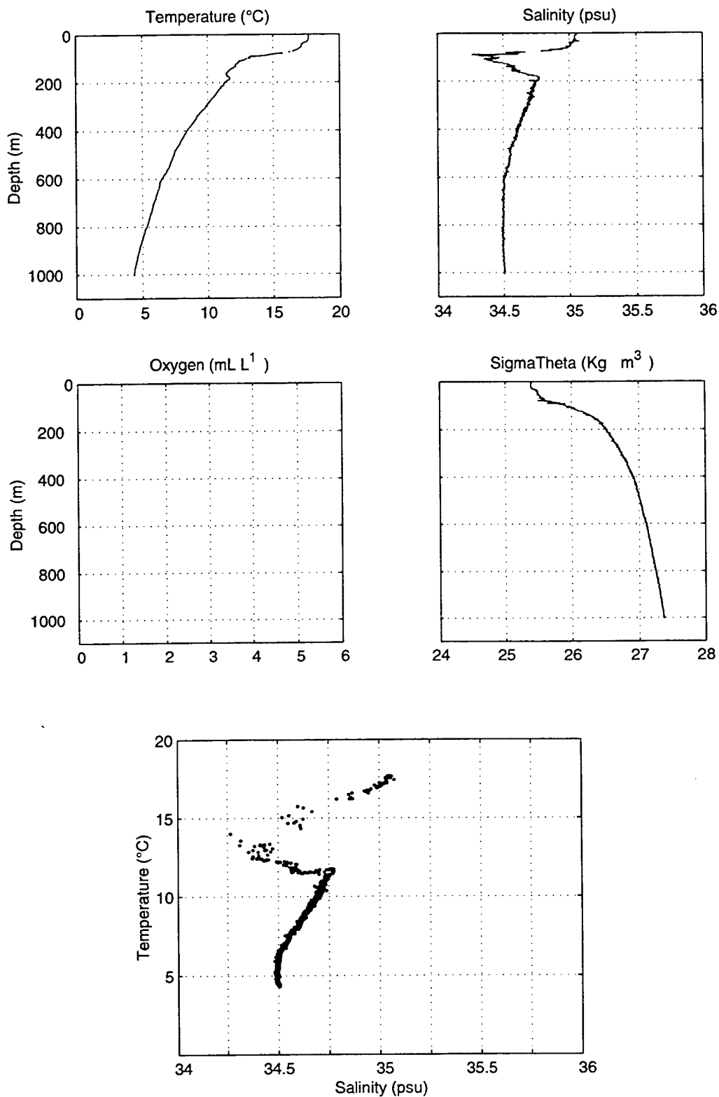
Figure 51. Stratus 16 CTD Cast, SBE 19 Data.
