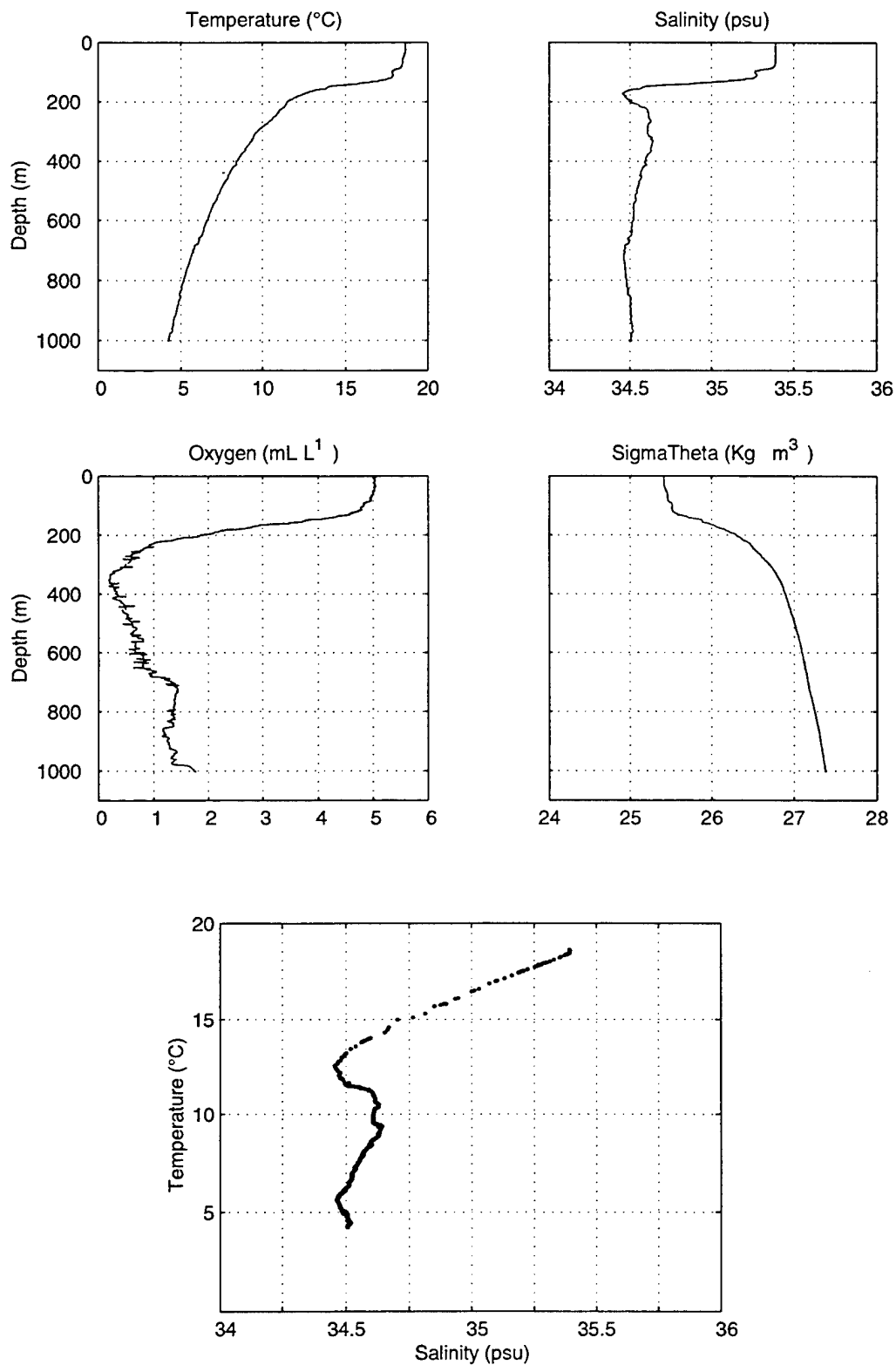
Figure 37. Stratus 08 CTD Cast.
