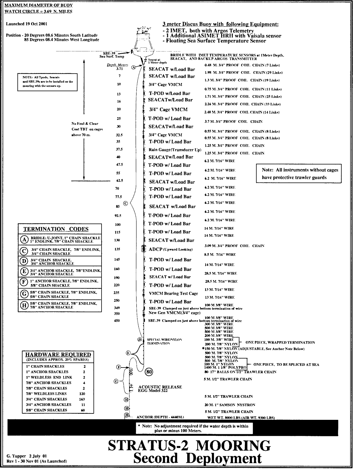
Figure 6. Stratus 2 Mooring Diagram.
