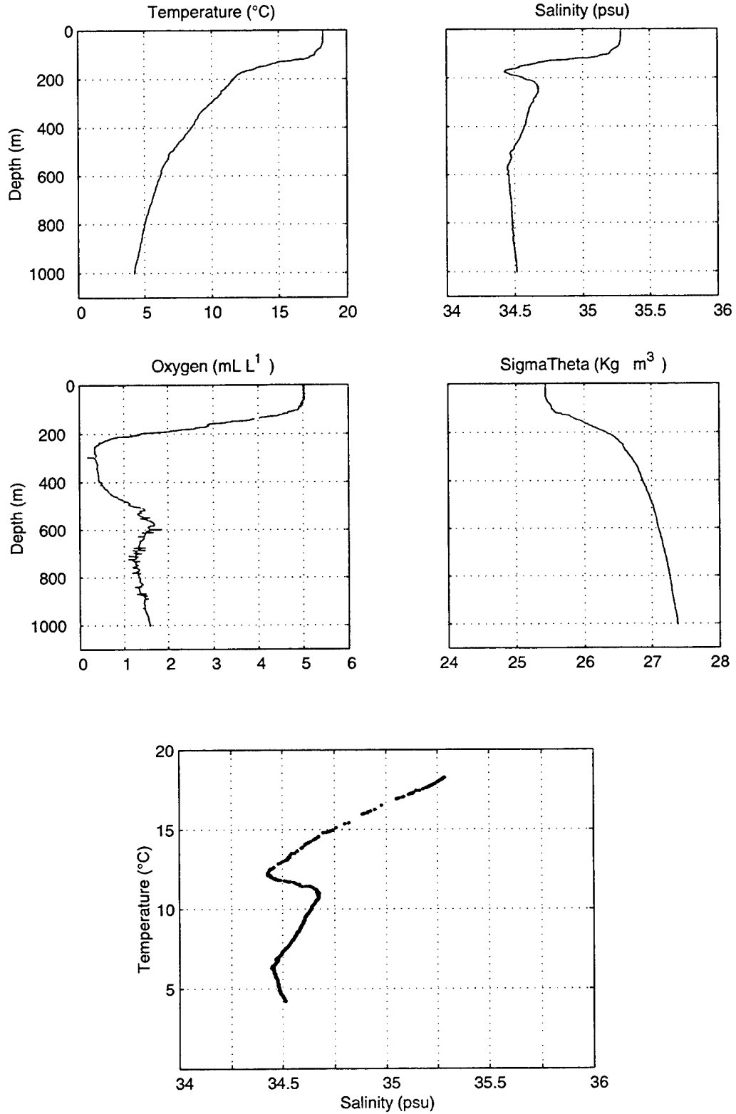
Figure 39. Stratus 10 CTD Cast.
