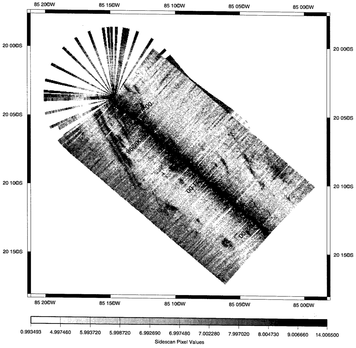
Figure 61. Sidescan sonar taken on October 23, 2002.
