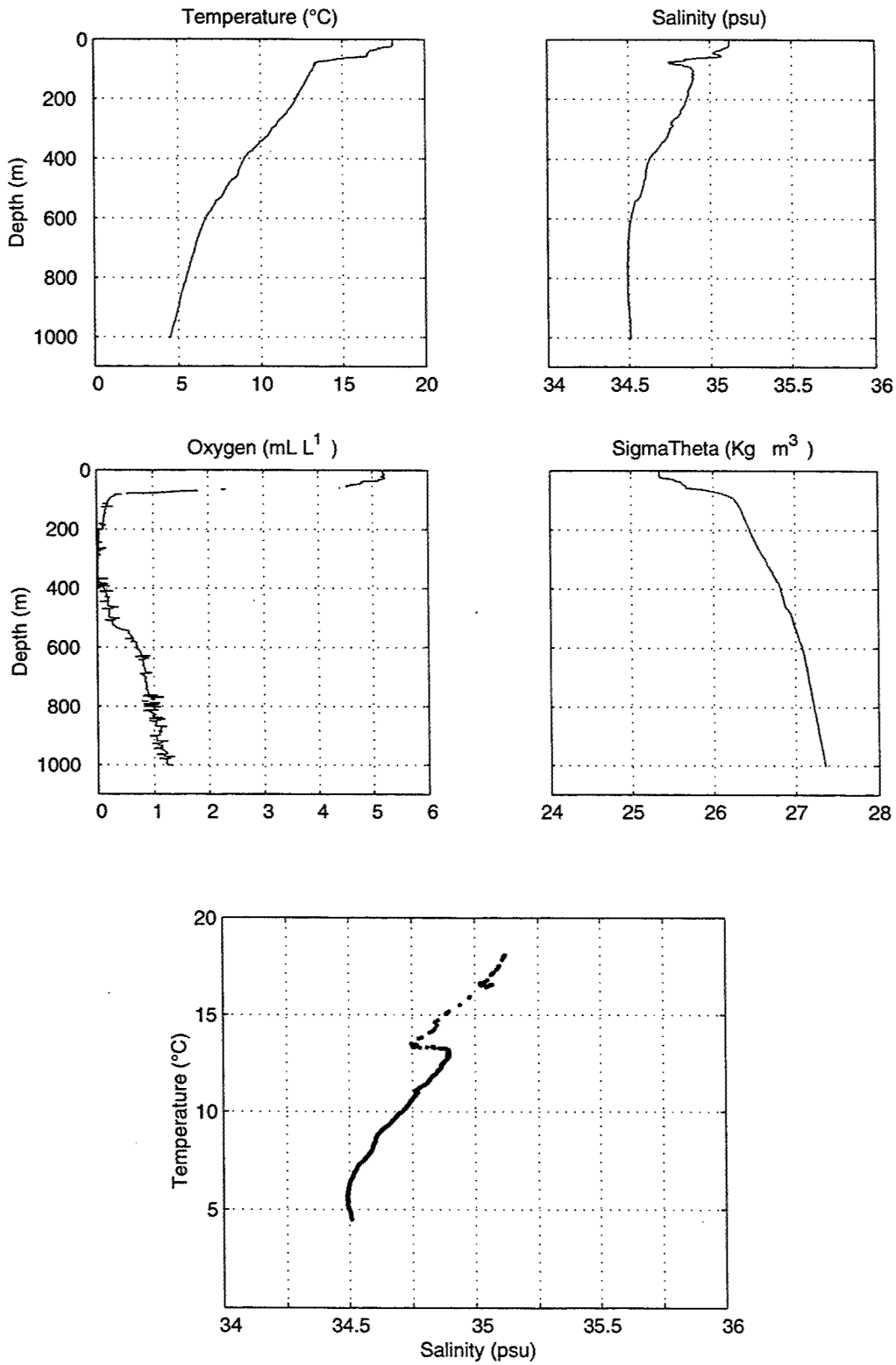
Figure 52. Stratus 17 CTD Cast.
