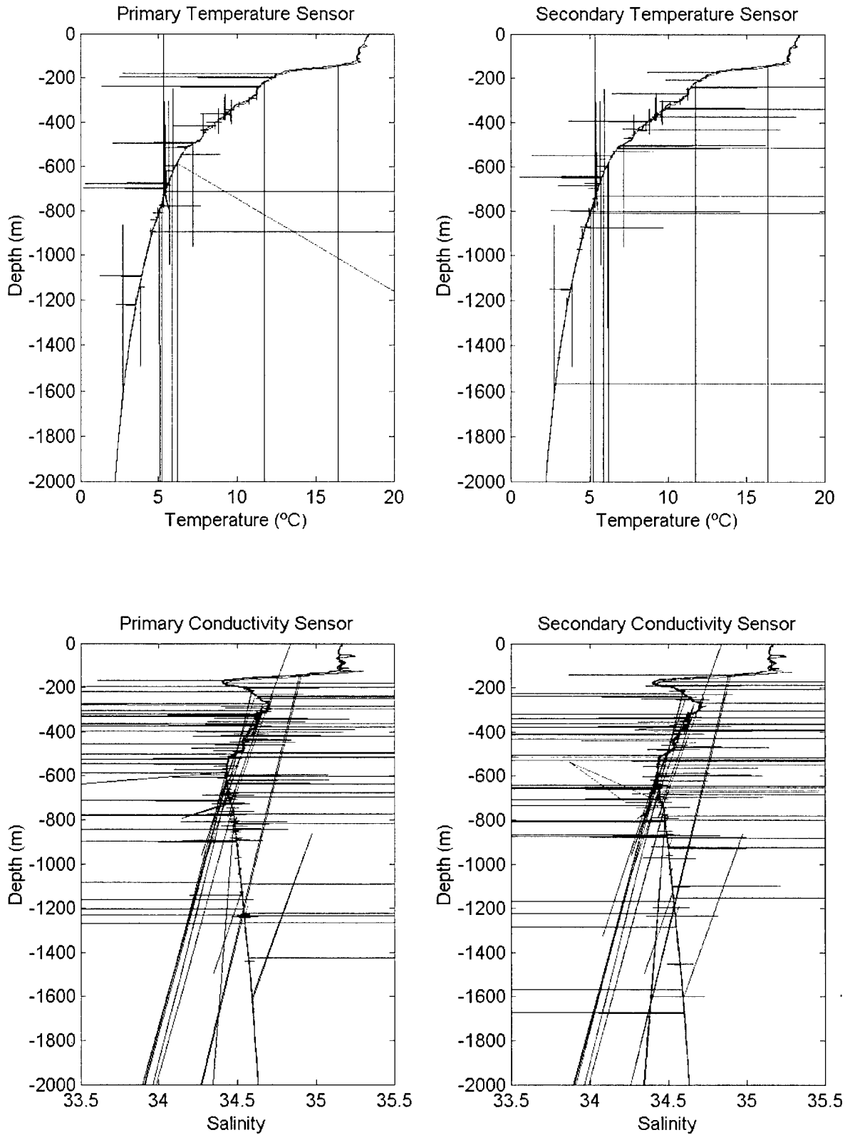
Figure 27. Raw CTD data with spikes.
