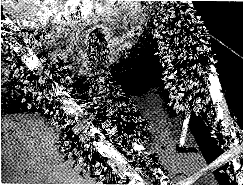
Figure 3. Bio-fouling on buoy and bridle.
