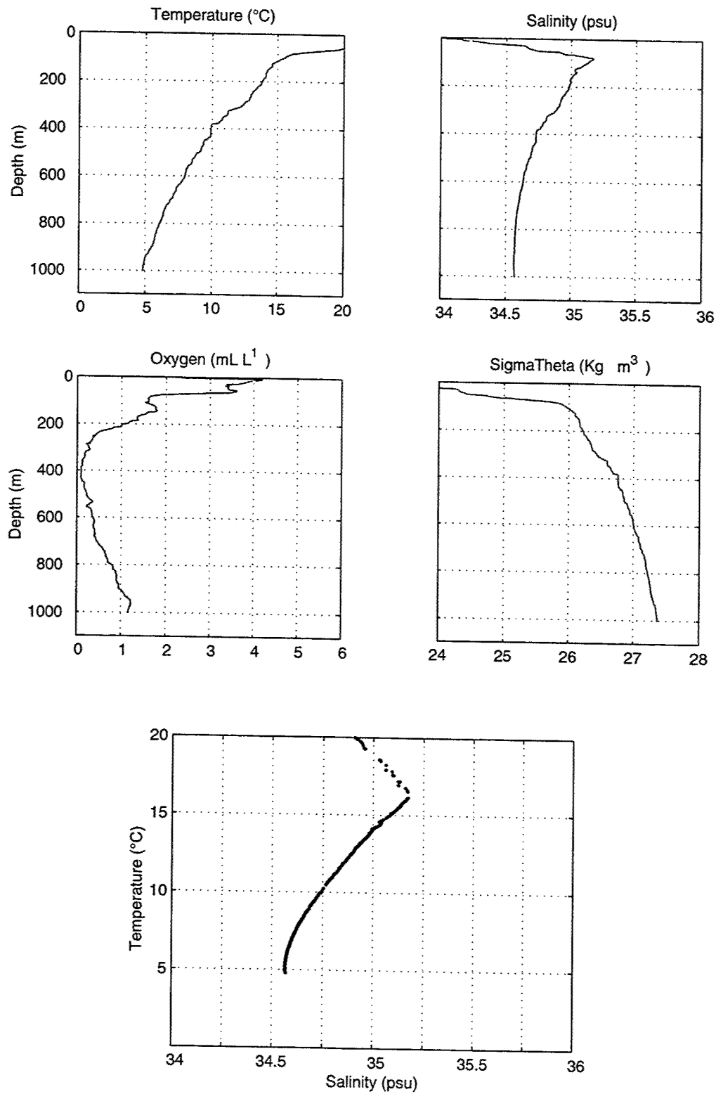
Figure 28. Stratus 00 CTD Cast.
