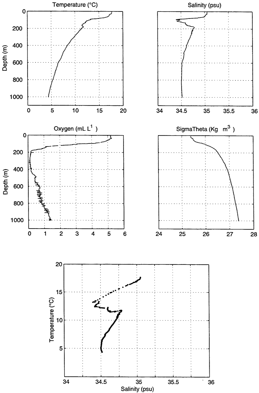
Figure 50. Stratus 16 CTD Cast.
