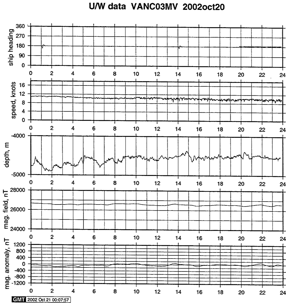
Figure 59. An example plot showing ship's true heading, speed, water depth, magnetic field, and magnetic anomaly.
