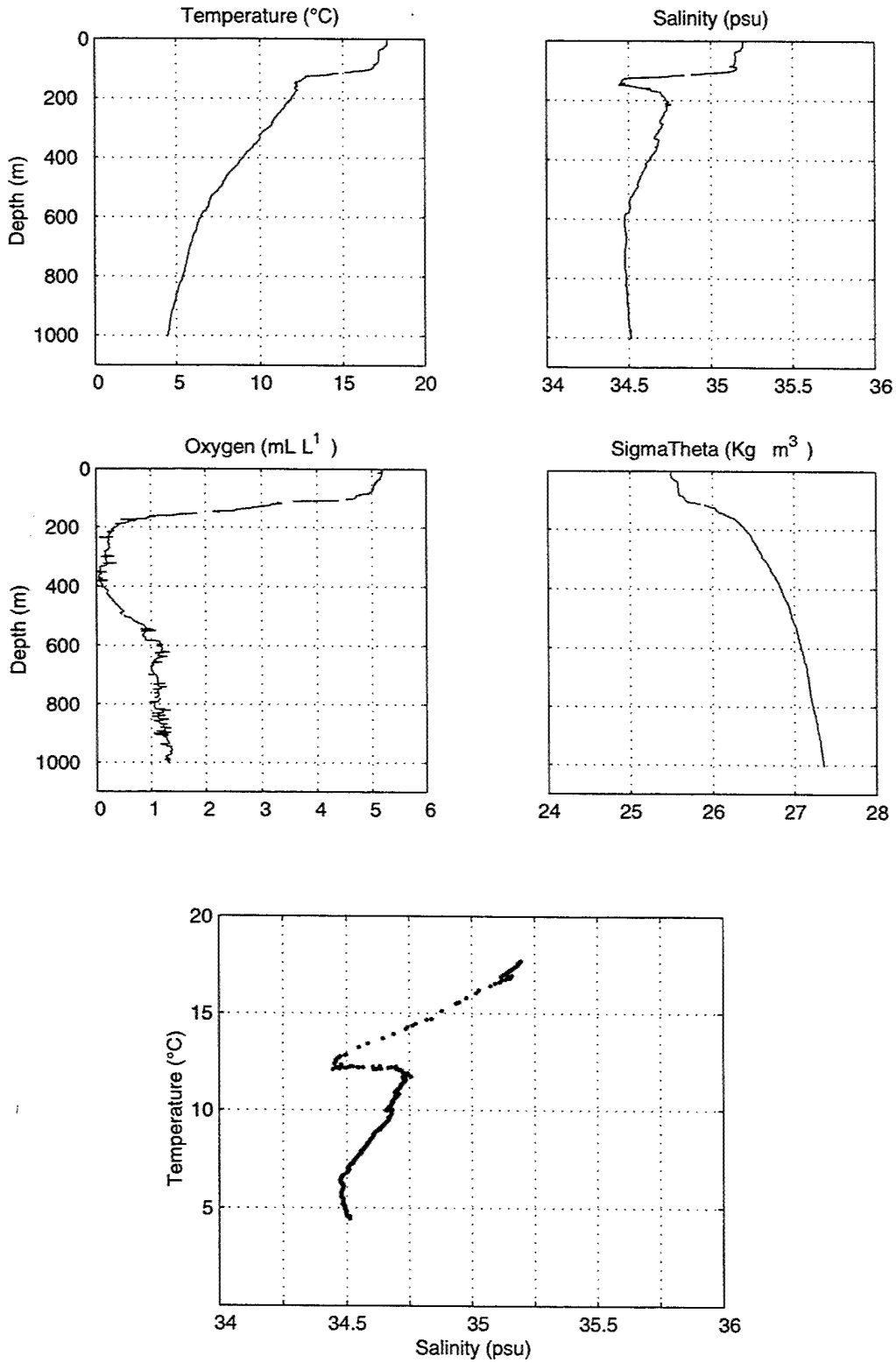
Figure 42. Stratus 12 CTD Cast.
