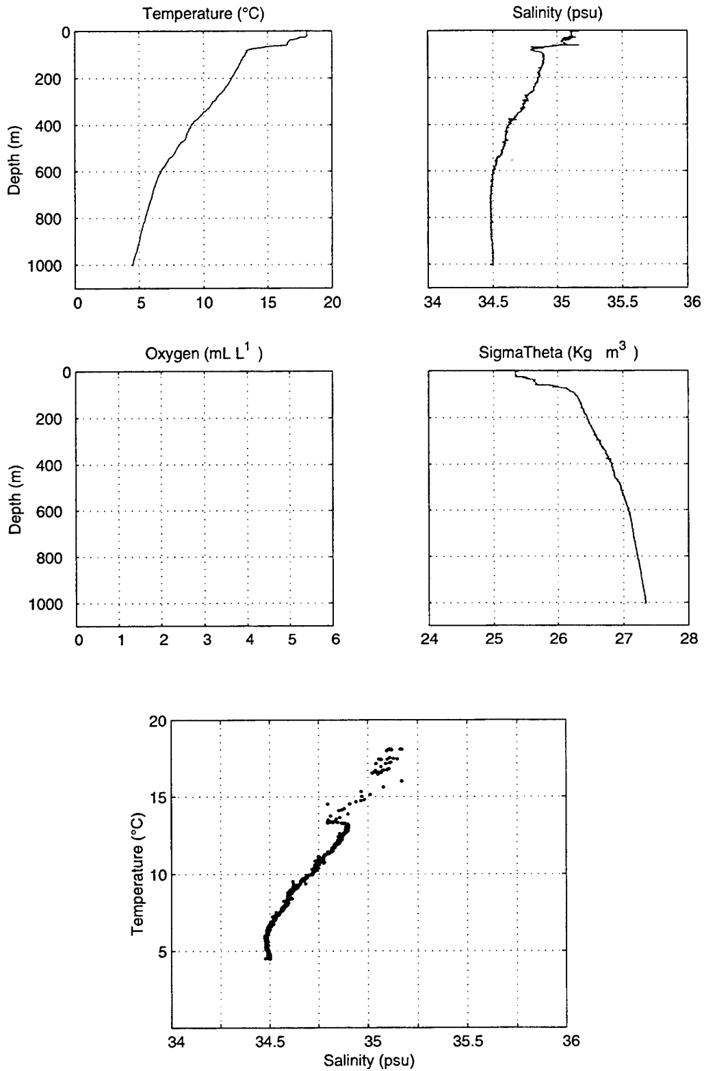
Figure 53. Stratus 17 CTD Cast, SBE 19 Data.
