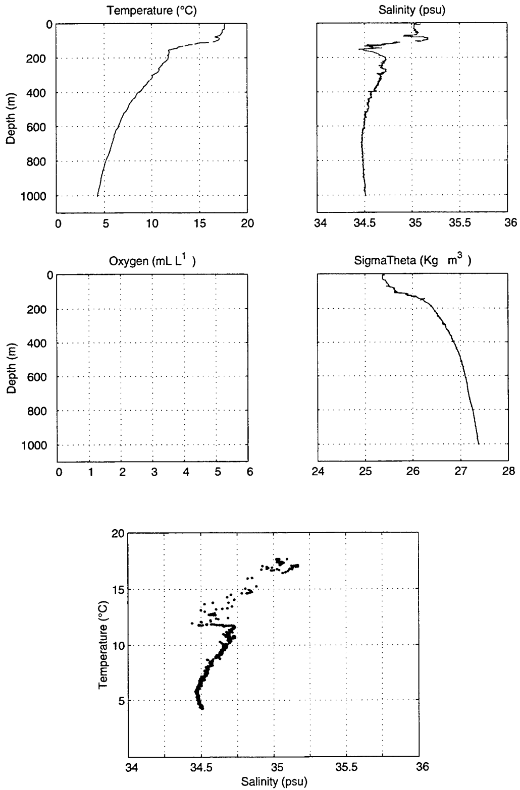
Figure 47. Stratus 14 CTD Cast, SBE 19 Data.
