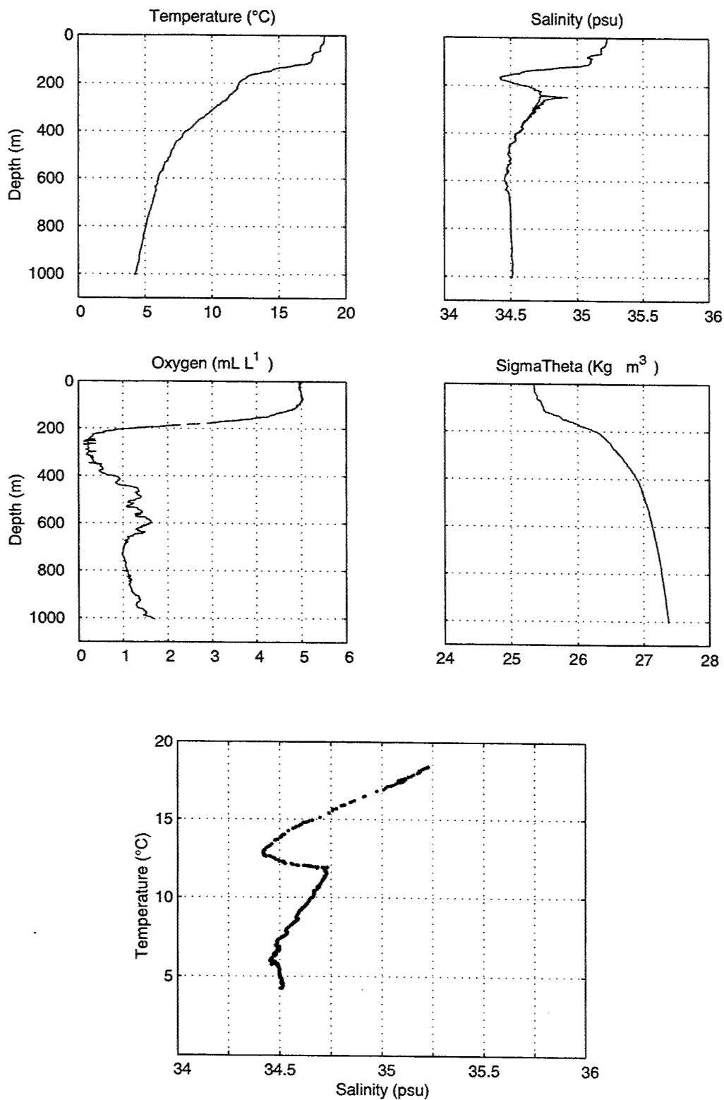
Figure 34. Stratus 05 CTD Cast.
