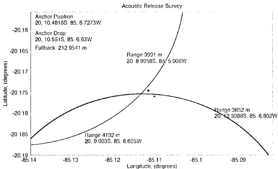
Figure 18. Acoustic Ranging to Locate Anchor.
