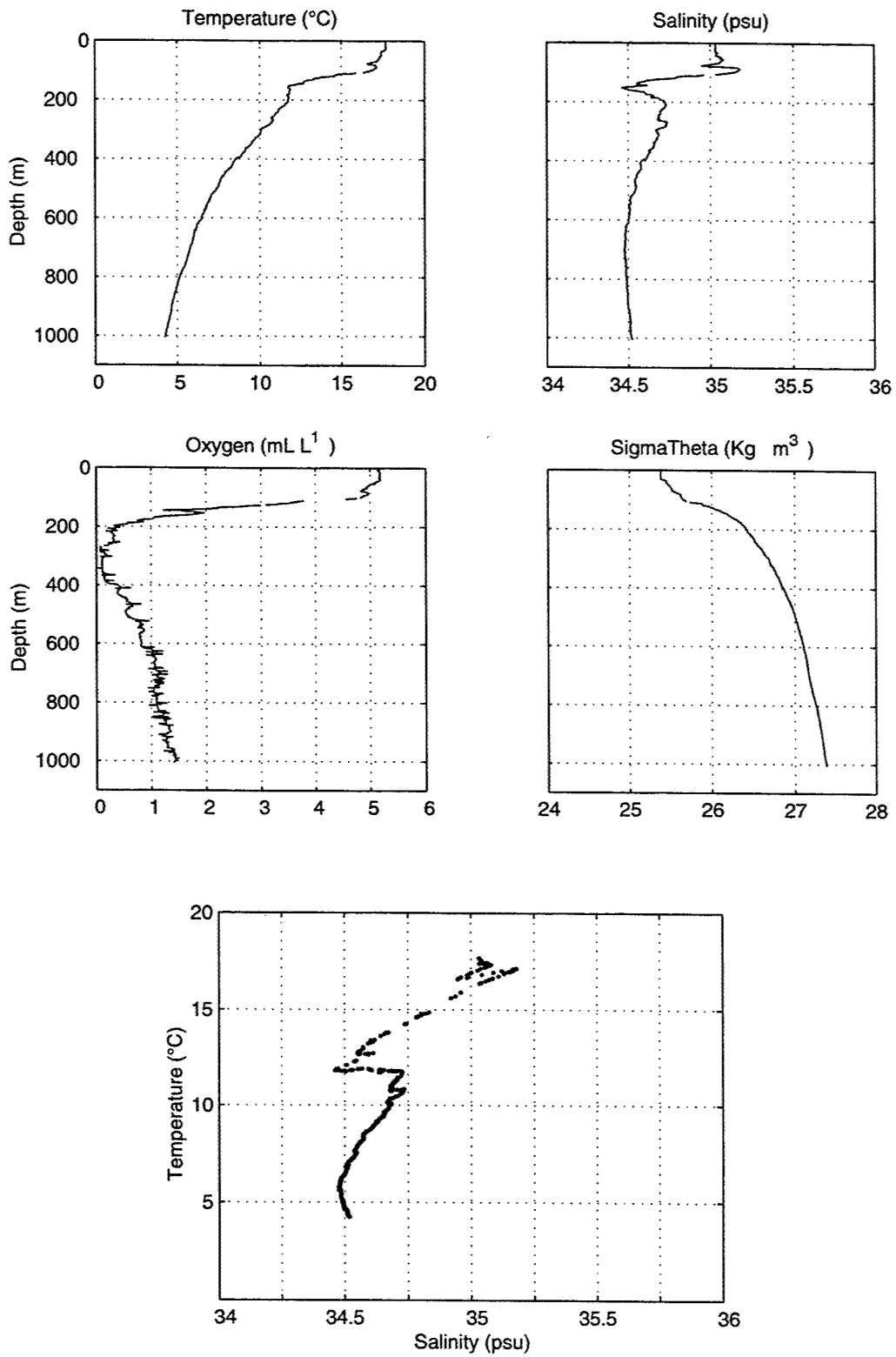
Figure 46. Stratus 14 CTD Cast.
