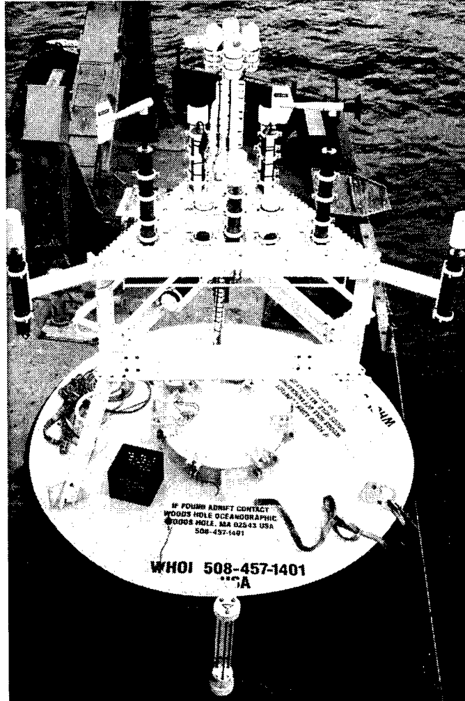
Figure 4. Surface instrumentation on the Stratus 3 mooring.
