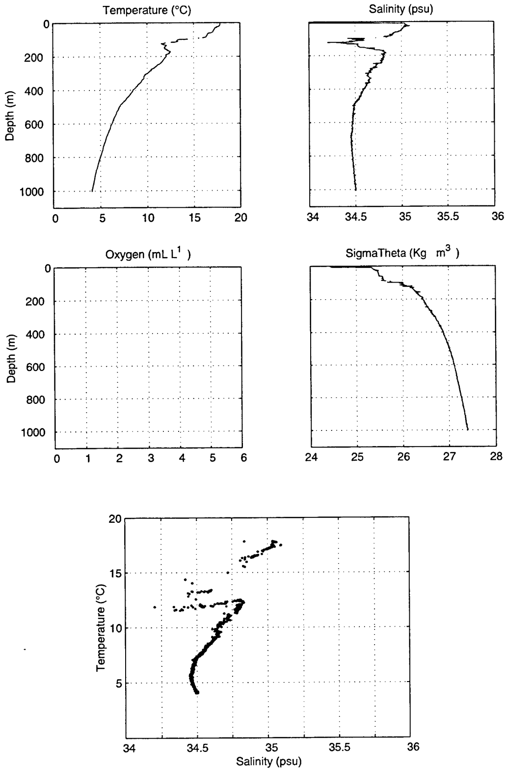
Figure 49. Stratus 15 CTD Cast, SBE 19 Data.
