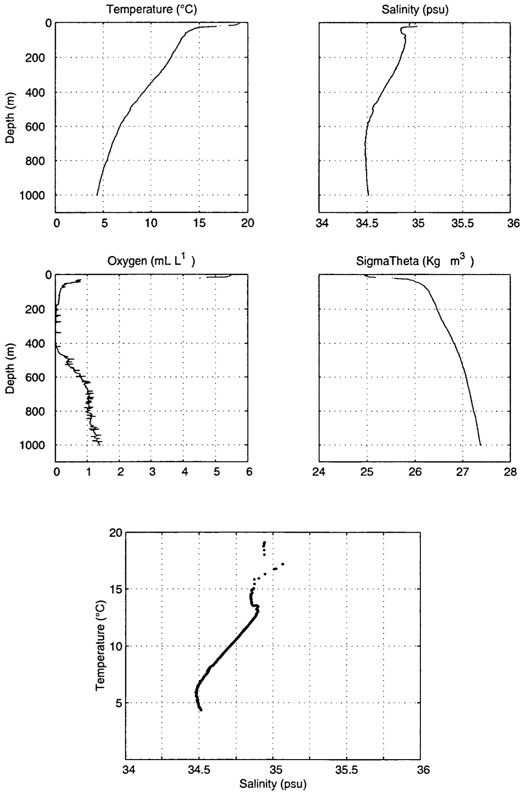
Figure 55. Stratus 19 CTD Cast.
