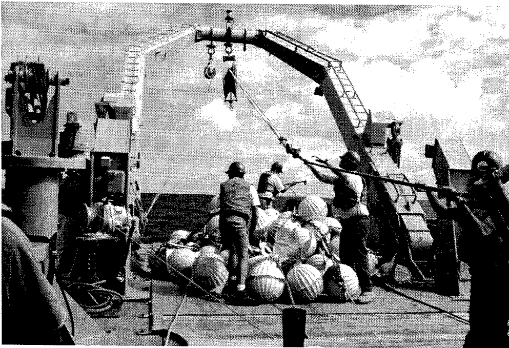
Figure 7. Retrieval of glass balls.
