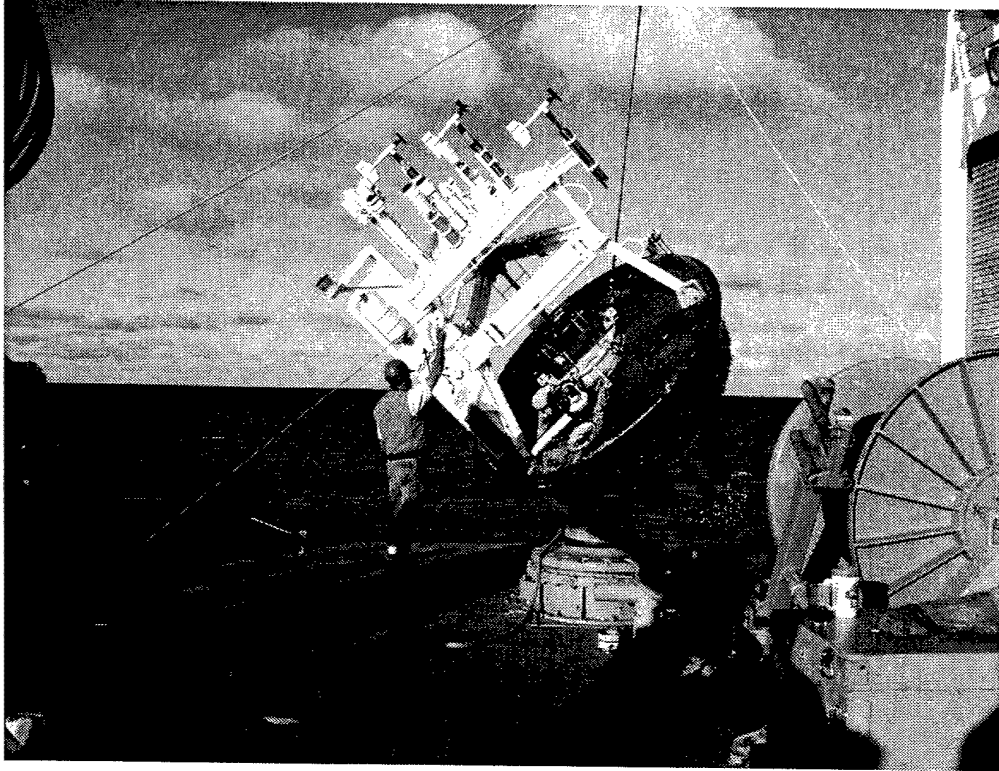
Figure 8. Retrieval of the Stratus 2 buoy.
