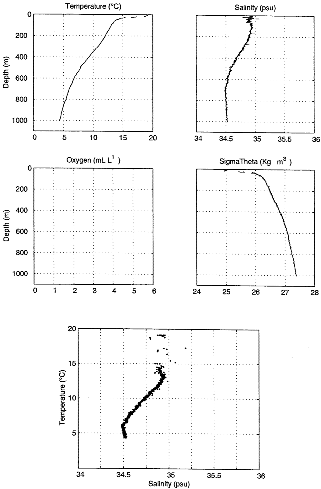
Figure 56. Stratus 19 CTD Cast, SBE 19 Data.
