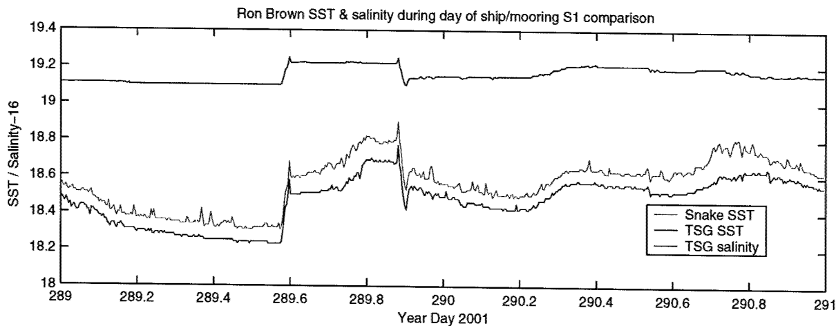
Figure 19: Ship data from the R/V Ron Brown during comparison for the Stratus 1 mooring.
