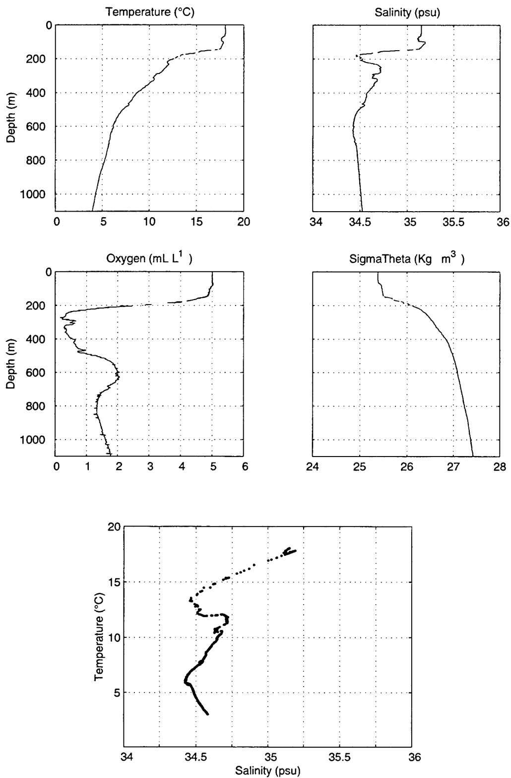
Figure 31. Stratus 02 CTD Cast.
