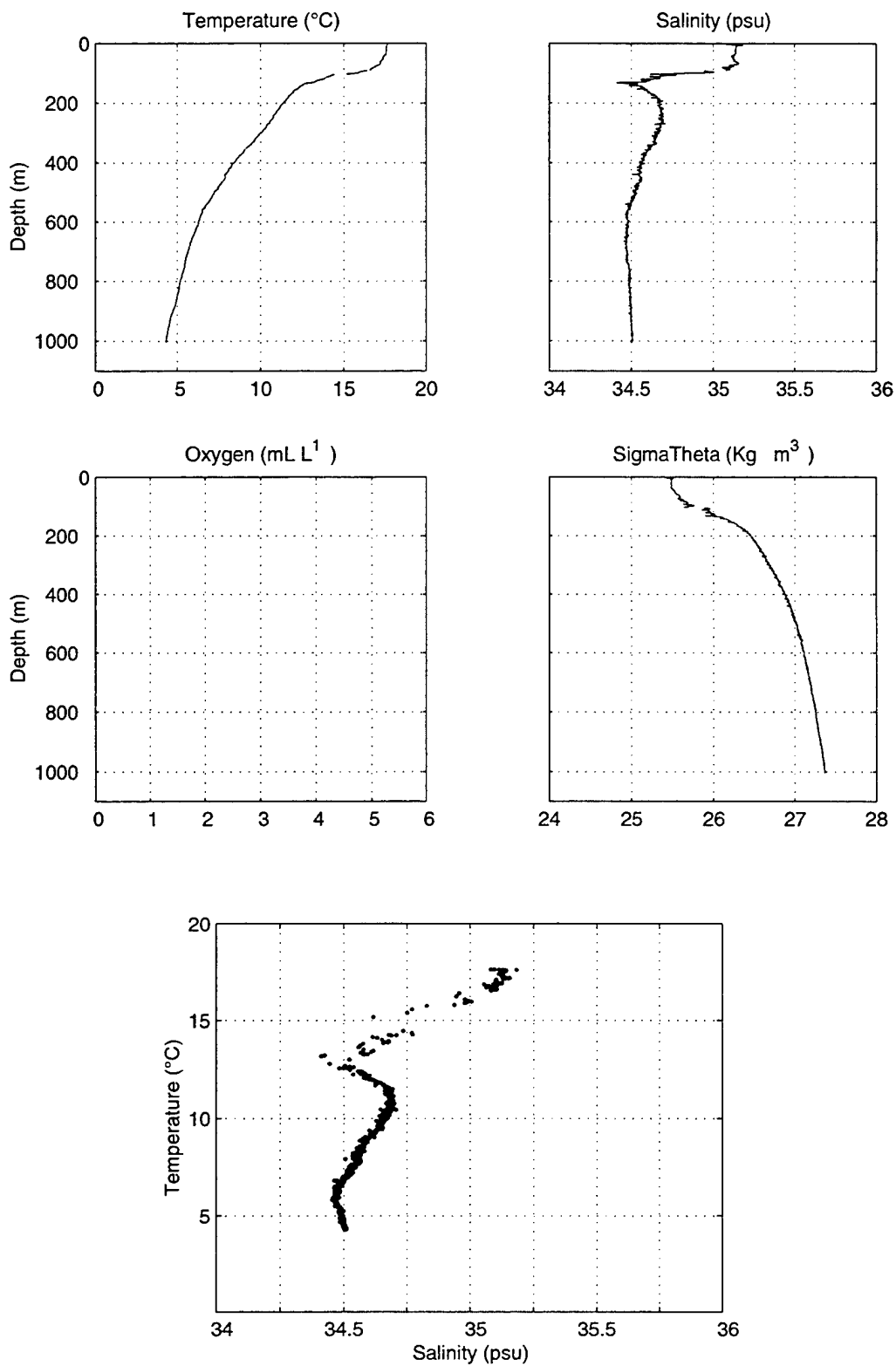
Figure 41. Stratus 11 CTD Cast, SBE 19 Data.
