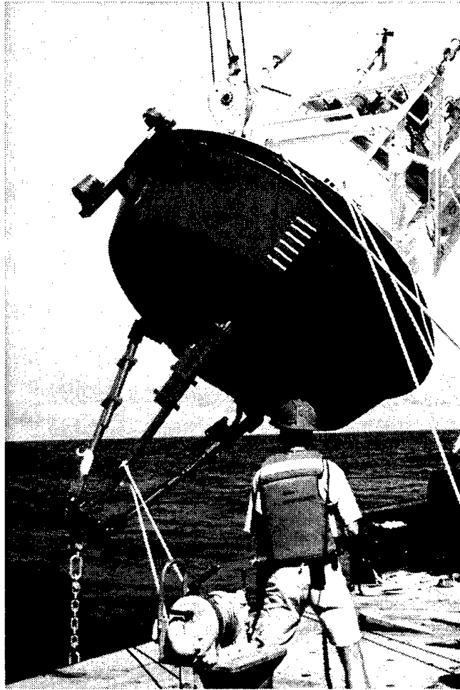
Figure 13: Slip lines rigged on the discus to maintain control during the lift.
