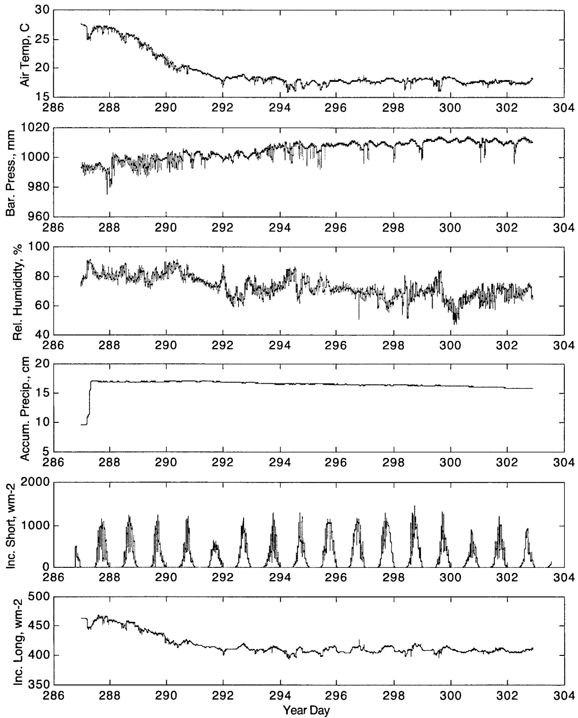
Figure 58. Shipboard IMET data collected during the Stratus 2002 cruise.
