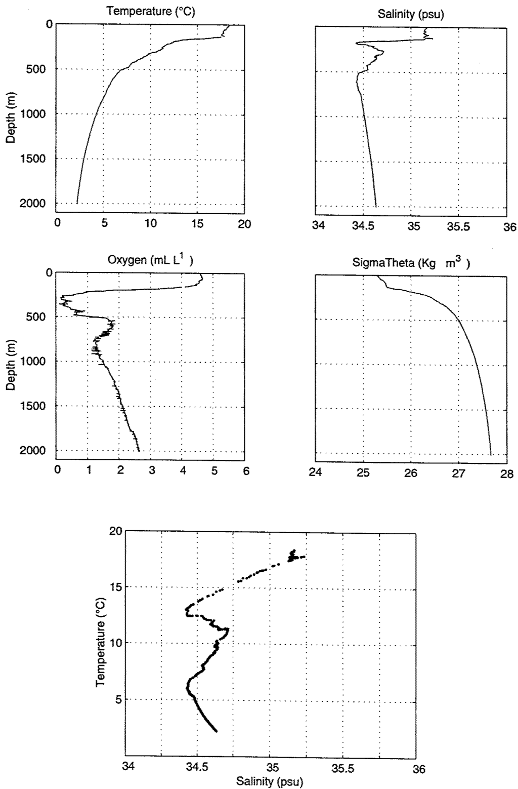
Figure 32. Stratus 03 CTD Cast.
