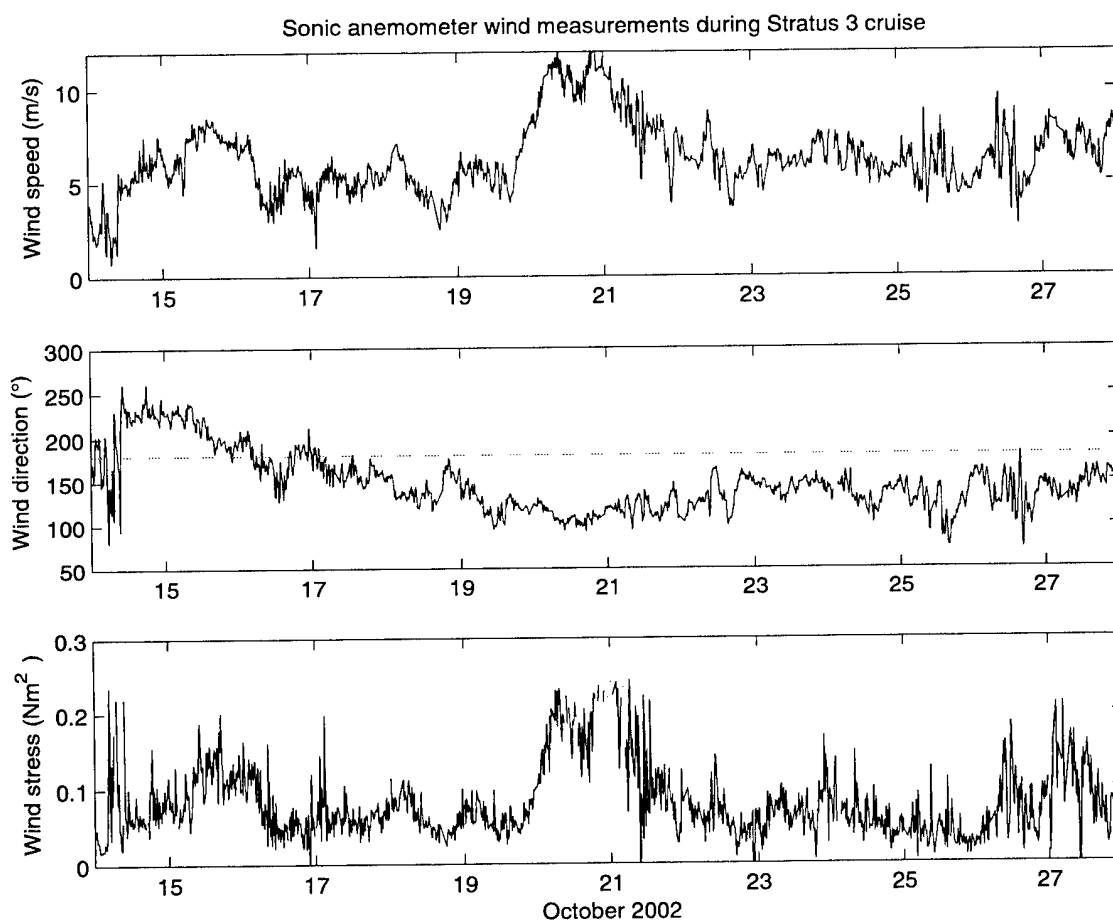
Figure 64: DCFs wind measurements during Stratus 3 cruise. a) wind speed (m/s), b) wind direction from (°), c) wind stress (Nm -2 ).
