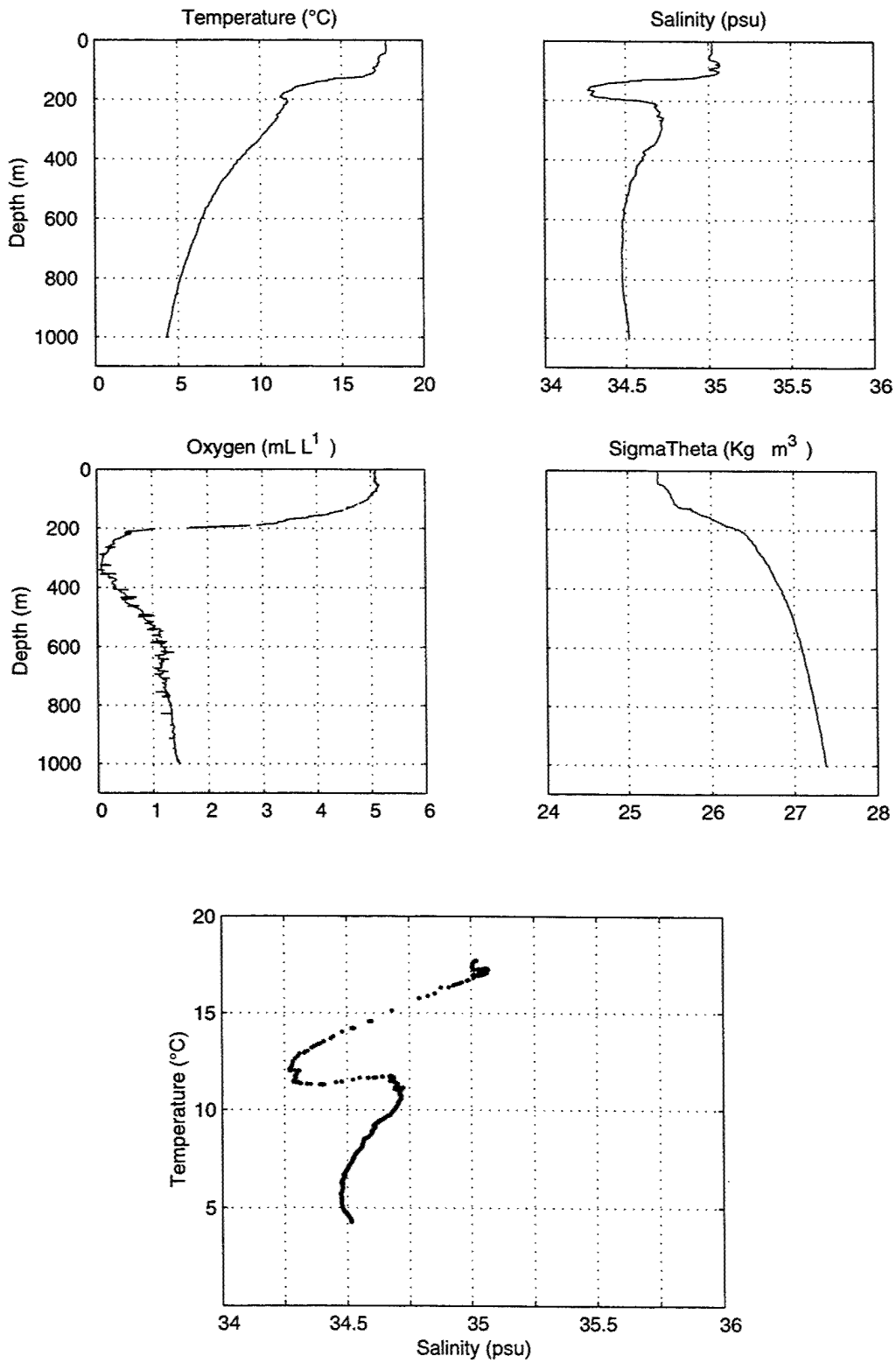
Figure 44. Stratus 13 CTD Cast.
