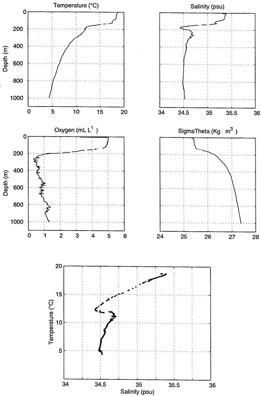
Figure 36. Stratus 07 CTD Cast.
