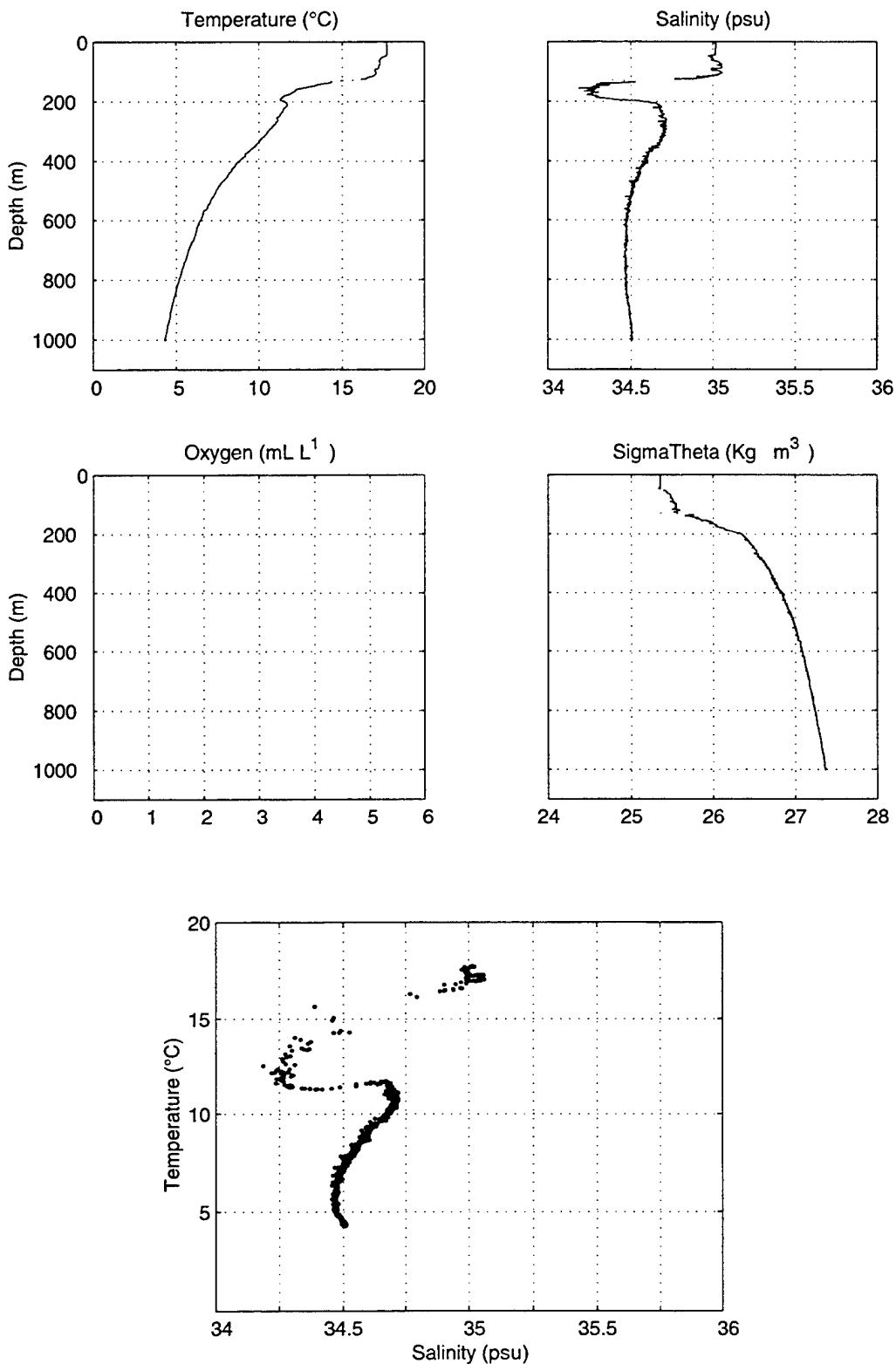
Figure 45. Stratus 13 CTD Cast, SBE 19 Data.
