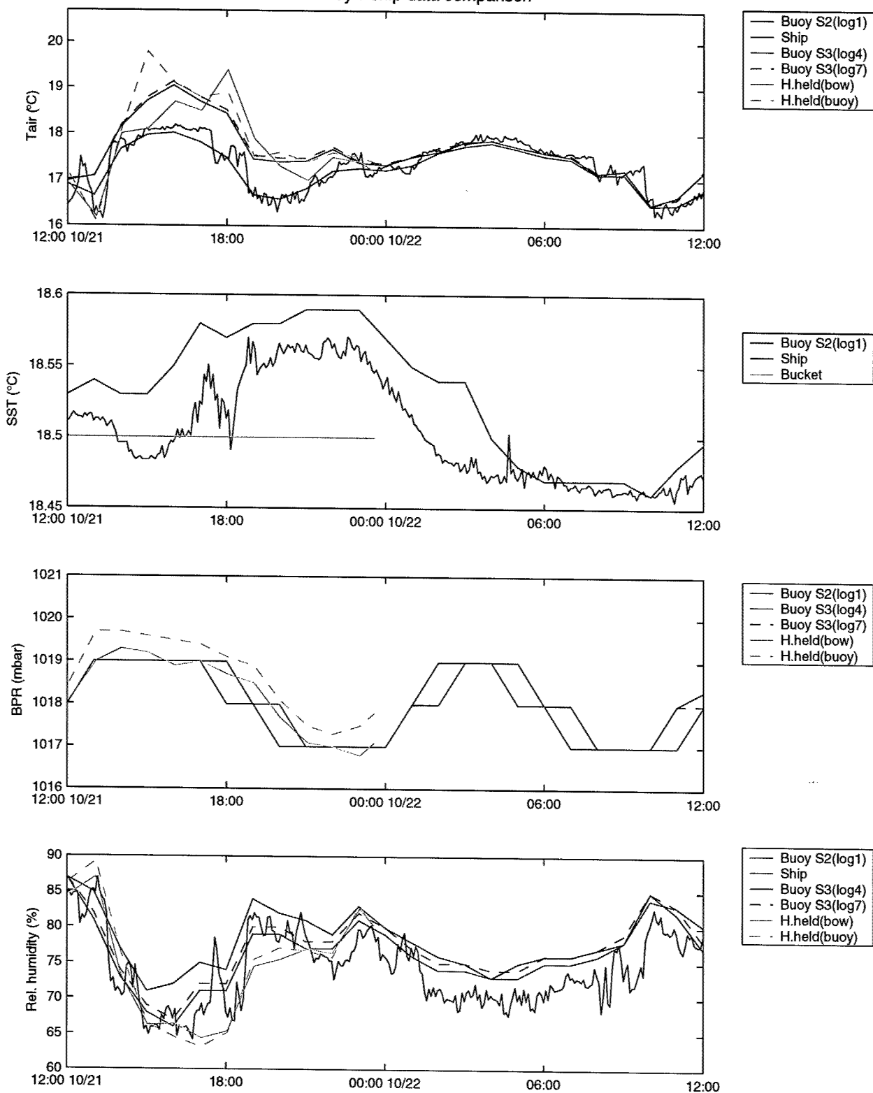
Figure 22: Stratus 2 buoy data comparison (times are given in UTC).
