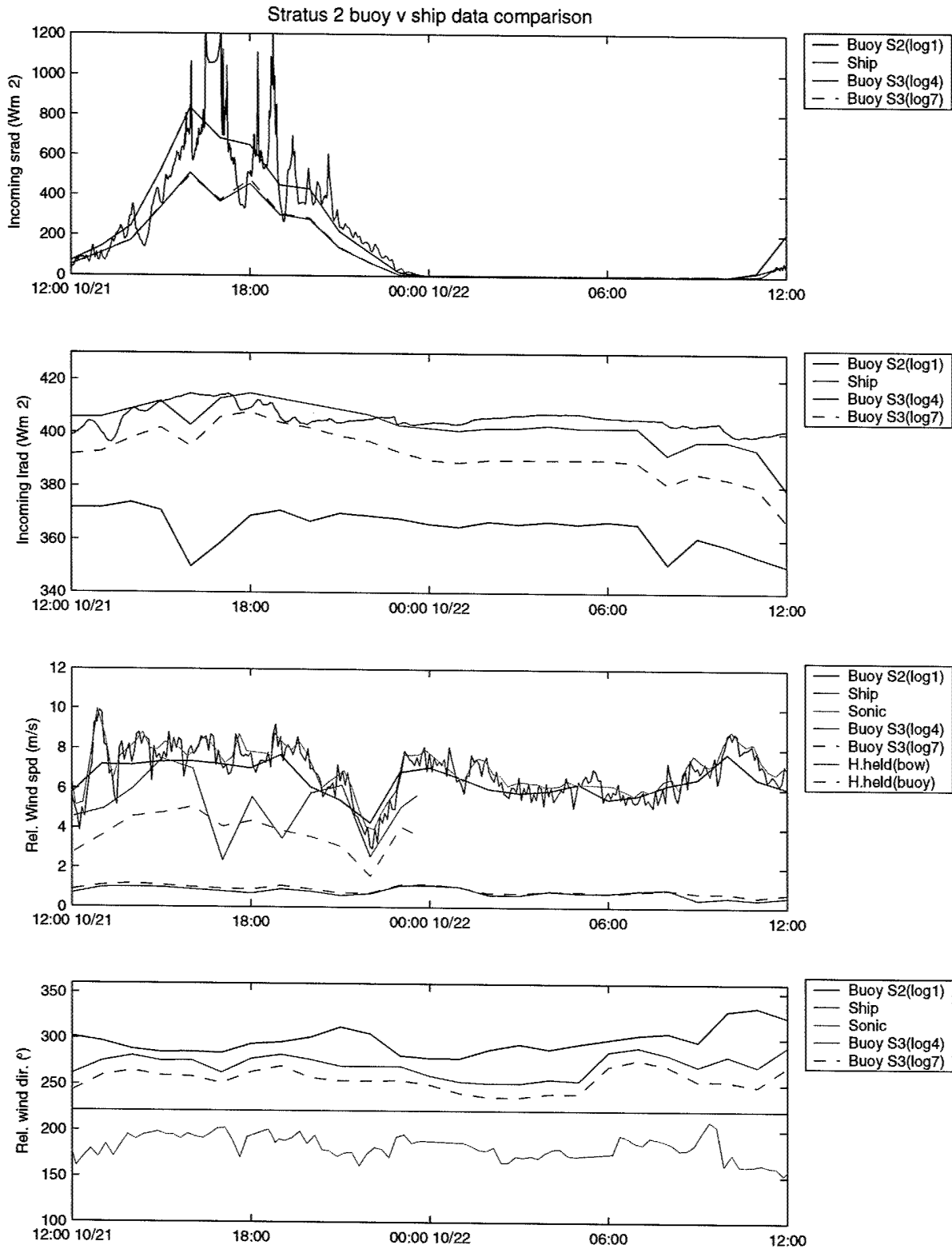
Figure 23: Stratus 2 buoy data comparison (times are given in UTC).
