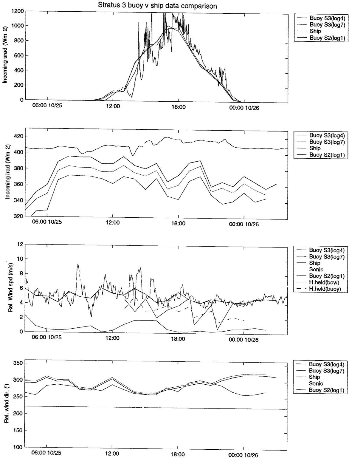
Figure 25: Stratus 3 buoy data comparison.
