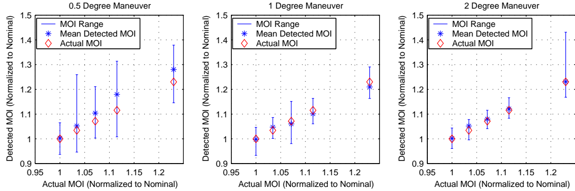
Figure 4.12 Data Overlap and Accuracy, Method Three
