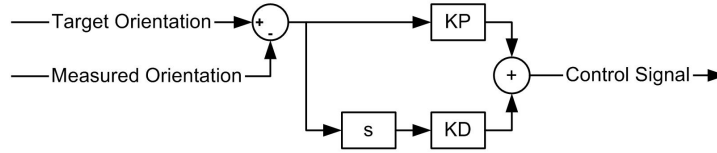
Figure 2.4 Satellite Proportional Plus Derivative Controller
