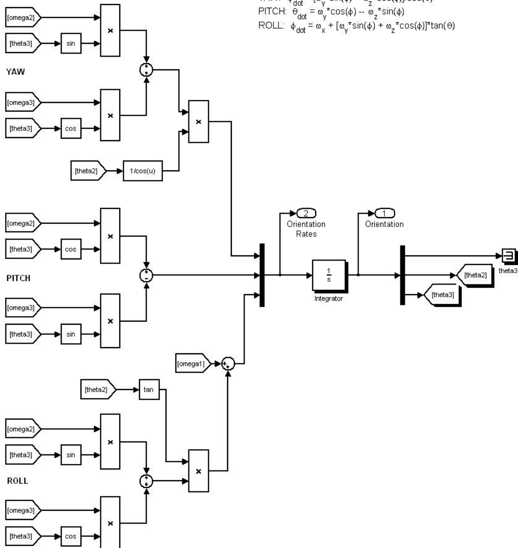
Figure E.12 Euler 3-2-1 Kinematics, Level 2 Submodel
