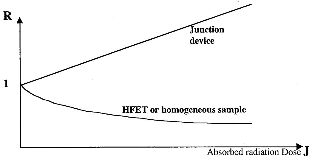
Fig. 1. Dependence of the Noise Modification Ratio R on the absorbed radiation dose J
