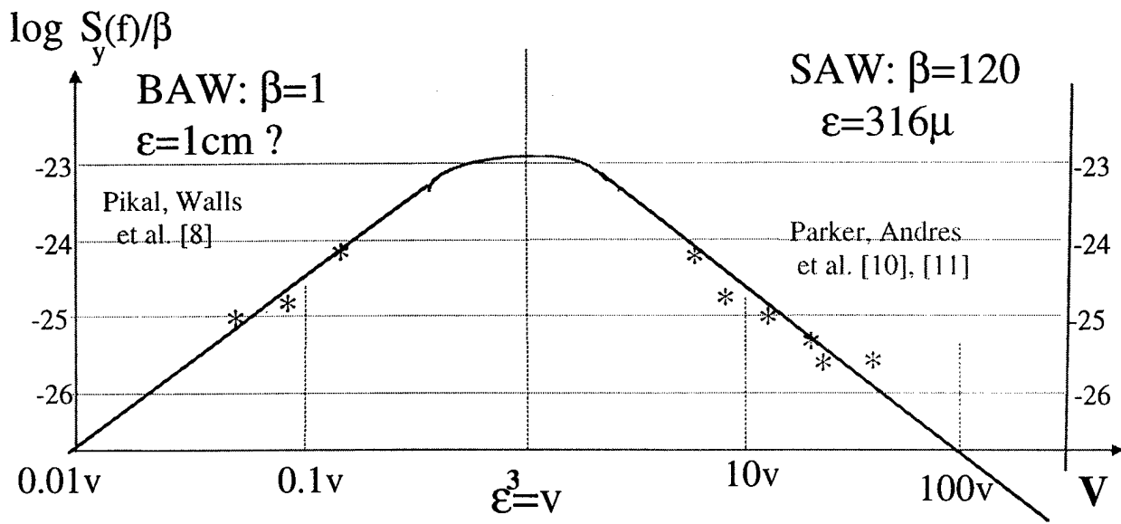
Fig. 4: Quantum 1/f Noise in BAW & SAW Resonators Yields Bio/Chem Sensitivity Limit
