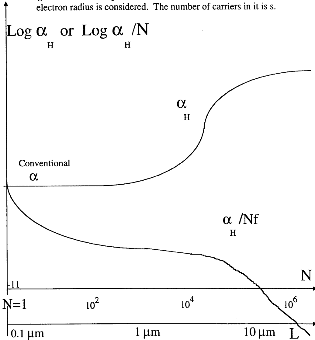
Fig. 6: The quantum 1/f parameter \alpha_H and the resulting spectral density S_j = \alpha_H/Nf as a function of the number of carriers in the sample N or of the cross section size L .
