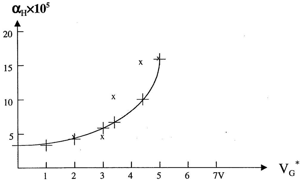
Fig. 3: Comparison of the quantum 1/f first-principles results + with the experimental results x of A. Balandin et al., on "Flicker Noise in GaN/AlGaN Doped Channel Heterostructure FETs", IEEE-Electron Device Letters 19 , 475-477 (1998).
