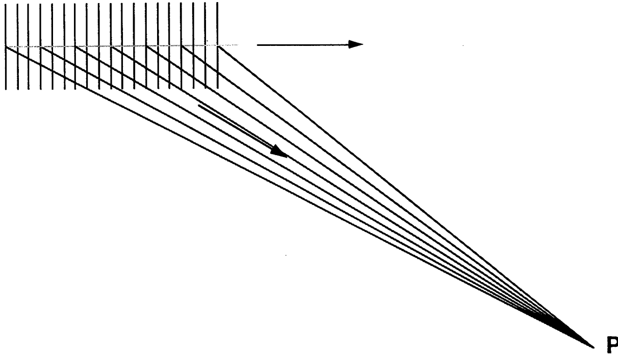
Fig. 2: An antenna array generates a coherent superposition of beams from each antenna in the array, with a resulting angular width given by the diffraction limit \delta_o\theta = \lambda/2N\text{acos}\theta in the absence of phase noise.
