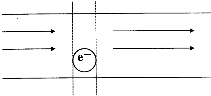
Fig. 5: To define the parameter s , a slice as thick as the classical electron radius is considered. The number of carriers in it is s .
