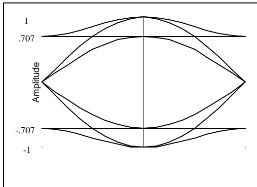
Figure 1-10. FQPSK-B wavelets.
