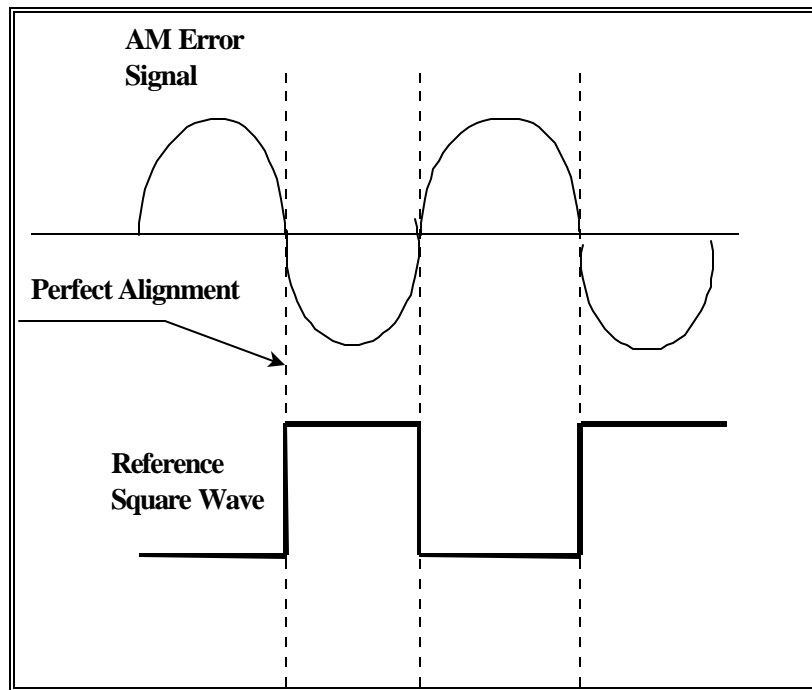
Figure 3-6. AM modulation error signal.
