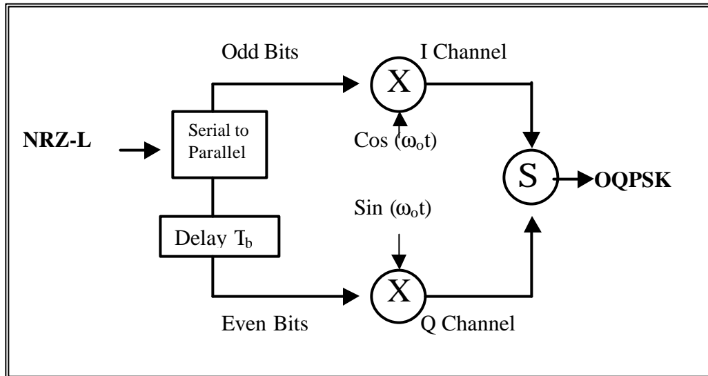
Figure 1-9. OQPSK block diagram.
