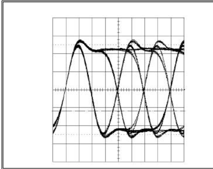
Figure 1-13. 5-Mb/s PCM eye pattern.
