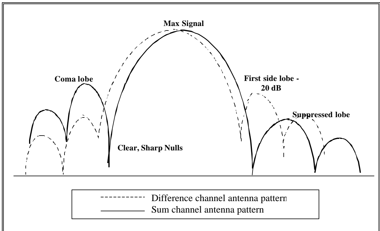
Figure 3-5. Typical antenna pattern for conical scan feed assembly units.
