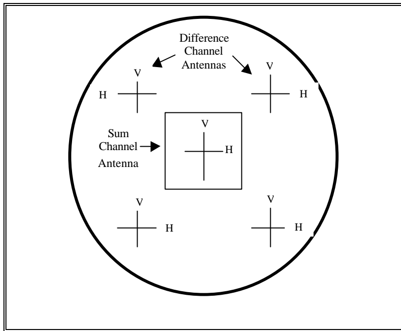
Figure 3-2. Single channel monopulse dipole antennas.
