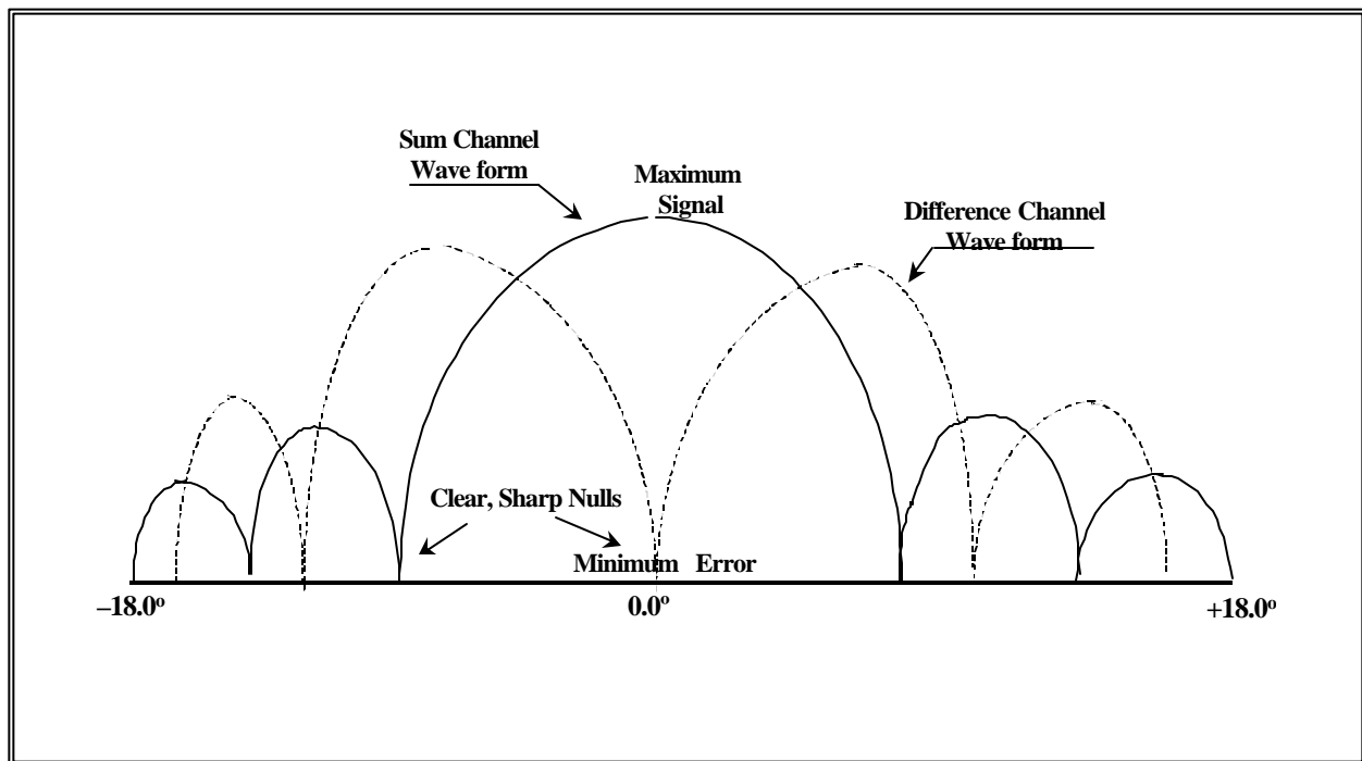
Figure 3-4. Typical sum channel and difference channel patterns (unscaled).
