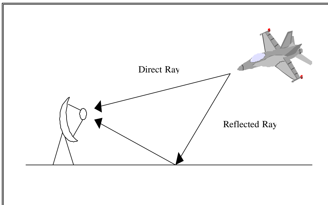
Figure 2-1. Multipath signal propagation.
