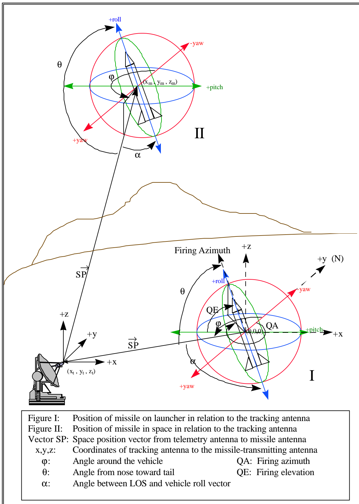
Figure 3-9. Pictorial of parameters needed for measurement of transmitted gain.
