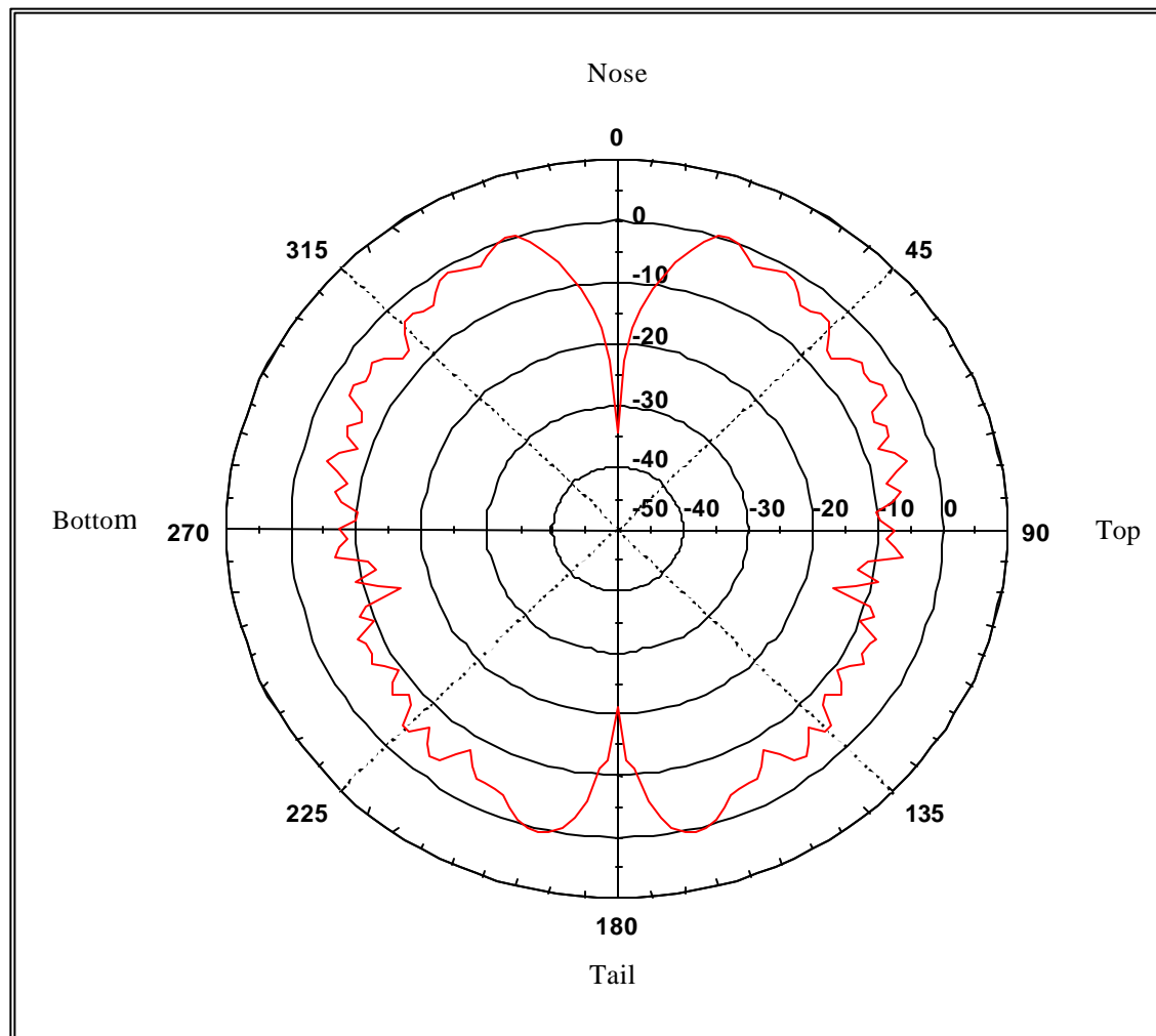
Figure 1-15. Antenna pattern for the pitch plane.
