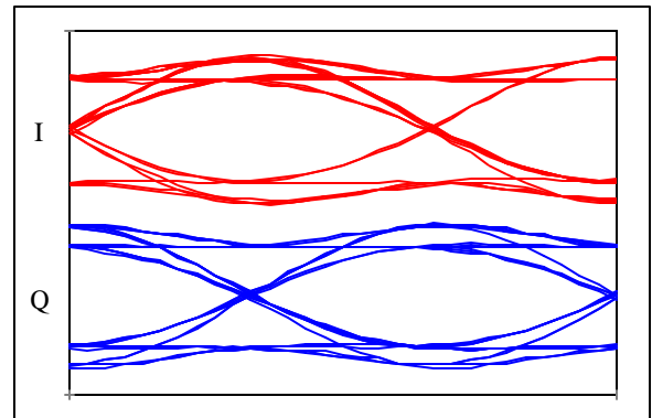
Figure 1-11. FQPSK-B:I & Q signals.
