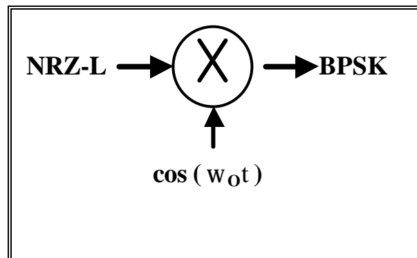
Figure 1-7. BPSK block diagram.
