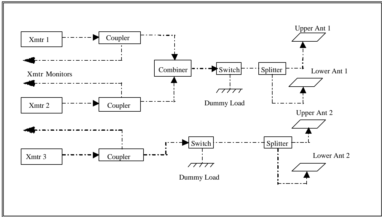
Figure 1-6. Configuration 6: Complex telemetry transmit system.
