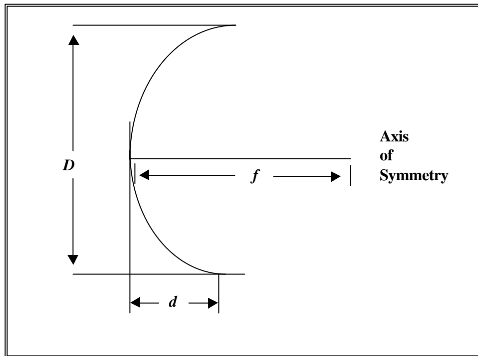
Figure 3-1. Measurements used to calculate f/D ratio.
