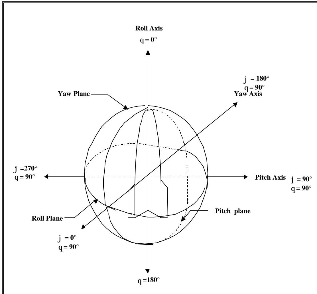
Figure 1-14. Vehicle coordinate system. 7
