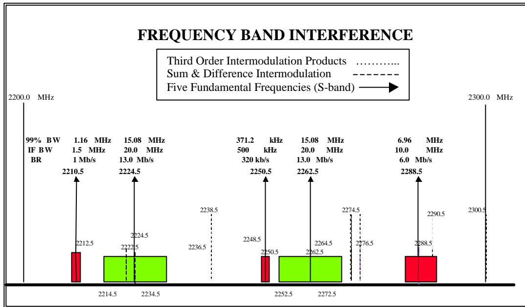
Figure 3-12. Frequency band interference.
