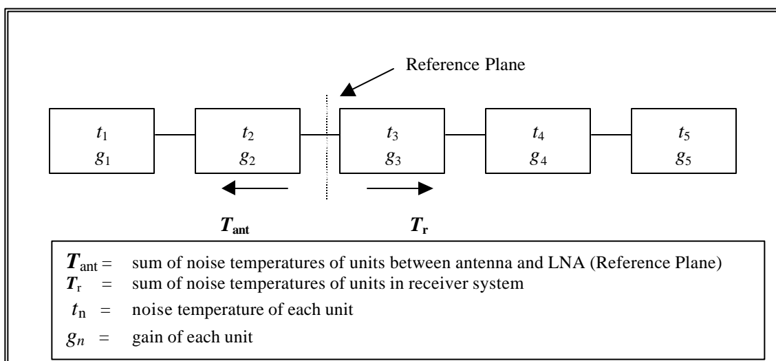
Figure 3-10. Block diagram of RF units in the RF assembly.
