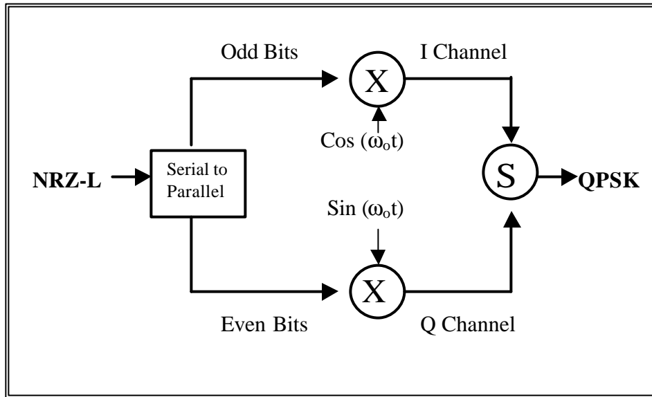
Figure 1-8. QPSK block diagram.
