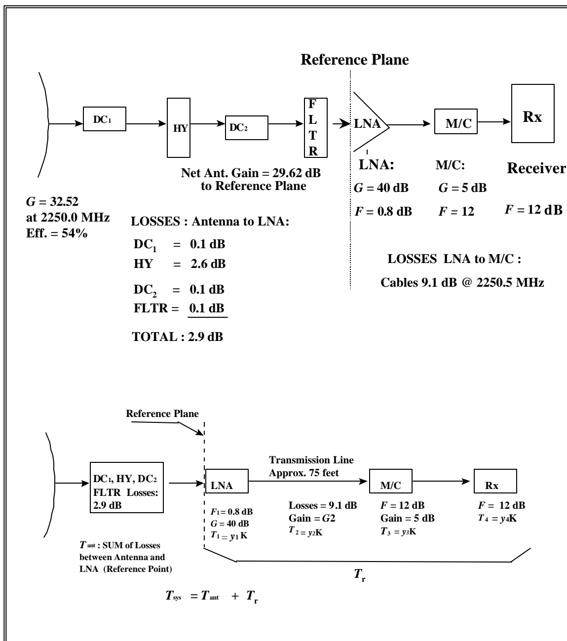
Figure 3-11. Block diagram of a sample RF subsystem.
