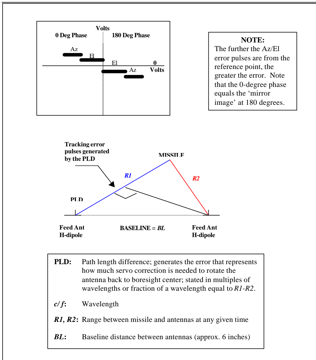
Figure 3-3. Tracking errors generated by dipole antennas.
