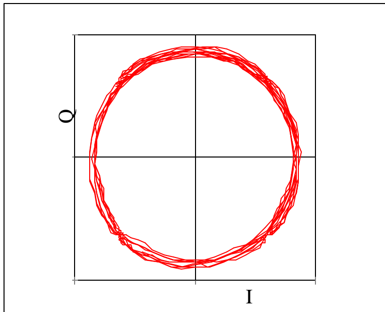
Figure 1-12. FQPSK vector diagram.
