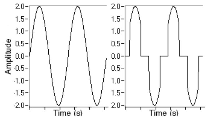
Fig. 2. Illustration of the process of center clipping. K=0.6 , which gives a threshold of 1.2.
