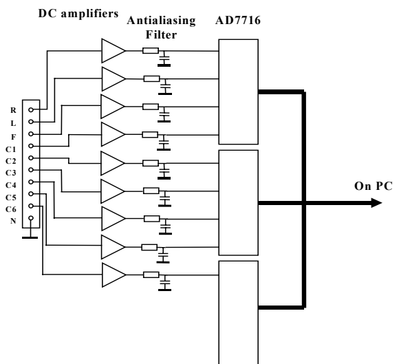
Fig. 2. 12-channel ECG on AD7716
