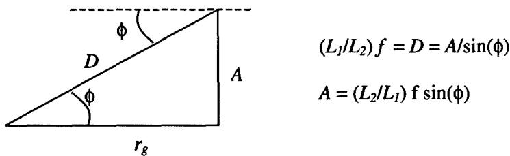
Figure 23. Geometry for aerial photography.
