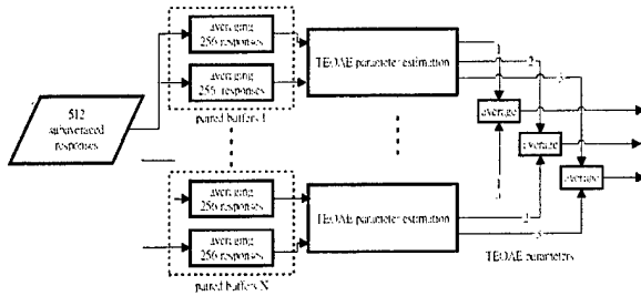
Fig. 1 Block diagram of the multi-average method
