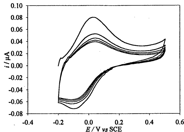
Figure 6: Electrochemical behaviour of a copolymer of aniline and anthranilic acid (1:1 ratio) in 0.1 M citrate/phosphate buffer pH 7, \nu = 50 \text{ mV s}^{-1} (electropolymerisation by CV at 60 °C, Q_{\text{growth}} = 51.34 \text{ mC} ).
