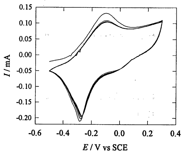
Figure 10: Electrochemical behaviour of a PANi-Nafion ® composite film in 0.1 M citrate/phosphate buffer pH = 7 ( Q_{\text{growth}} = 150 \text{ mC} , area = 0.38 \text{ cm}^2 ), \nu = 50 \text{ mV s}^{-1} .
