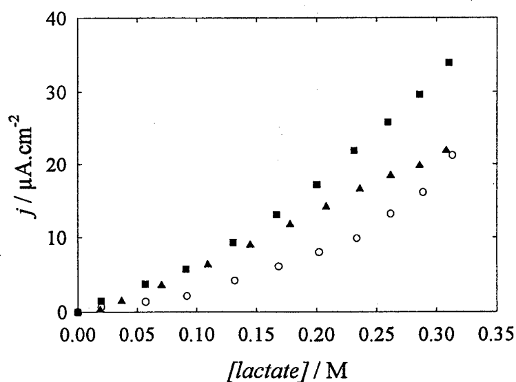
Figure 42: Catalytic currents for enzymatically produced NADH, recorded at 0.05 V vs SCE at an enzyme/PANi-PAA modified electrode (electropolymerisation by cyclic voltammetry, deposition charge \sim 200 mC, geometric area = 0.38 cm 2 , film thickness \sim 11 \mu\text{m} (measured by SEM), PANi-PAA film soaked in an enzyme solution ( 0.43 mg ml -1 ) for 2 hours at 4°C) rotated at 9 Hz in 1.0 M Tris-HCl pH 7.1 at 35 °C, containing 30 mM NAD + , under argon. O, ■ and ▲ represent WT-LDH, LDH-CHis and LDH-NHis respectively.
