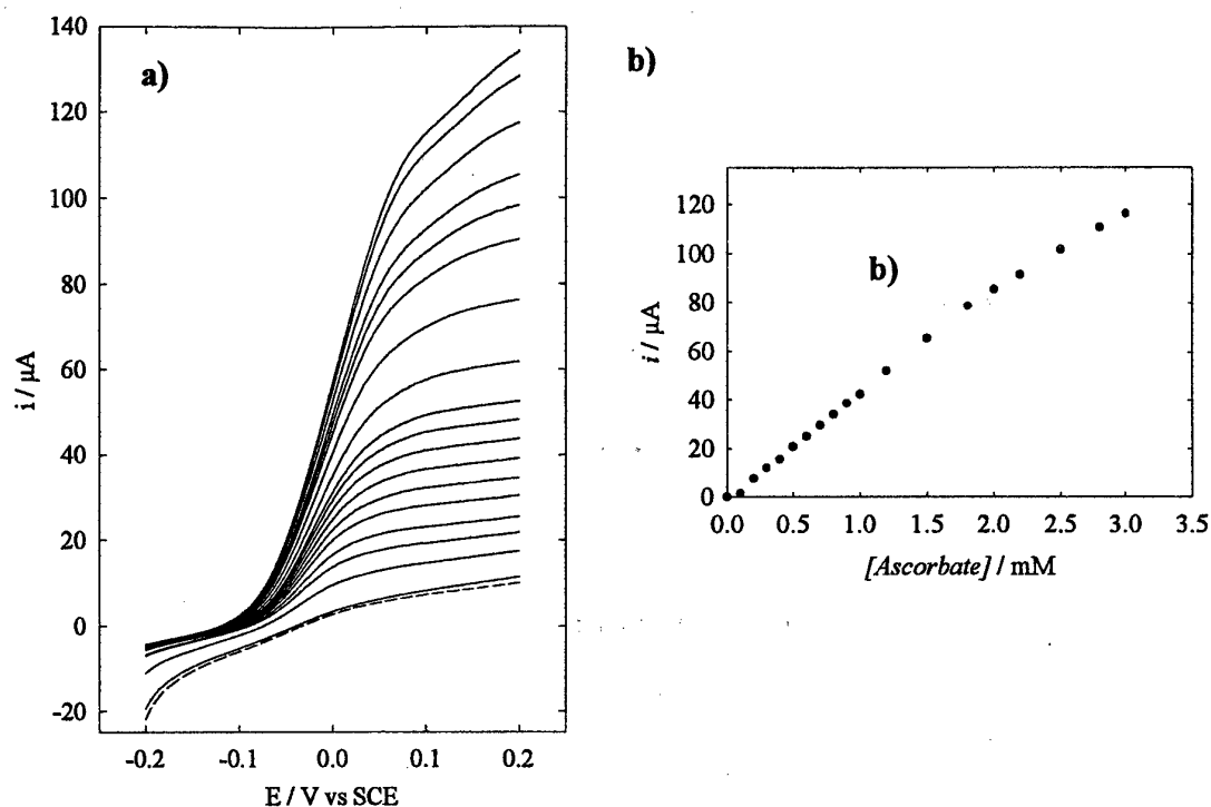
Figure 13: a) Ascorbate oxidation at a PANi-Nafion modified electrode, in 0.1M citrate/phosphate buffer pH 7.0, 25 °C, under argon, \omega = 5 Hz, potential swept from -0.2 to +0.2 V vs SCE at 2 \text{ mV s}^{-1} b) Plot of the plateau current versus the concentration of ascorbate in the bulk of the solution.
