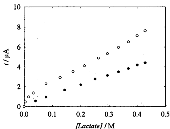
Figure 38: NADH detection at a LDH-CHis-PANi-PAA modified electrode, LDH-CHis tagged to PANi-PAA or free in solution. E_{\text{applied}} = 50 \text{ mV} , W = 9 \text{ Hz} , in 1 M L-lysine-acetic acid + 10 mM of \text{CaCl}_2 , pH 7.0 at 35^\circ \text{C} in presence of 17.7 mM of \text{NAD}^+ . (●): LDH-CHis immobilized on PANi-PAA- \text{Ni}^{2+} ; (○): 30 mM free LDH-CHis.
