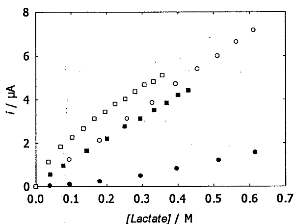
Figure 39: Currents recorded at +0.05 V vs SCE at poly(aniline)-poly(acrylate) and Ni 2+ doped poly(aniline)-poly(acrylate) coated glassy carbon electrodes (deposition charge ~ 280 mC cm -2 , electrode area = 0.38 cm 2 , thickness ~ 5.5 μm) rotated at 9 Hz in 1 M lysine, 10 mM CaCl 2 , 30 mM NAD + at pH 7 and 35° C as a function of the lactate concentration. Data are corrected for background in each case. ● and ■ represent LDH-WT and LDH-CHis respectively, on Ni 2+ doped PANi-PAA film and ○ and □ represent LDH-WT and LDH-CHis respectively, on a standard PANi-PAA film.
