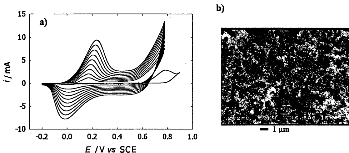
Figure 15: a) Electropolymerisation by cyclic voltammetry of aniline on a glassy carbon disc electrode (area = 0.38 cm 2 ) in 2.7 M HCl in the presence of 15% poly(acrylic acid). During the first cycle the potential is swept from -0.2 to 0.9 V vs SCE at 50 mV s -1 and then for all the subsequent cycles it is swept from -0.2 to 0.78 V. b) Scanning Electron Microscope image of a poly(aniline)-poly(acrylic) composite film deposited on a glassy carbon electrode (scale bar 1 μm).
