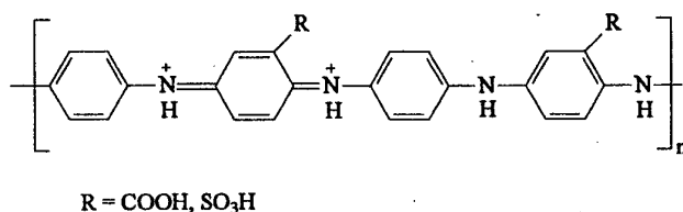
Figure 5: Self-doped poly(aniline).
