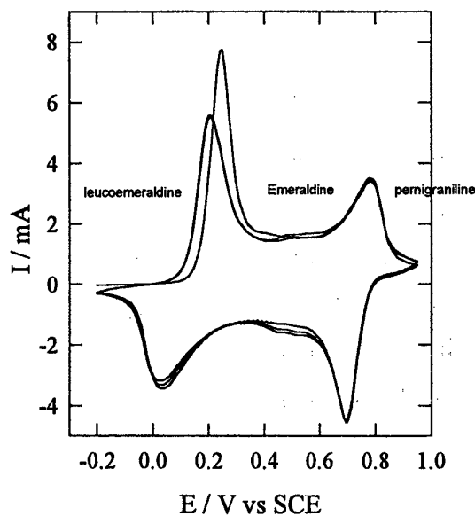
Figure 9: Electrochemical behaviour of a PANi-Nafion ® composite film in 1.0 M HCl ( Q_{\text{growth}} = 150 \text{ mC} , \text{rea} = 0.38 \text{ cm}^2 , \nu = 50 \text{ mV.s}^{-1} ).
