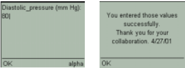
Fig. 5.Application screenshots.
