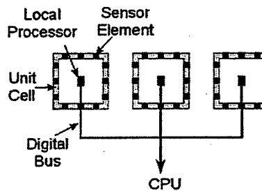
(b) Arrangement of continuous sensor & local processor
