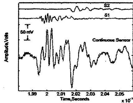
Figure 18: Acoustic Emission waveforms
