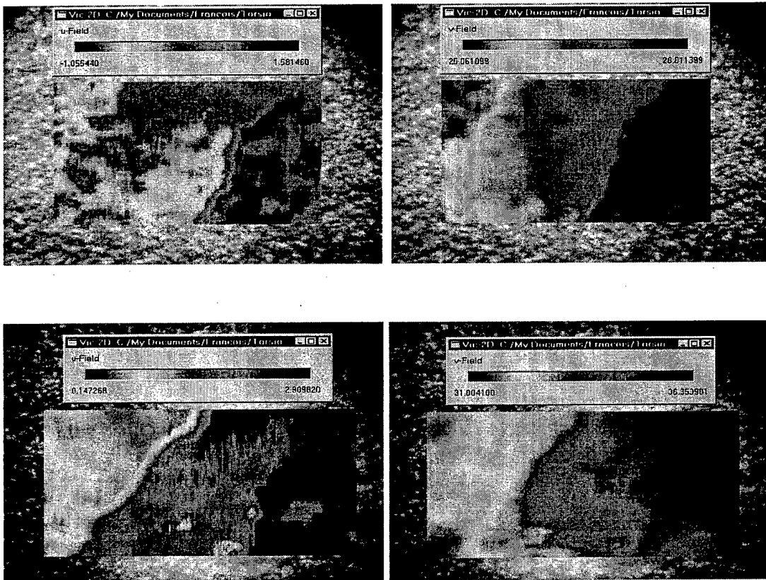
Figure 17 : Contours of horizontal and vertical displacement fields as obtained by image correlation of speckle patterns on sample surface.
