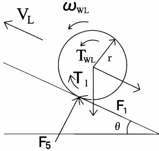
Fig.2 Left wheel free body on a slope
