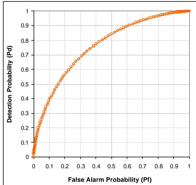
Figure 63. ROC Curve.
