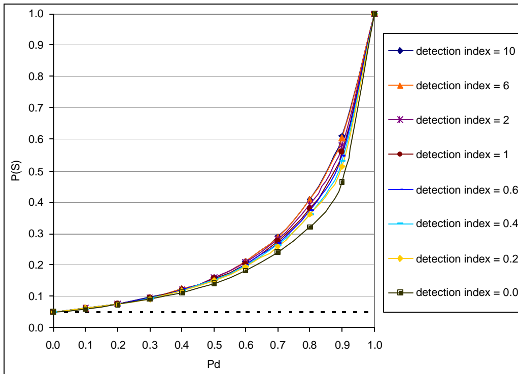
Figure 61. Probability of Safe Minefield Transit by Using the MOAM Model, L=6 , w=0.5 , I_O=0.6 , I_M=1.0 .
