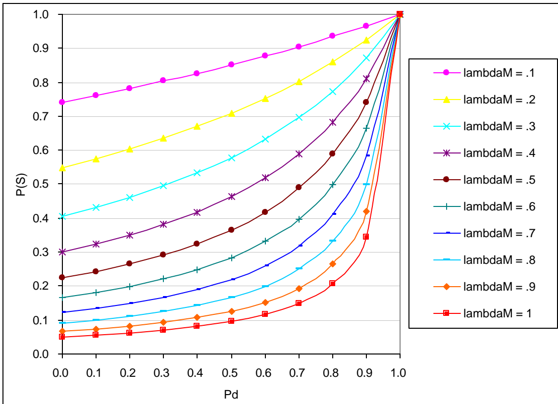
Figure 22. Probability of Safe Minefield Transit, L=6 , w=0.5 , I_o = 0.0 .
