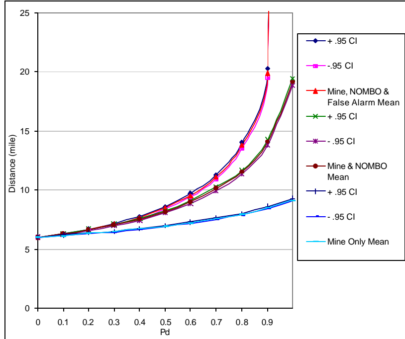
Figure 42. Conditional Mean Distance Traveled Given Successful Transit and 95% CI.
