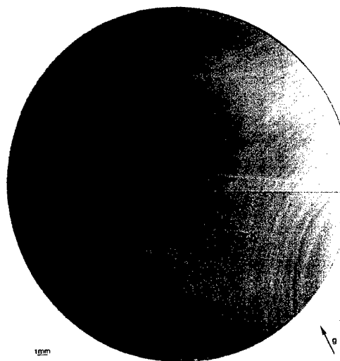
(b) A Y-cut LGT wafer g = \bar{1}100
