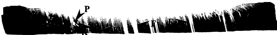
Figure 6. Enlargement of a topograph showing striation, K, precipitates, P, and facets, F. In this case, striations are clearly shown in the facets
