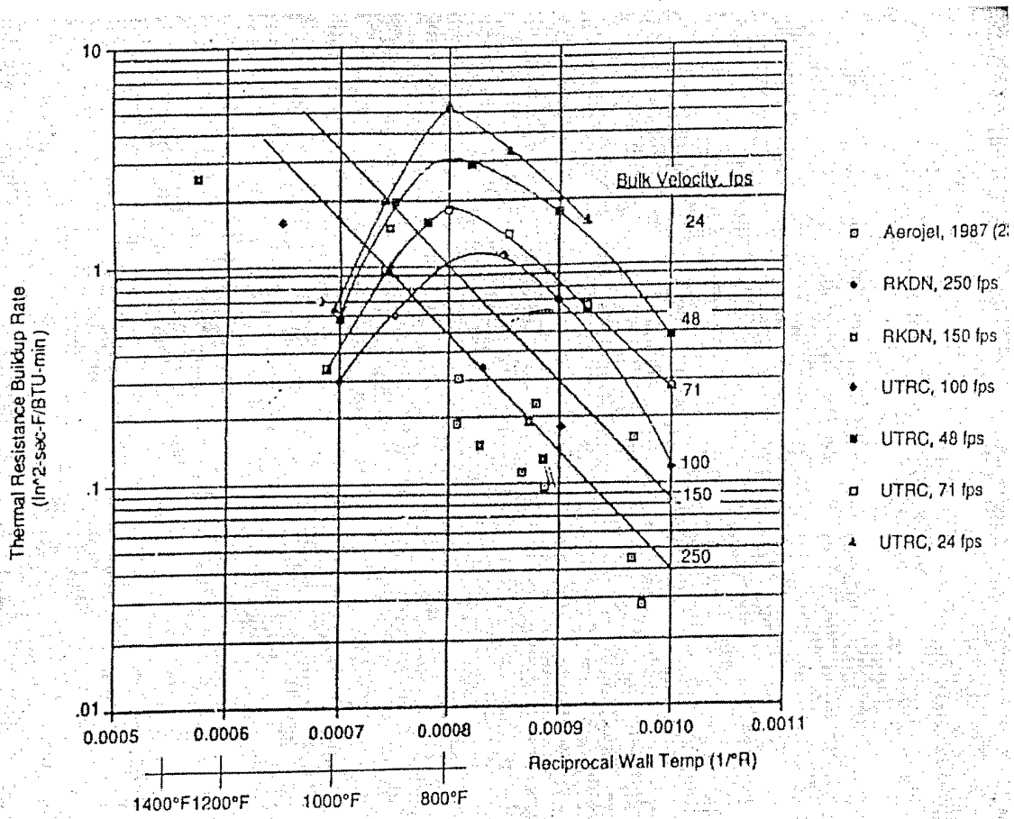
Figure 5 – Typical deposition (thermal resistance) behavior as a function of temperature [Rosenberg et al, 1970].
