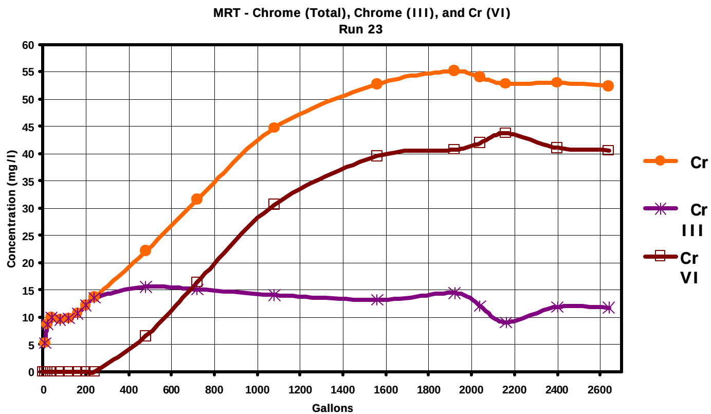
Figure 5-3. Plot of Cr (VI), Cr (III) & Total Cr plotted. (Total Cr T - Cr (VI) = Cr (III))
