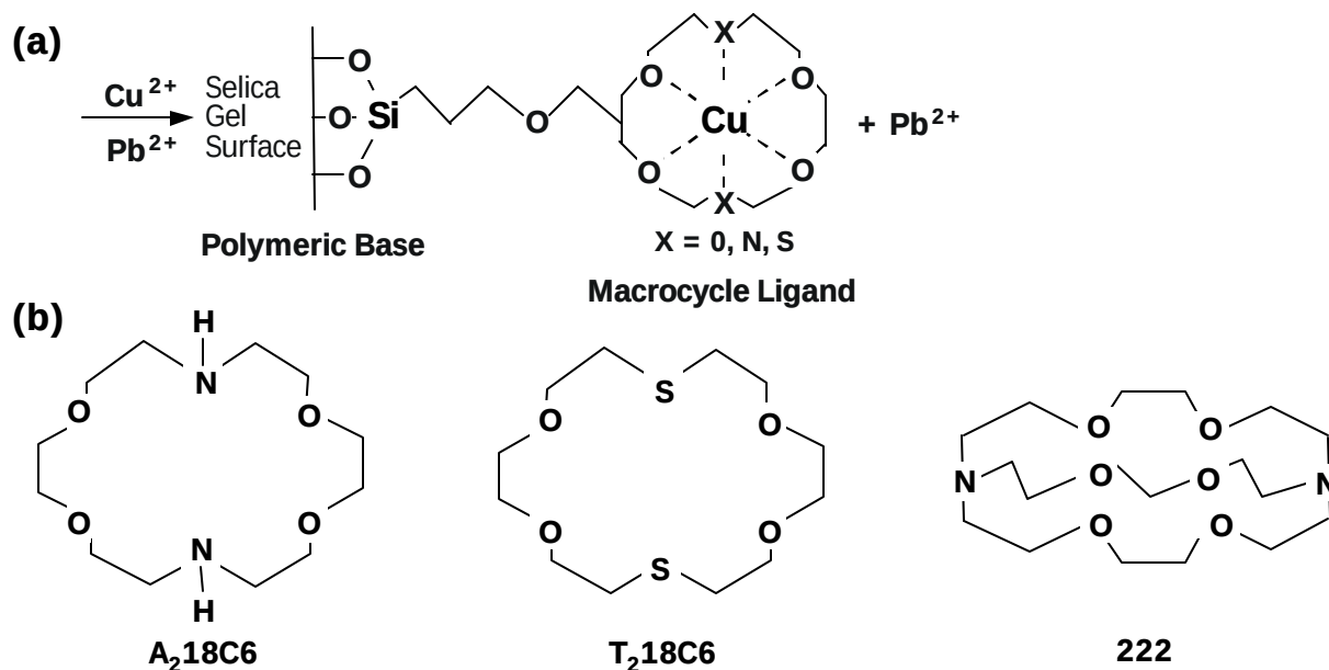
Figure 2-2. (a) Specific Ion Selectivity for Copper Ion Is Shown Over Lead Ion (b) IBC Patented Macrocyclic Ligands for Sequestering Metal Cations & Anions
