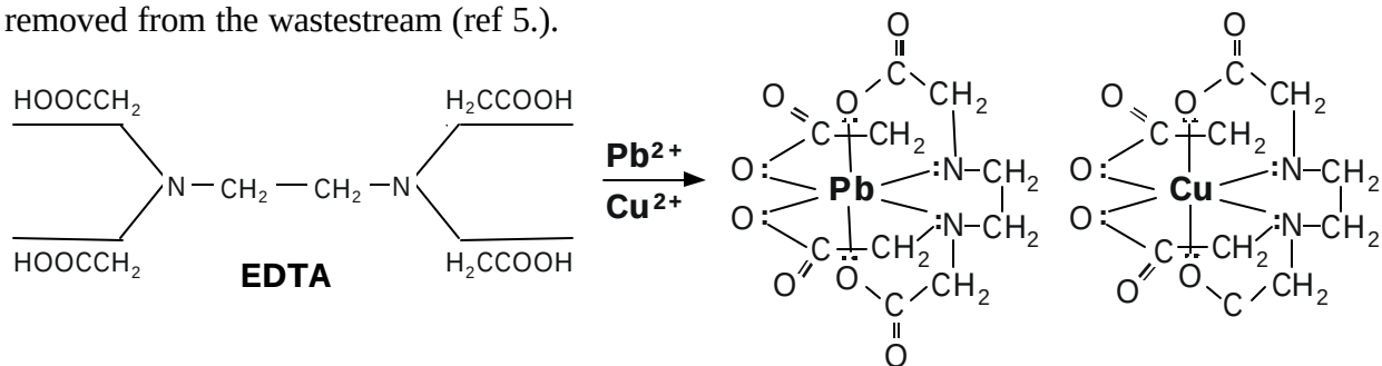
Figure 2-1. Non-Specific Metal Removal from Industrial Wastestreams with EDTA.
