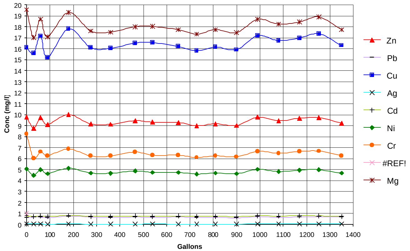
MRT - Data Run #4, Acid/Alkali, Port 2
