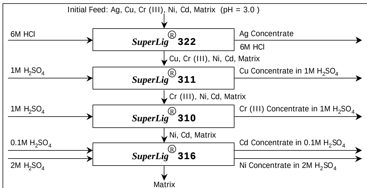
Figure 2-3. MRT Sequential, Selective Separation of Navy Chromium Wastewater
