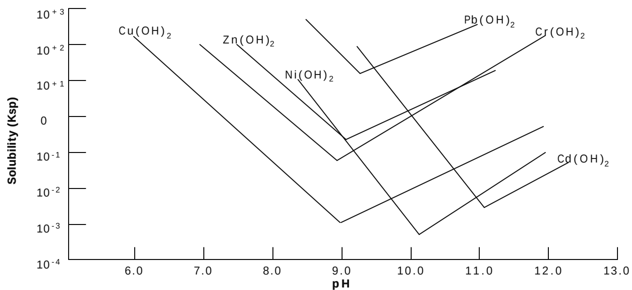
Figure 3-2 Solubility of Metal Hydroxides as a Function of pH (redrawn from ref. 8)
