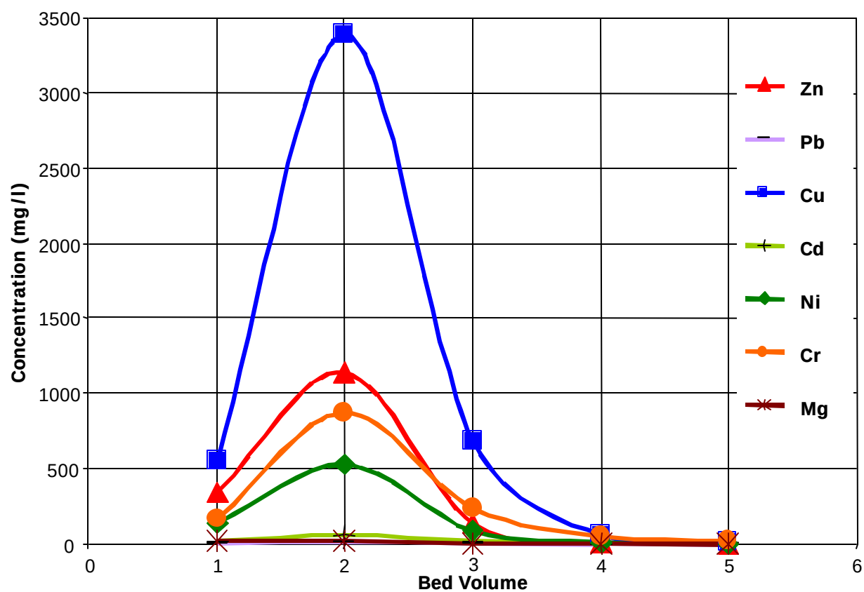
Figure 5-4. Acid/Alkali Regeneration Plot for Operation Test Run 4
