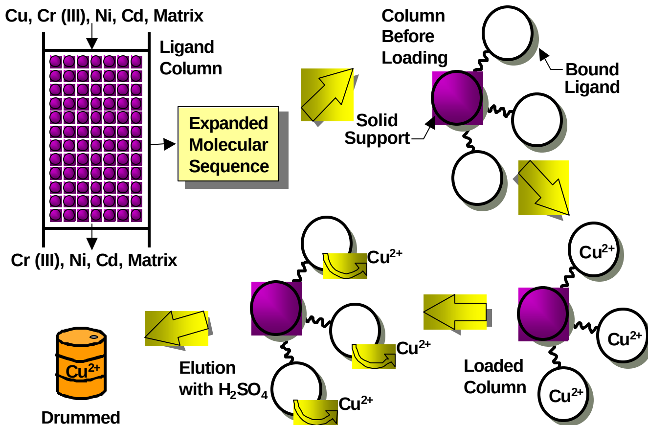
Figure 2-4. MRT Column \text{Cu}^{2+} Recovery Showing Final Product Concentrate for Recycle
