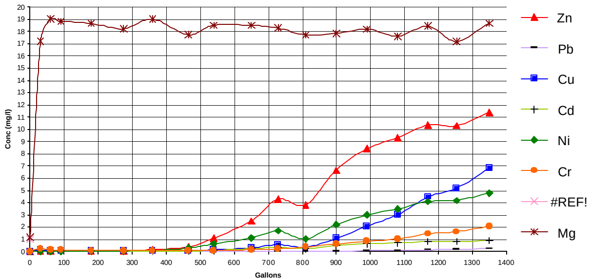
MRT - Data Run #4, Acid/Alkali, Port 3
