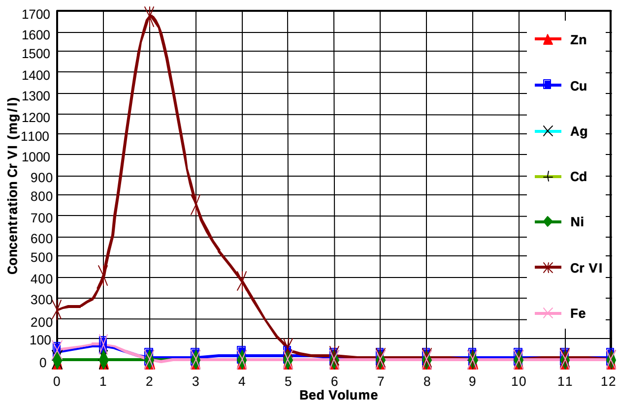
Figure 5-5. MRT 1M NaOH Regeneration for Chromium Recycle to Process, Run 23
