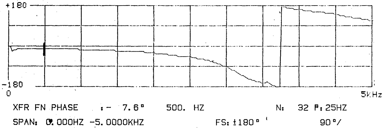
Figure 26. Transfer Function Amplitude and Phase for PCB SN1210 vs Columbia 902H
