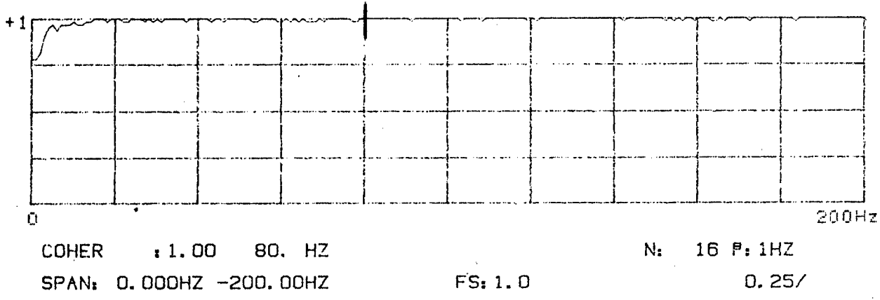
Figure 72. Transfer Function Amplitude and Coherence for PCB SN1237 vs Setra
