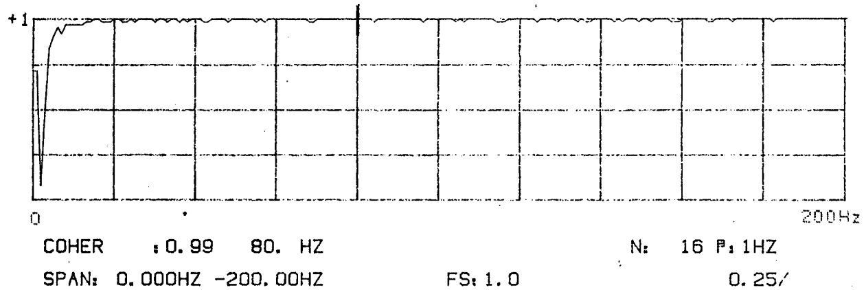
Figure 66. Transfer Function Amplitude and Coherence for PCB SN1212 vs Setra
