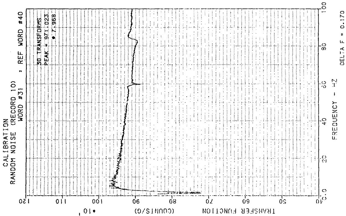
Figure 119. Transfer Function for word 31 (PCB SN 1212)
