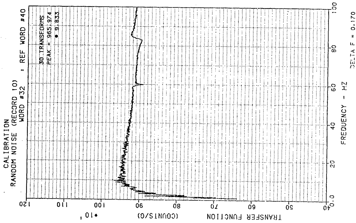
Figure 120. Transfer Function for word 32 (PCB SN 867)
