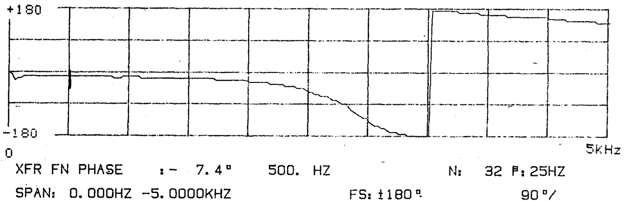
Figure 33. Transfer Function Amplitude and Phase for PCB SN1237 vs Columbia 902H
