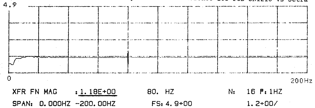
Figure 65. Transfer Function Amplitude and Coherence for PCB SN1210 vs Setra
