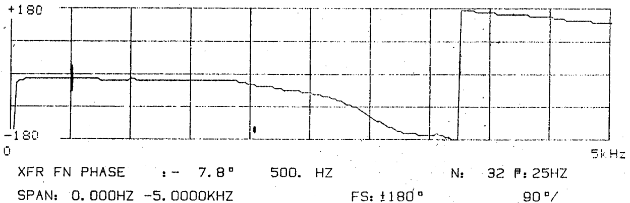
Figure 13. Transfer Function Amplitude and Phase for PCB SN889 vs Columbia 902H
