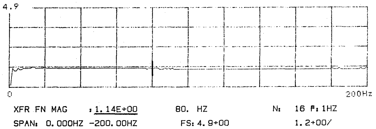
Figure 67. Transfer Function Amplitude and Coherence for PCB SN1213 vs Setra
