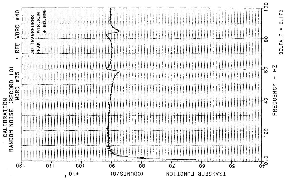
Figure 123. Transfer Function for word 35 (PCB SN 1208)
