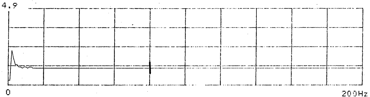
Figure 47. Transfer Function Amplitude and Coherence for PCB SN1089 vs Setra
