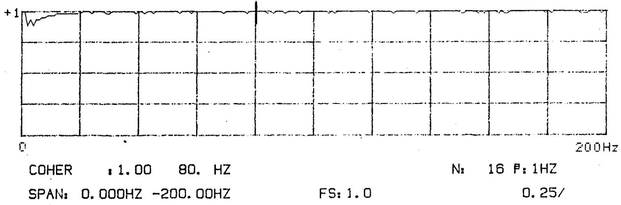
Figure 68. Transfer Function Amplitude and Coherence for PCB SN1215 vs Setra
