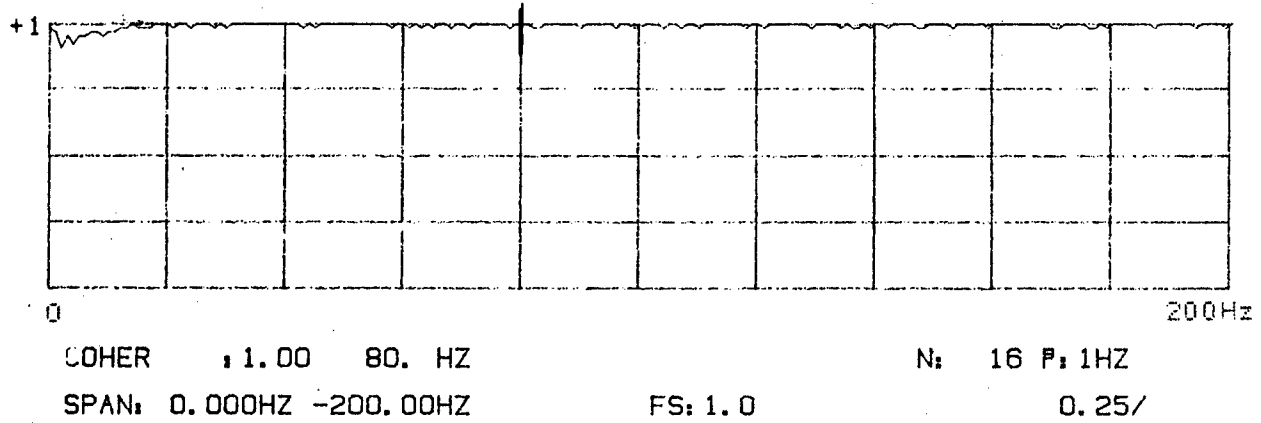
Figure 65. Transfer Function Amplitude and Coherence for PCB SN1210 vs Setra
