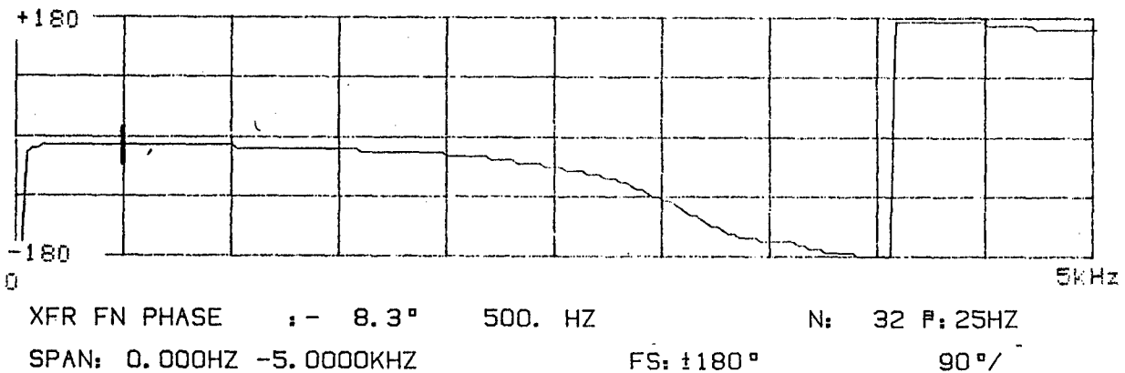
Figure 27. Transfer Function Amplitude and Phase for PCB SN1211 vs Columbia 902H
