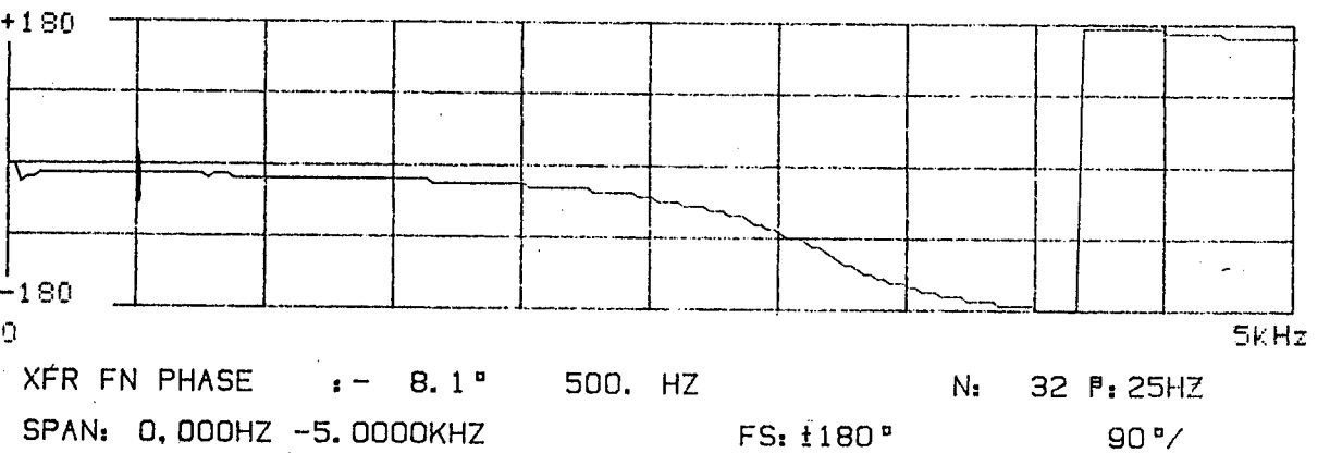
Figure 31. Transfer Function Amplitude and Phase for PCB SN1219 vs Columbia 902H
