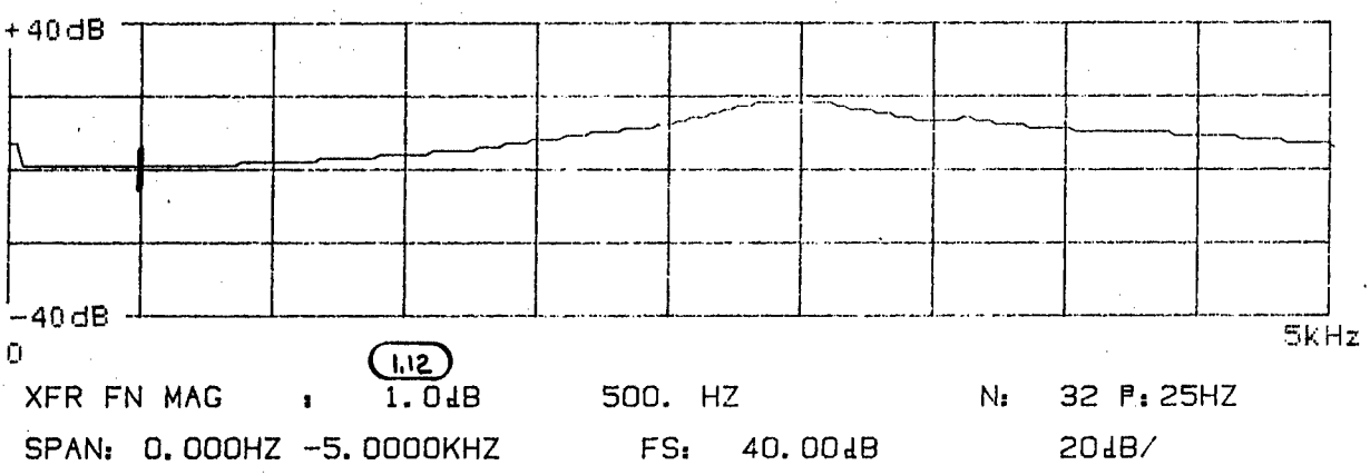
Figure 28. Transfer Function Amplitude and Phase for PCB SN1213 vs Columbia 902H
