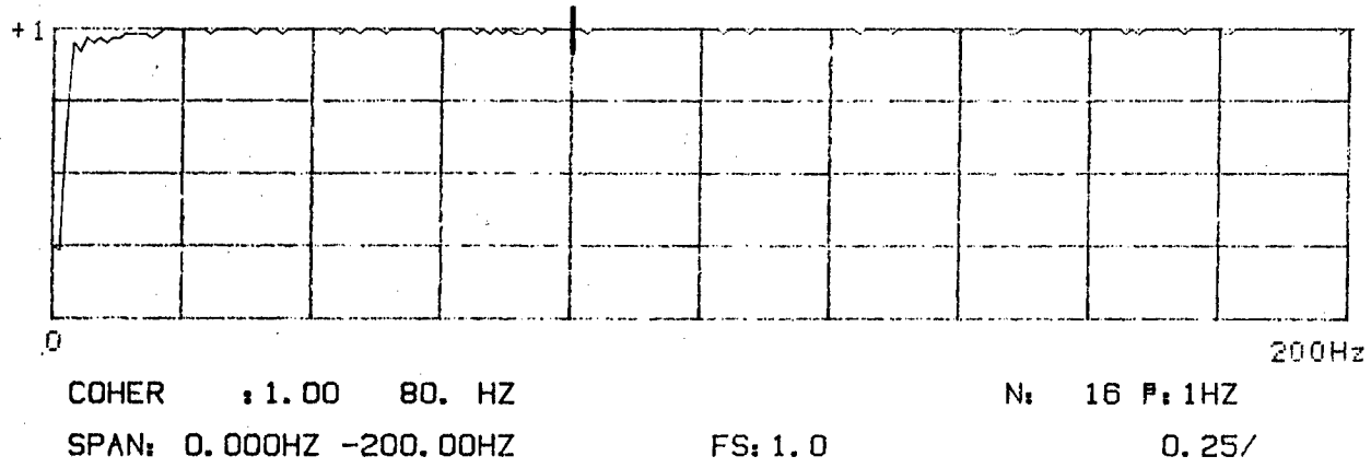
Figure 71. Transfer Function Amplitude and Coherence for PCB SN1234 vs Setra
