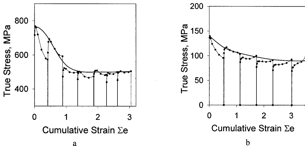
Fig. 9. Cumulative curve S-\Sigma\epsilon for 'abc' deformation at 550°C (a) and 800°C (b), and strain rate 10^{-3}s^{-1} of Ti-6Al-4V alloy, quenched in water from \beta -area.
