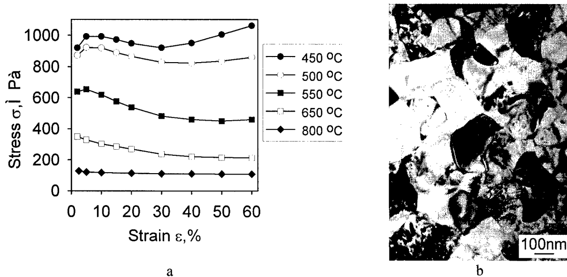
Fig. 2. Ti-6Al-4V alloy flow stress dependence on the strain at various temperatures and the strain rate of 10^{-3}\text{s}^{-1} (a); Ti-6Al-4V alloy microstructure after 70% deformation at 550°C and 10^{-3}\text{s}^{-1} (b).
