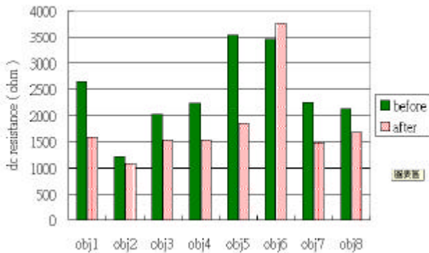
Fig. 3. The DC impedance before and after soaking. Solid column represent the impedance before soaking, and broken column represent the impedance after soaking.
