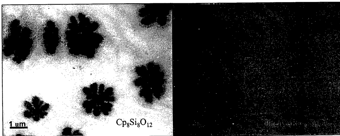
Figures 4 & 5: TEM of Cp_8Si_8O_{12} (Figure 4, left) and TEM of OctaphenethylPOSS (6) (Figure 5, right) in 2 million mol. wt. polystyrene.
