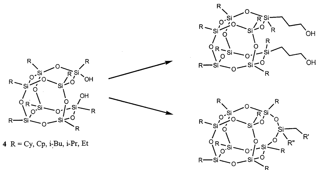
Scheme III
