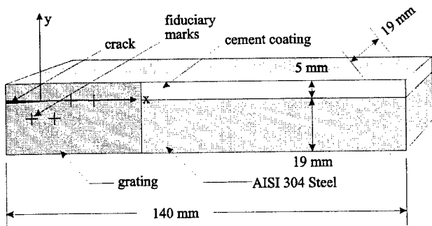
Figure 1 Geometry of the steel-thermocouple cement specimen
